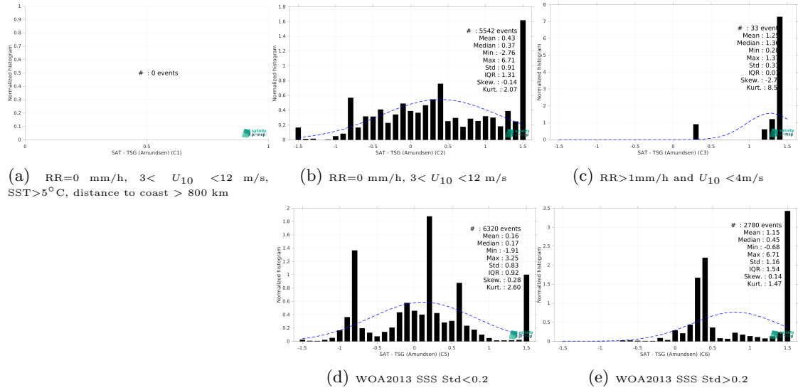
Figure 15: Normalized histogram of \Delta SSS (Aquarius SSS L4 OI v5 - Weekly (IPRC) - TSG (Amundsen)) for 5 different subdatasets corresponding to: RR=0 mm/h, 3 < U_{10} < 12 m/s, SST>5°C, distance to coast > 800 km (a), RR=0 mm/h, 3 < U_{10} < 12 m/s (b), RR>1mm/h and U_{10} < 4 m/s (c), WOA2013 SSS Std<0.2 (d), WOA2013 SSS Std>0.2 (e).
