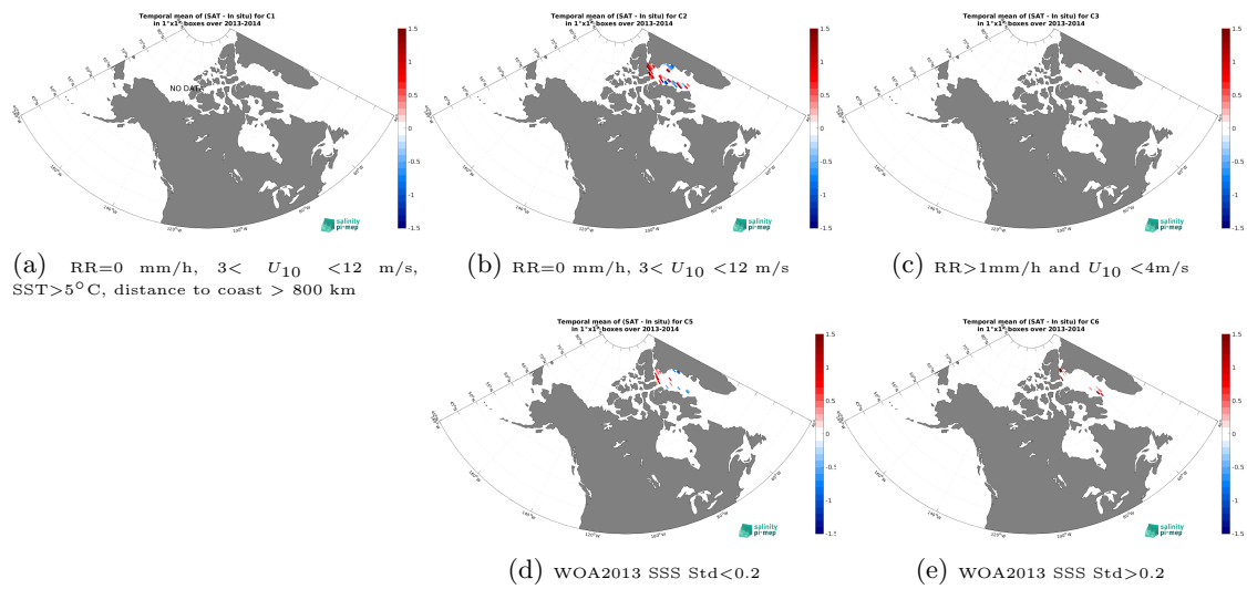
Figure 14: Temporal mean gridded over spatial boxes of size 1^\circ \times 1^\circ of \Delta SSS (Aquarius SSS L4 OI v5 - Weekly (IPRC) - TSG (Amundsen)) for 5 different subdatasets corresponding to:RR=0 mm/h, 3 < U_{10} < 12 m/s, SST > 5°C, distance to coast > 800 km (a), RR=0 mm/h, 3 < U_{10} < 12 m/s (b), RR > 1mm/h and U_{10} < 4 m/s (c), WOA2013 SSS Std < 0.2 (d), WOA2013 SSS Std > 0.2 (e).
