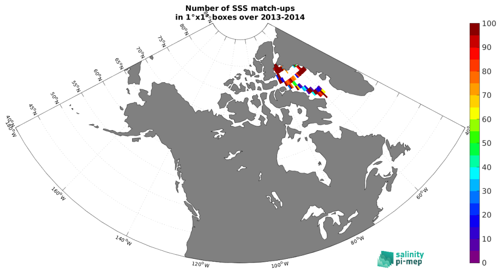
Figure 5: Number of SSS match-ups between TSG (Amundsen) SSS and the Aquarius SSS L4 OI v5 - Weekly (IPRC) SSS product for the Arctic Ocean Pi-MEP region over 1^\circ \times 1^\circ boxes and for the full satellite product period.
