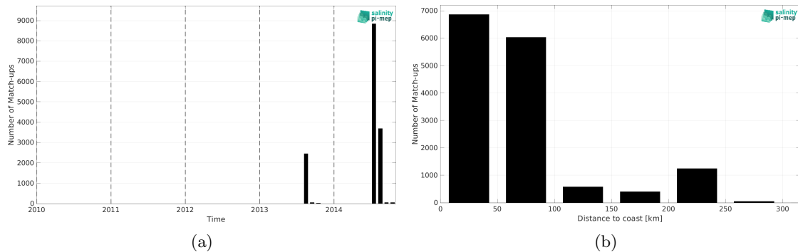
Figure 2: Number of match-ups between TSG (Amundsen) and Aquarius SSS L4 OI v5 - Weekly (IPRC) SSS as a function of time (a) and as function of the distance to coast (b) over the Arctic Ocean Pi-MEP region and for the full satellite product period.
