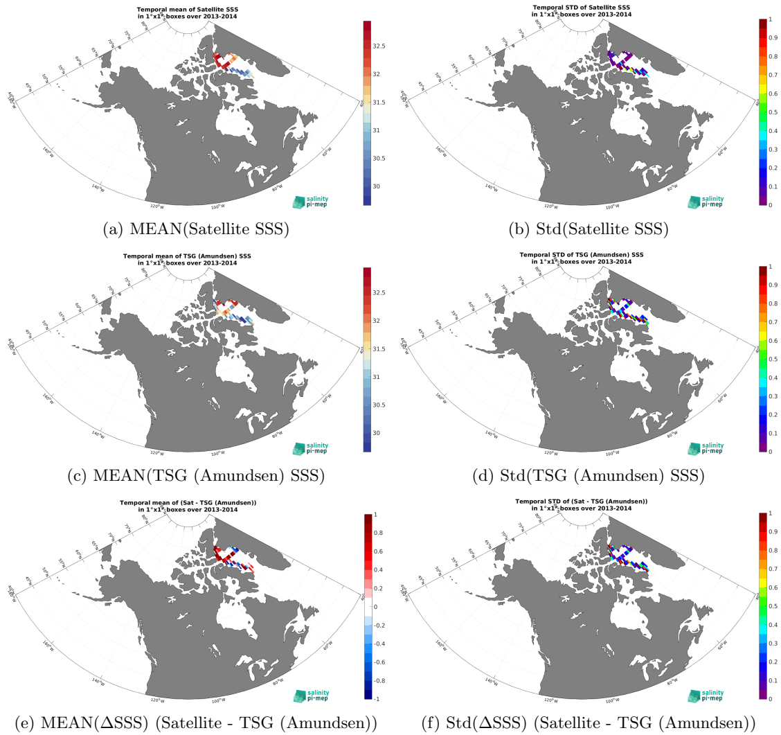
Figure 7: Temporal mean (left) and Std (right) of SSS from Aquarius SSS L4 OI v5 - Weekly (IPRC) (top), TSG (Amundsen) (middle), and of \Delta SSS (Satellite - TSG (Amundsen)). Only match-up pairs are used to generate these maps.
