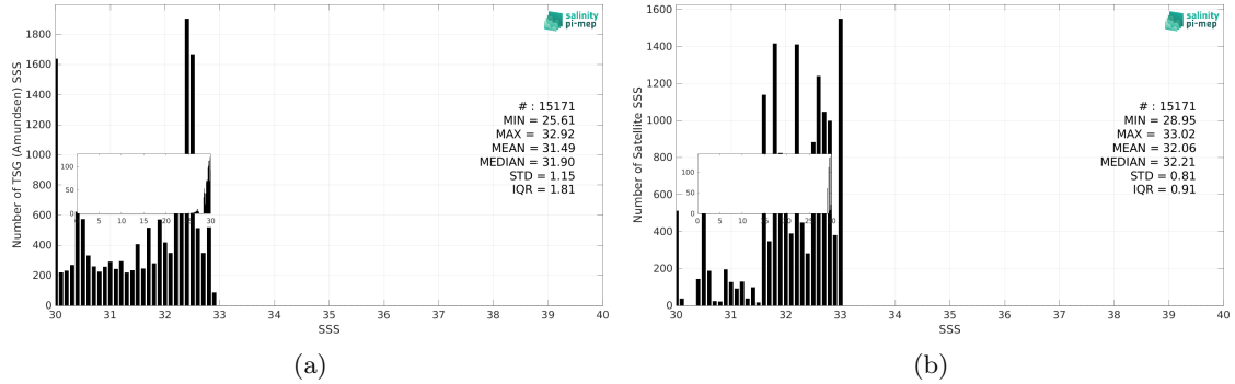
Figure 3: Histograms of SSS from TSG (Amundsen) (a) and Aquarius SSS L4 OI v5 - Weekly (IPRC) (b) considering all match-up pairs per bins of 0.1 over the Arctic Ocean Pi-MEP region and for the full satellite product period.
