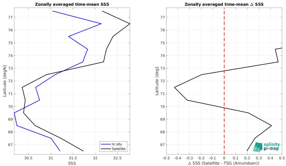
Figure 9: Left panel: Zonal mean SSS from Aquarius SSS L4 OI v5 - Weekly (IPRC) satellite product (black) and from TSG (Amundsen) (blue). Right panel: Zonal mean of \Delta SSS (Satellite - TSG (Amundsen)) for all the collected Pi-MEP match-up pairs estimated over the full satellite product period.
