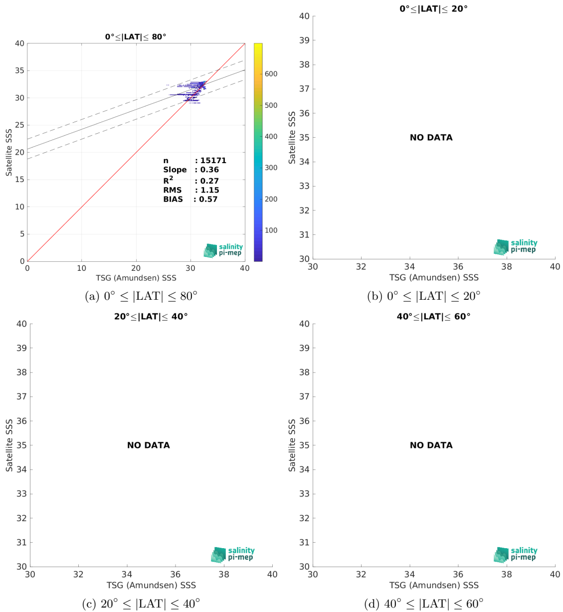
Figure 10: Contour maps of the concentration of Aquarius SSS L4 OI v5 - Weekly (IPRC) SSS (y-axis) versus TSG (Amundsen) SSS (x-axis) at match-up pairs for different latitude bands. For each plot, the red line shows x=y . The black thin and dashed lines indicate a linear fit through the data cloud and the \pm 95\% confidence levels, respectively. The number match-up pairs n , the slope and R^2 coefficient of the linear fit, the root mean square (RMS) and the mean bias between satellite and in situ data are indicated for each latitude band in each plots.
