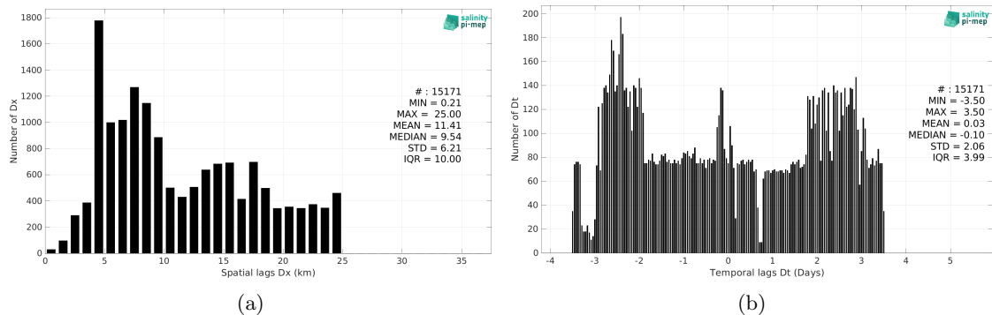
Figure 6: Histograms of the spatial (a) and temporal (b) lags between the location/time of the TSG (Amundsen) measurement and the date of the corresponding Aquarius SSS L4 OI v5 - Weekly (IPRC) SSS pixel.
