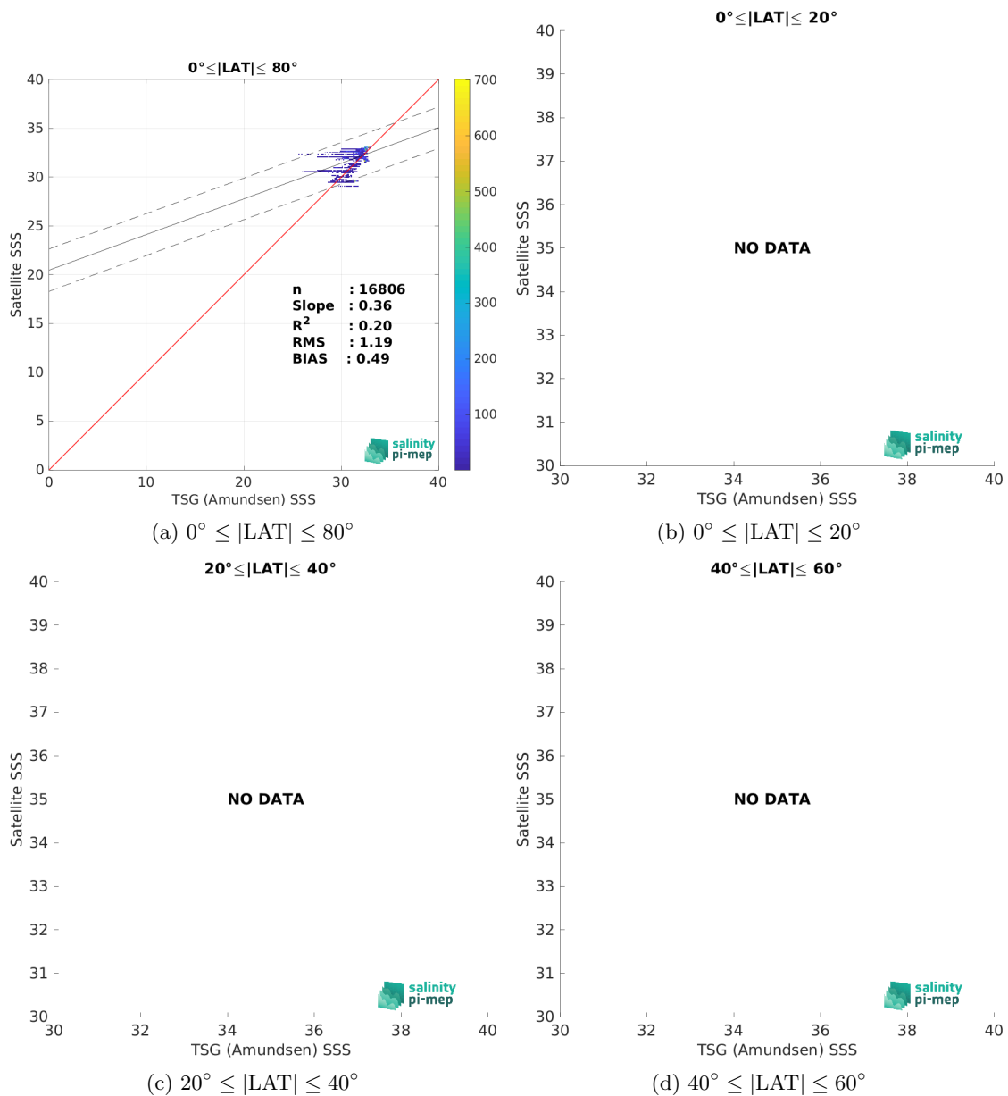
Figure 9: Contour maps of the concentration of Aquarius SSS L4 OI v5 - Weekly (IPRC) SSS (y-axis) versus TSG (Amundsen) SSS (x-axis) at match-up pairs for different latitude bands. For each plot, the red line shows x=y . The black thin and dashed lines indicate a linear fit through the data cloud and the \pm 95\% confidence levels, respectively. The number match-up pairs n , the slope and R^2 coefficient of the linear fit, the root mean square (RMS) and the mean bias between satellite and in situ data are indicated for each latitude band in each plots.
