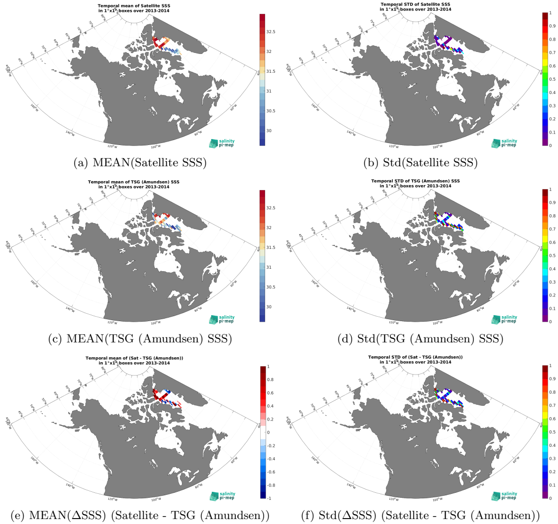
Figure 6: Temporal mean (left) and Std (right) of SSS from Aquarius SSS L4 OI v5 - Weekly (IPRC) (top), TSG (Amundsen) (middle), and of \Delta SSS (Satellite - TSG (Amundsen)). Only match-up pairs are used to generate these maps.
