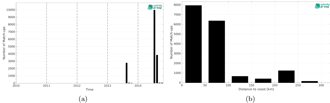
Figure 1: Number of match-ups between TSG (Amundsen) and Aquarius SSS L4 OI v5 - Weekly (IPRC) SSS as a function of time (a) and as function of the distance to coast (b) over the Arctic Ocean Pi-MEP region and for the full satellite product period.
