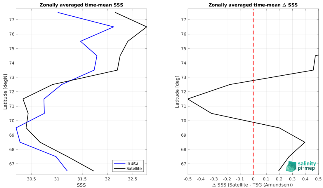
Figure 8: Left panel: Zonal mean SSS from Aquarius SSS L4 OI v5 - Weekly (IPRC) satellite product (black) and from TSG (Amundsen) (blue). Right panel: Zonal mean of \Delta SSS (Satellite - TSG (Amundsen)) for all the collected Pi-MEP match-up pairs estimated over the full satellite product period.
