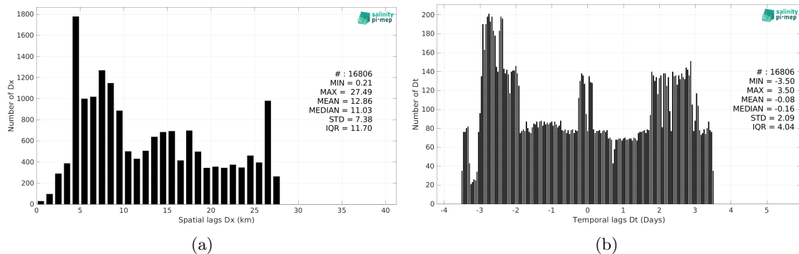
Figure 5: Histograms of the spatial (a) and temporal (b) lags between the location/time of the TSG (Amundsen) measurement and the date of the corresponding Aquarius SSS L4 OI v5 - Weekly (IPRC) SSS pixel.
