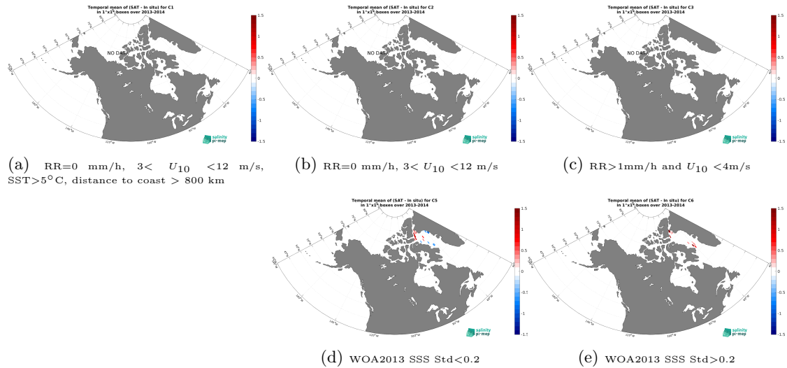
Figure 12: Temporal mean gridded over spatial boxes of size 1^{\circ}\times 1^{\circ} of \Delta\text{SSS} (Aquarius SSS L4 OI v5 - Weekly (IPRC) - TSG (Amundsen)) for 5 different subdatasets corresponding to:RR=0 mm/h, 3 < U_{10} < 12 m/s, SST >5^{\circ}\text{C} , distance to coast > 800 km (a), RR=0 mm/h, 3 < U_{10} < 12 m/s (b), RR >1 mm/h and U_{10} < 4 m/s (c), WOA2013 SSS Std <0.2 (d), WOA2013 SSS Std >0.2 (e).
