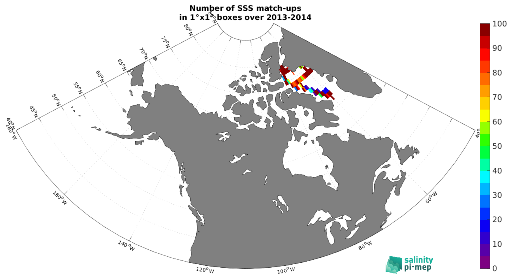
Figure 4: Number of SSS match-ups between TSG (Amundsen) SSS and the Aquarius SSS L4 OI v5 - Weekly (IPRC) SSS product for the Arctic Ocean Pi-MEP region over 1^\circ \times 1^\circ boxes and for the full satellite product period.
