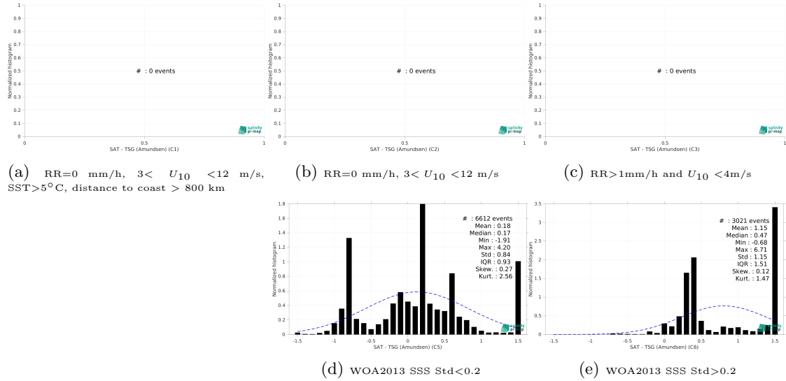
Figure 13: Normalized histogram of \Delta SSS (Aquarius SSS L4 OI v5 - Weekly (IPRC) - TSG (Amundsen)) for 5 different subdatasets corresponding to: RR=0 mm/h, 3 < U_{10} < 12 m/s, SST >5^{\circ} C, distance to coast > 800 km (a), RR=0 mm/h, 3 < U_{10} < 12 m/s (b), RR >1 mm/h and U_{10} < 4 m/s (c), WOA2013 SSS Std <0.2 (d), WOA2013 SSS Std >0.2 (e).
