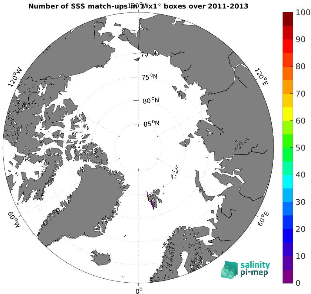
Figure 4: Number of SSS match-ups between Marine mammals SSS and the Aquarius SSS L4 OI v5 - Weekly (IPRC) SSS product for the Arctic Ocean Pi-MEP region over 1^\circ \times 1^\circ boxes and for the full satellite product period.
