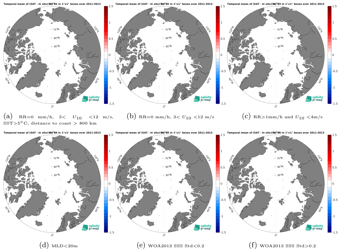
Figure 12: Temporal mean gridded over spatial boxes of size 1^{\circ}\times 1^{\circ} of \Delta\text{SSS} (Aquarius SSS L4 OI v5 - Weekly (IPRC) - Marine mammals) for 6 different subdatasets corresponding to:RR=0 mm/h, 3 < U_{10} < 12 m/s, SST >5^{\circ}\text{C} , distance to coast > 800 km (a), RR=0 mm/h, 3 < U_{10} < 12 m/s (b), RR >1 mm/h and U_{10} < 4 m/s (c),MLD <20 m (d),WOA2013 SSS Std <0.2 (e),WOA2013 SSS Std >0.2 (f).
