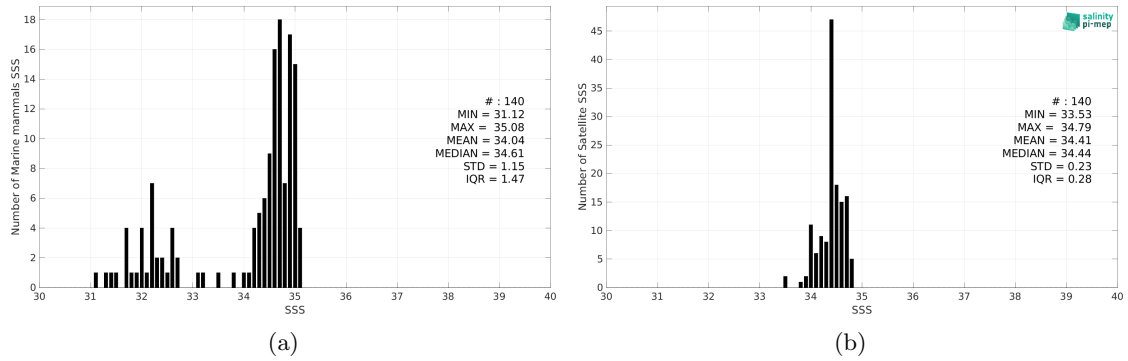
Figure 2: Histograms of SSS from Marine mammals (a) and Aquarius SSS L4 OI v5 - Weekly (IPRC) (b) considering all match-up pairs per bins of 0.1 over the Arctic Ocean Pi-MEP region and for the full satellite product period.
