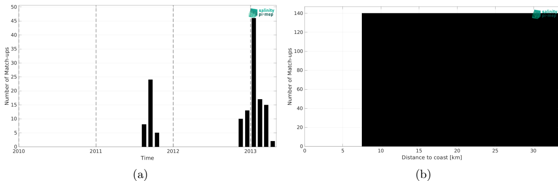
Figure 1: Number of match-ups between Marine mammals and Aquarius SSS L4 OI v5 - Weekly (IPRC) SSS as a function of time (a) and as function of the distance to coast (b) over the Arctic Ocean Pi-MEP region and for the full satellite product period.
