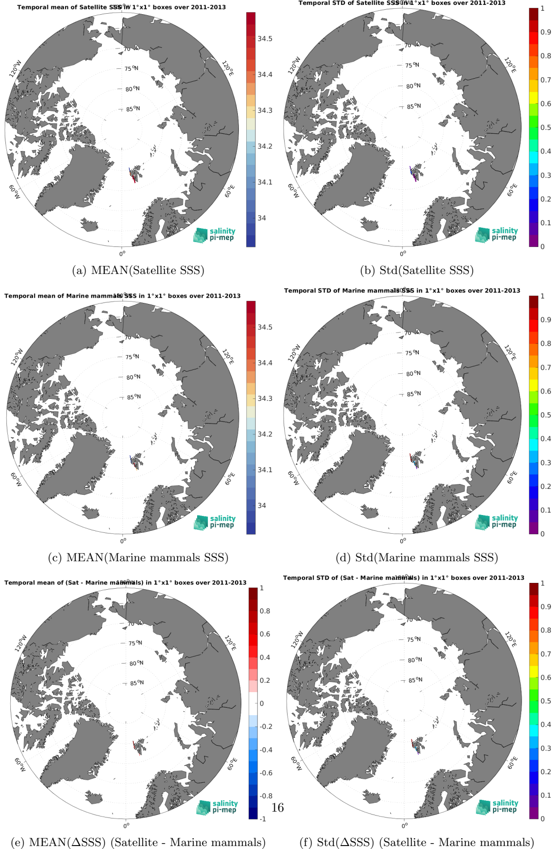
Figure 6: Temporal mean (left) and Std (right) of SSS from Aquarius SSS L4 OI v5 - Weekly (IPRC) (top), Marine mammals (middle), and of \Delta SSS (Satellite - Marine mammals). Only match-up pairs are used to generate these maps.
