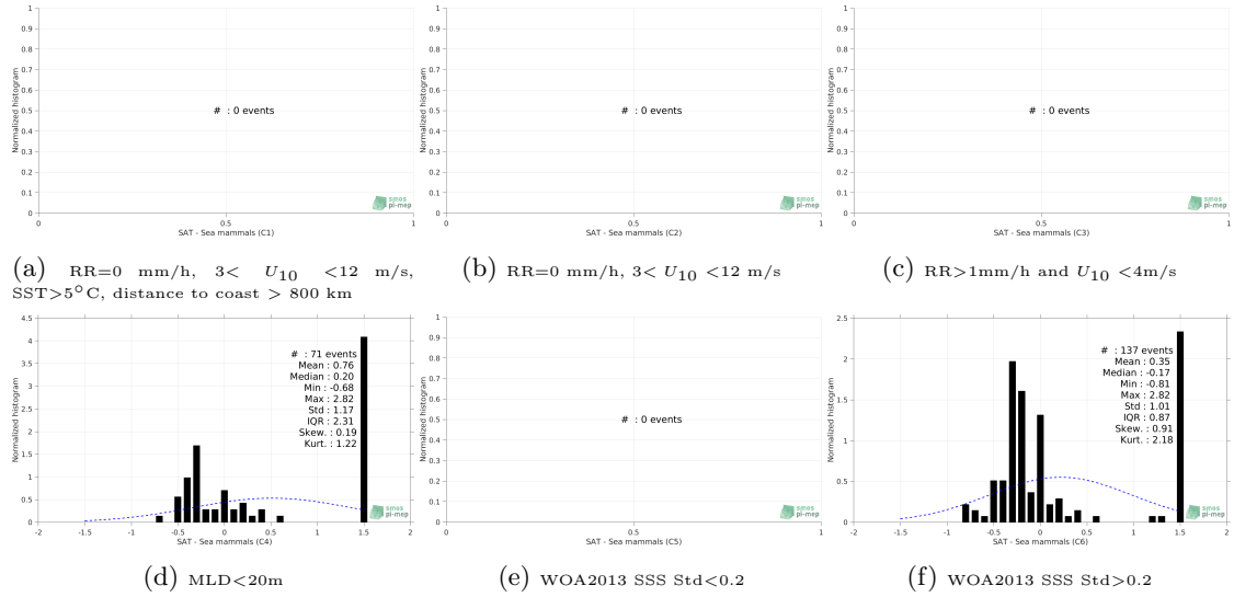
Figure 13: Normalized histogram of \Delta\text{SSS} (Aquarius-L4-IPRC-V5-WEEKLY - Sea mammals) for 6 different subdatasets corresponding to: RR=0 mm/h, 3 < U_{10} < 12 m/s, SST >5^{\circ}\text{C} , distance to coast > 800 km (a), RR=0 mm/h, 3 < U_{10} < 12 m/s (b), RR >1 mm/h and U_{10} < 4 m/s (c), MLD <20 m (d), WOA2013 SSS Std <0.2 (e), WOA2013 SSS Std >0.2 (f).
