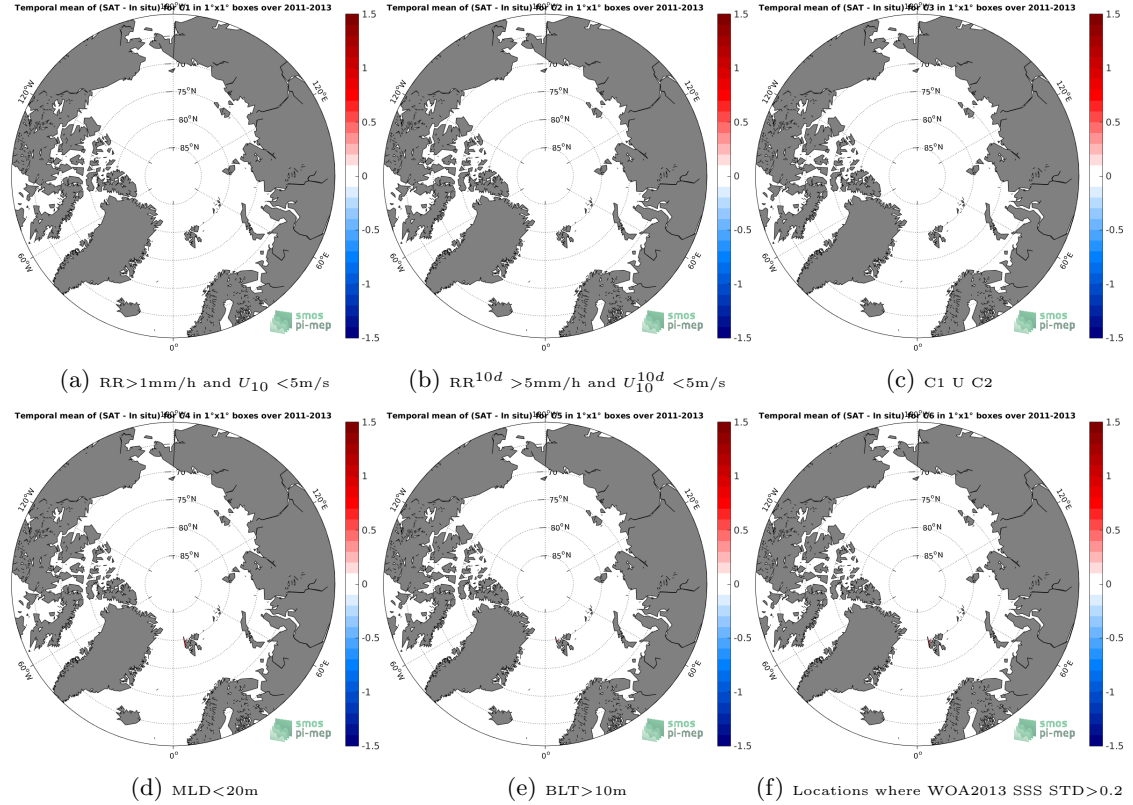
Figure 12: Temporal mean gridded over spatial boxes of size 1^\circ \times 1^\circ of \Delta\text{SSS} (Aquarius-L4-IPRC-V5-WEEKLY - Sea mammals) for 6 different subdatasets corresponding to: \text{RR} > 1\text{mm/h} and U_{10} < 5\text{m/s} (a), \text{RR}^{10d} > 5\text{mm/h} and U_{10}^{10d} < 5\text{m/s} (b), C1 U C2 (c), \text{MLD} < 20\text{m} (d), \text{BLT} > 10\text{m} (e), Locations where WOA2013 SSS STD > 0.2 (f).
