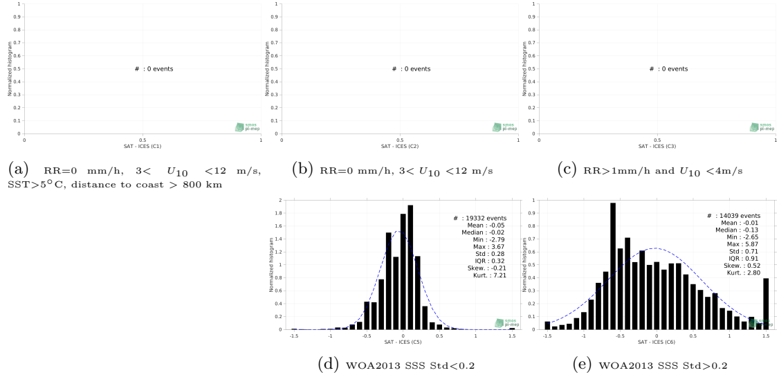
Figure 13: Normalized histogram of \Delta SSS (Aquarius SSS L4 OI v5 - Weekly (IPRC) - ICES) for 5 different subdatasets corresponding to: RR=0 mm/h, 3 < U_{10} < 12 m/s, SST > 5°C, distance to coast > 800 km (a), RR=0 mm/h, 3 < U_{10} < 12 m/s (b), RR > 1mm/h and U_{10} < 4 m/s (c), WOA2013 SSS Std < 0.2 (d), WOA2013 SSS Std > 0.2 (e).
