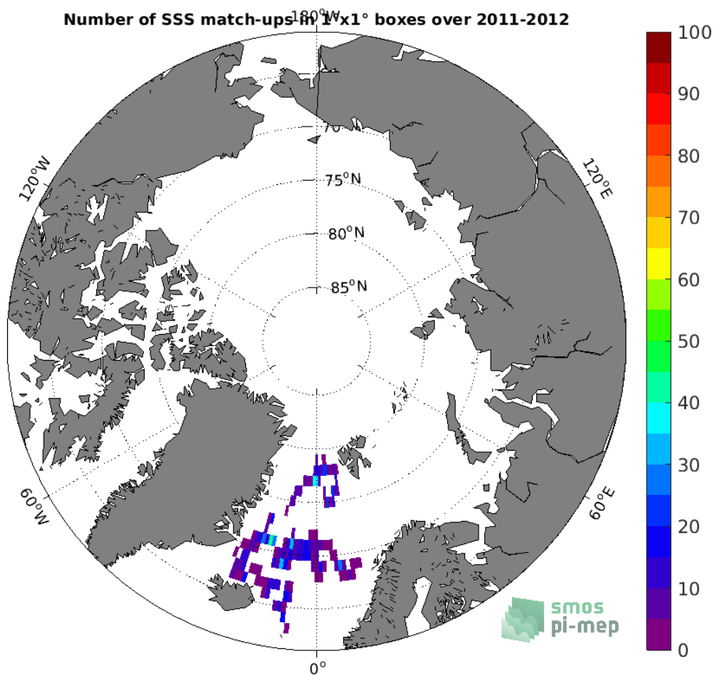
Figure 3: Number of SSS match-ups between Surface drifters SSS and the Aquarius SSS L4 OI v5 - Weekly (IPRC) SSS product for the Arctic Ocean Pi-MEP region over 1^\circ \times 1^\circ boxes and for the full satellite product period.
