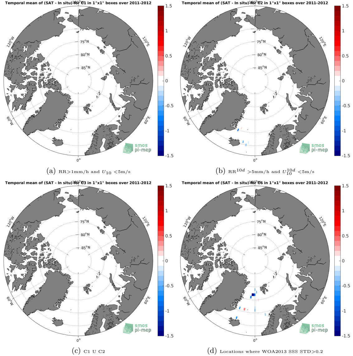
Figure 11: Temporal mean gridded over spatial boxes of size 1^\circ \times 1^\circ of \Delta SSS (Aquarius-L4-IPRC-V5-WEEKLY - Surface drifters) for 4 different subdatasets corresponding to: RR > 1\text{mm/h} and U_{10} < 5\text{m/s} (a), RR^{10d} > 5\text{mm/h} and U_{10}^{10d} < 5\text{m/s} (b), C1 U C2 (c), Locations where WOA2013 SSS STD > 0.2 (d).
