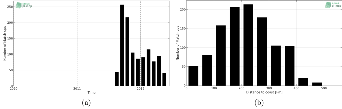
Figure 1: Number of match-ups between Surface drifters and Aquarius-L4-IPRC-V5-WEEKLY SSS as a function of time (a) and as function of the distance to coast (b) over the Arctic Ocean Pi-MEP region and for the full satellite product period.
