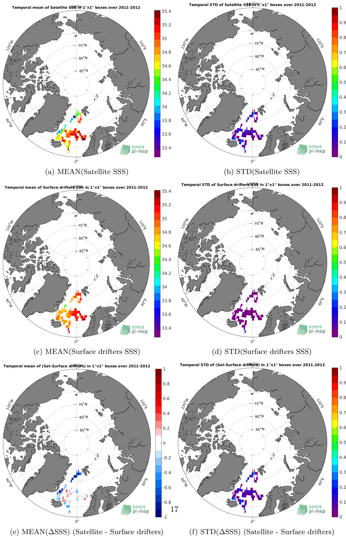
Figure 5: Temporal mean (left) and STD (right) of SSS from Aquarius-L4-IPRC-V5-WEEKLY (top), Surface drifters (middle), and of \Delta SSS (Satellite - Surface drifters). Only match-up pairs are used to generate these maps.
