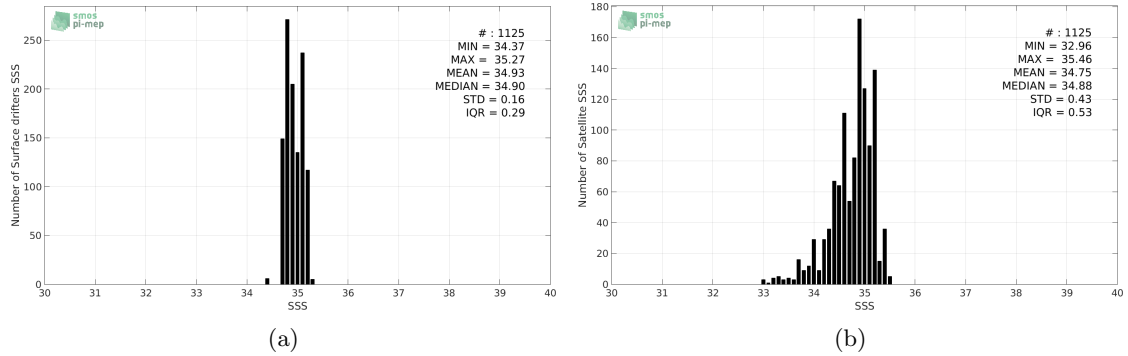
Figure 2: Histograms of SSS from Surface drifters (a) and Aquarius-L4-IPRC-V5-WEEKLY (b) considering all match-up pairs per bins of 0.1 over the Arctic Ocean Pi-MEP region and for the full satellite product period.
