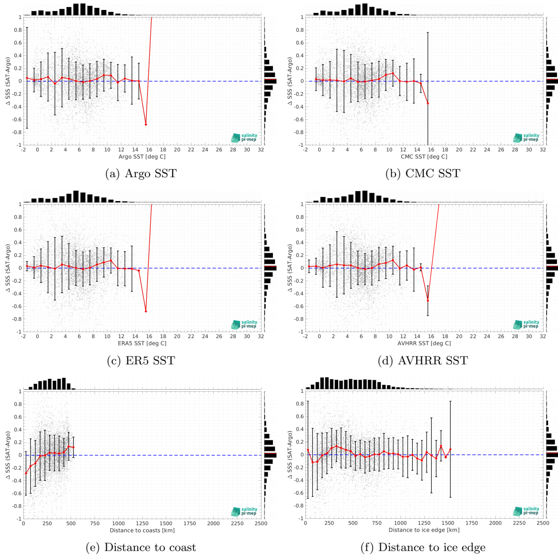
Figure 13: \Delta \text{SSS} (Satellite - Argos) sorted as function of Argos SST values (a), CMC SST (b), ERA5 SST (c), AVHRR SST (d), distance to coast (e) and distance to ice edge (f). In all plots the median and Std of \Delta \text{SSS} for each bin is indicated by the red curves and black vertical thick bars ( \pm 1 \text{ Std} ). Links to similar figures sorted as function of Sea ice fraction and in situ measurement depth .
