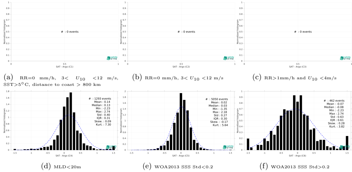
Figure 13: Normalized histogram of \Delta\text{SSS} (Aquarius SSS L4 OI v5 - Weekly (IPRC) - Argo) for 6 different subdatasets corresponding to: RR=0 mm/h, 3 < U_{10} < 12 m/s, SST > 5^{\circ}\text{C} , distance to coast > 800 km (a), RR=0 mm/h, 3 < U_{10} < 12 m/s (b), RR > 1\text{mm/h} and U_{10} < 4\text{m/s} (c), MLD < 20\text{m} (d), WOA2013 SSS Std < 0.2 (e), WOA2013 SSS Std > 0.2 (f).
