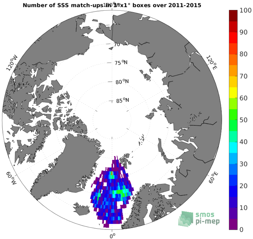
Figure 4: Number of SSS match-ups between Argo SSS and the Aquarius SSS L4 OI v5 - Weekly (IPRC) SSS product for the Arctic Ocean Pi-MEP region over 1^\circ \times 1^\circ boxes and for the full satellite product period.
