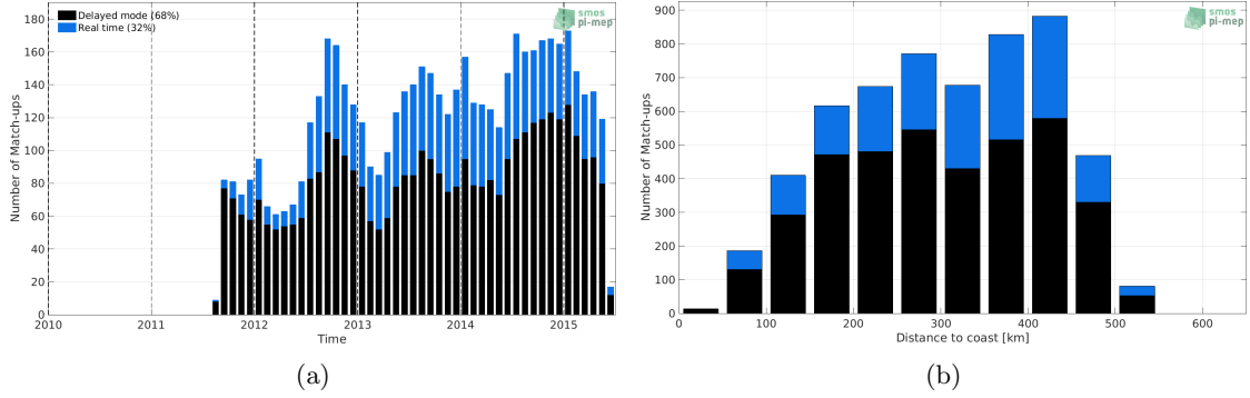
Figure 1: Number of match-ups between Argo and Aquarius SSS L4 OI v5 - Weekly (IPRC) SSS as a function of time (a) and as function of the distance to coast (b) over the Arctic Ocean Pi-MEP region and for the full satellite product period.
