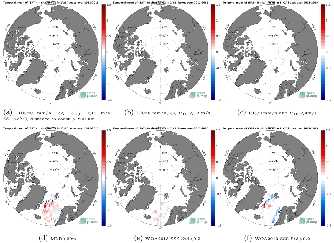
Figure 12: Temporal mean gridded over spatial boxes of size 1^{\circ}\times 1^{\circ} of \Delta\text{SSS} (Aquarius SSS L4 OI v5 - Weekly (IPRC) - Argo) for 6 different subdatasets corresponding to:RR=0 mm/h, 3 < U_{10} < 12 m/s, SST >5^{\circ}\text{C} , distance to coast > 800 km (a), RR=0 mm/h, 3 < U_{10} < 12 m/s (b), RR >1 mm/h and U_{10} < 4 m/s (c),MLD <20 m (d),WOA2013 SSS Std <0.2 (e),WOA2013 SSS Std >0.2 (f).
