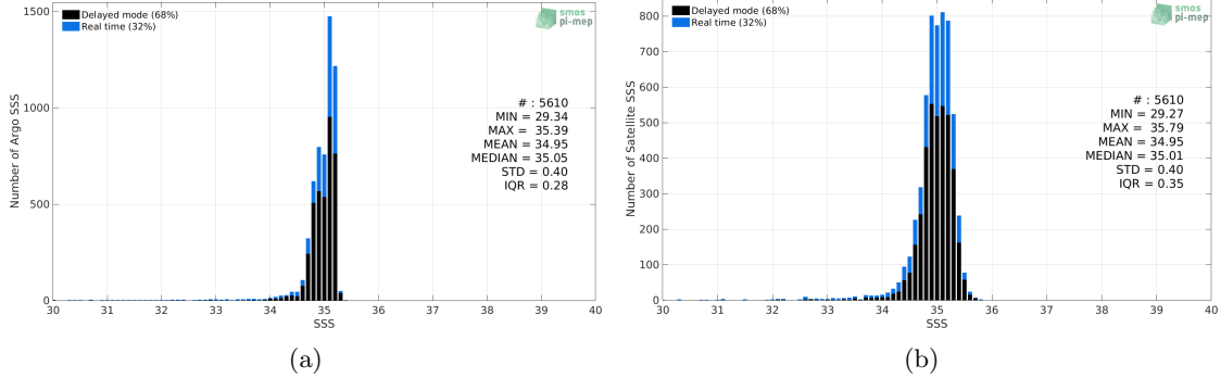
Figure 2: Histograms of SSS from Argo (a) and Aquarius SSS L4 OI v5 - Weekly (IPRC) (b) considering all match-up pairs per bins of 0.1 over the Arctic Ocean Pi-MEP region and for the full satellite product period.
