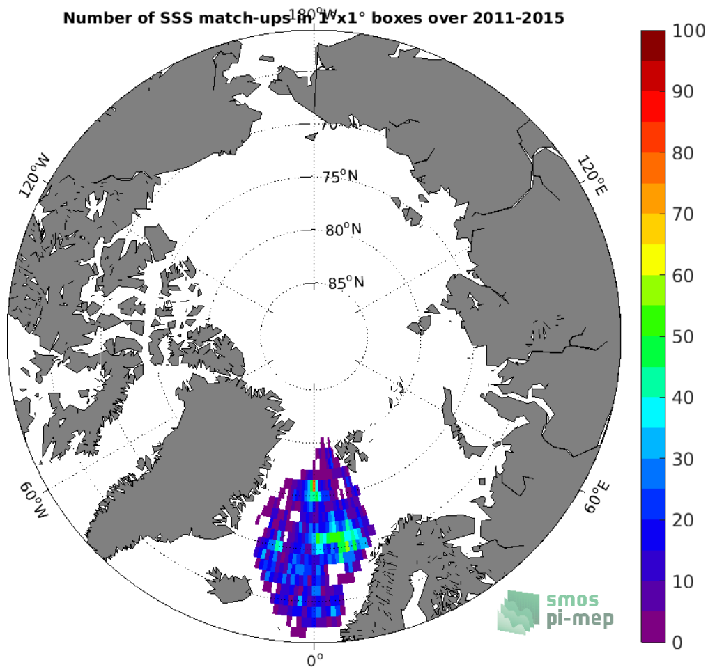
Figure 4: Number of SSS match-ups between Argo SSS and the Aquarius SSS L4 OI v5 - Weekly (IPRC) SSS product for the Arctic Ocean Pi-MEP region over 1°x1° boxes and for the full satellite product period.
