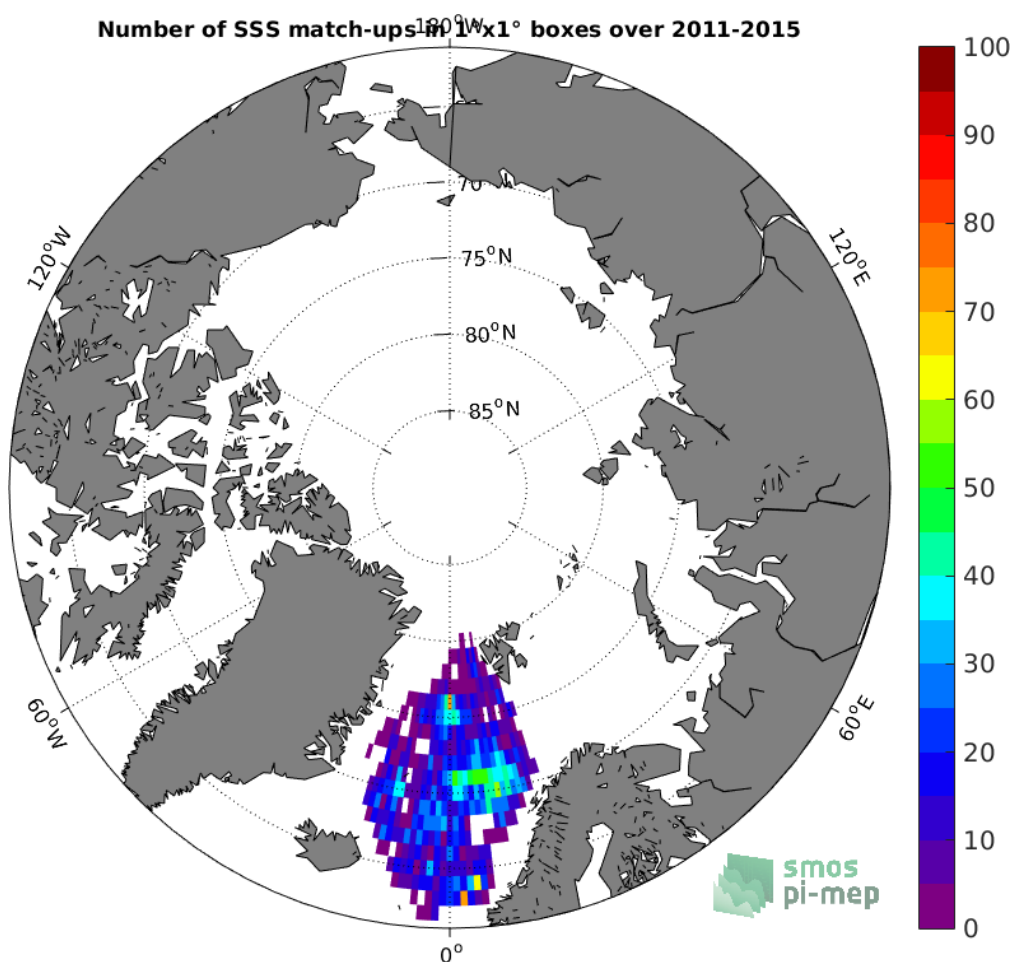
Figure 4: Number of SSS match-ups between Argo SSS and the Aquarius-L4-IPRC-V5-WEEKLY SSS product for the Arctic Ocean Pi-MEP region over 1°x1° boxes and for the full satellite product period.
