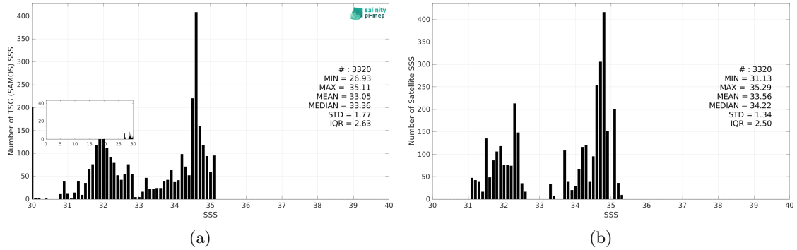
Figure 3: Histograms of SSS from TSG (SAMOS) (a) and Aquarius SSS L4 OI v5 - Monthly (IPRC) (b) considering all match-up pairs per bins of 0.1 over the Arctic Ocean Pi-MEP region and for the full satellite product period.
