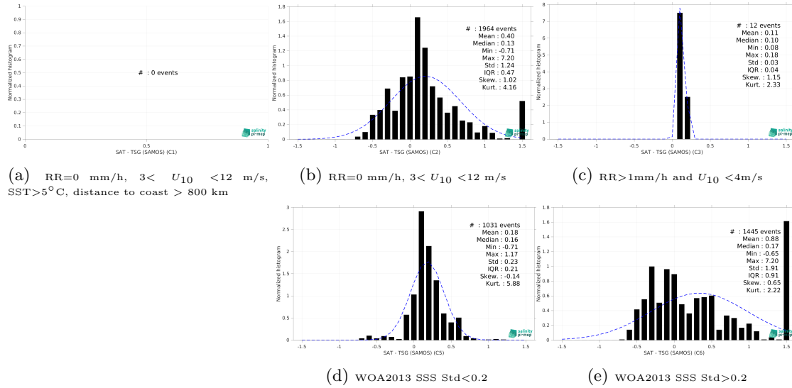
Figure 15: Normalized histogram of \Delta SSS (Aquarius SSS L4 OI v5 - Monthly (IPRC) - TSG (SAMOS)) for 5 different subdatasets corresponding to: RR=0 mm/h, 3 < U_{10} < 12 m/s, SST >5^{\circ} C, distance to coast > 800 km (a), RR=0 mm/h, 3 < U_{10} < 12 m/s (b), RR >1 mm/h and U_{10} < 4 m/s (c), WOA2013 SSS Std <0.2 (d), WOA2013 SSS Std >0.2 (e).
