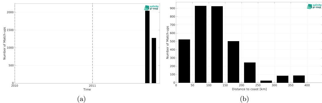
Figure 2: Number of match-ups between TSG (SAMOS) and Aquarius SSS L4 OI v5 - Monthly (IPRC) SSS as a function of time (a) and as function of the distance to coast (b) over the Arctic Ocean Pi-MEP region and for the full satellite product period.
