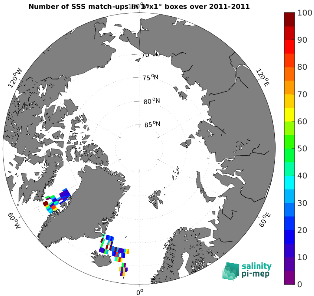
Figure 5: Number of SSS match-ups between TSG (SAMOS) SSS and the Aquarius SSS L4 OI v5 - Monthly (IPRC) SSS product for the Arctic Ocean Pi-MEP region over 1^{\circ} \times 1^{\circ} boxes and for the full satellite product period.
