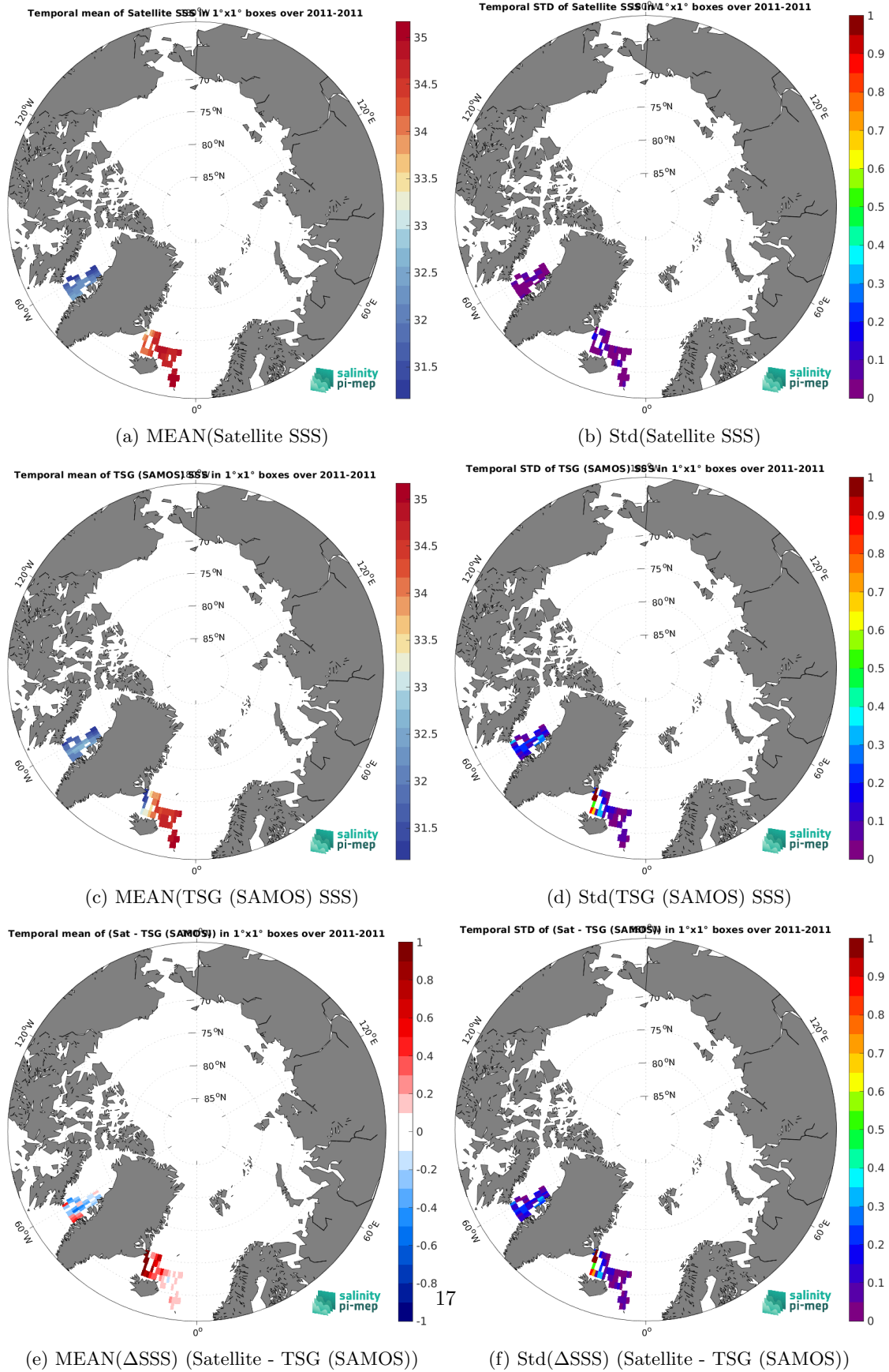
Figure 7: Temporal mean (left) and Std (right) of SSS from Aquarius SSS L4 OI v5 - Monthly (IPRC) (top), TSG (SAMOS) (middle), and of \Delta SSS (Satellite - TSG (SAMOS)). Only match-up pairs are used to generate these maps.
