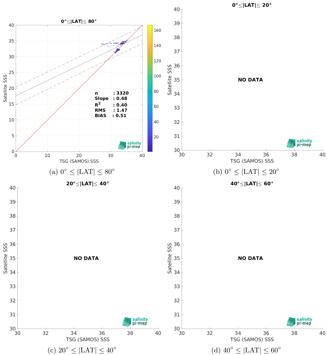
Figure 10: Contour maps of the concentration of Aquarius SSS L4 OI v5 - Monthly (IPRC) SSS (y-axis) versus TSG (SAMOS) SSS (x-axis) at match-up pairs for different latitude bands. For each plot, the red line shows x=y . The black thin and dashed lines indicate a linear fit through the data cloud and the \pm 95\% confidence levels, respectively. The number match-up pairs n , the slope and R^2 coefficient of the linear fit, the root mean square (RMS) and the mean bias between satellite and in situ data are indicated for each latitude band in each plots.
