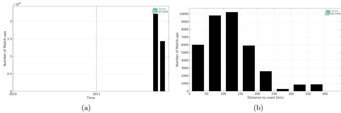
Figure 1: Number of match-ups between TSG (SAMOS) and Aquarius SSS L4 OI v5 - Monthly (IPRC) SSS as a function of time (a) and as function of the distance to coast (b) over the Arctic Ocean Pi-MEP region and for the full satellite product period.
