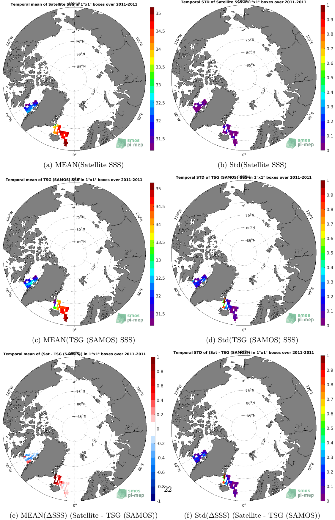
Figure 6: Temporal mean (left) and Std (right) of SSS from Aquarius SSS L4 OI v5 - Monthly (IPRC) (top), TSG (SAMOS) (middle), and of \Delta SSS (Satellite - TSG (SAMOS)). Only match-up pairs are used to generate these maps.
