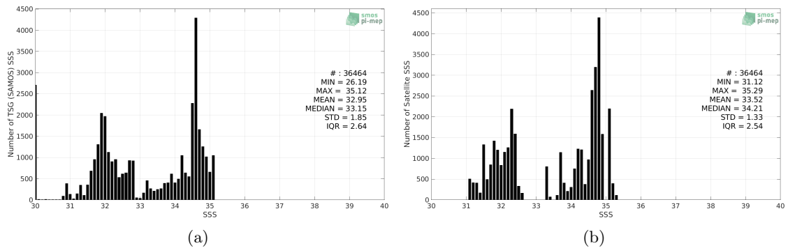
Figure 2: Histograms of SSS from TSG (SAMOS) (a) and Aquarius SSS L4 OI v5 - Monthly (IPRC) (b) considering all match-up pairs per bins of 0.1 over the Arctic Ocean Pi-MEP region and for the full satellite product period.
