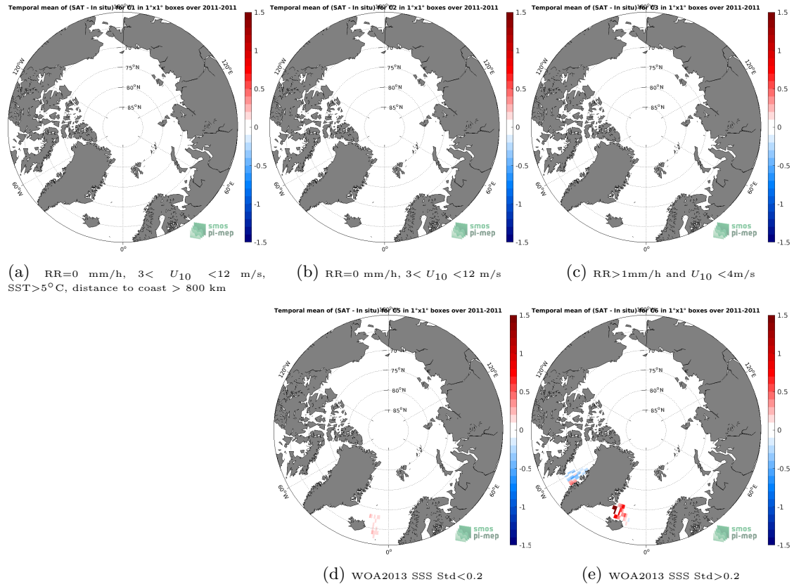
Figure 12: Temporal mean gridded over spatial boxes of size 1^{\circ}\times 1^{\circ} of \Delta\text{SSS} (Aquarius SSS L4 OI v5 - Monthly (IPRC) - TSG (SAMOS)) for 5 different subdatasets corresponding to:RR=0 mm/h, 3 < U_{10} < 12 m/s, SST >5^{\circ}\text{C} , distance to coast > 800 km (a), RR=0 mm/h, 3 < U_{10} < 12 m/s (b), RR >1 mm/h and U_{10} < 4 m/s (c), WOA2013 SSS Std <0.2 (d), WOA2013 SSS Std >0.2 (e).
