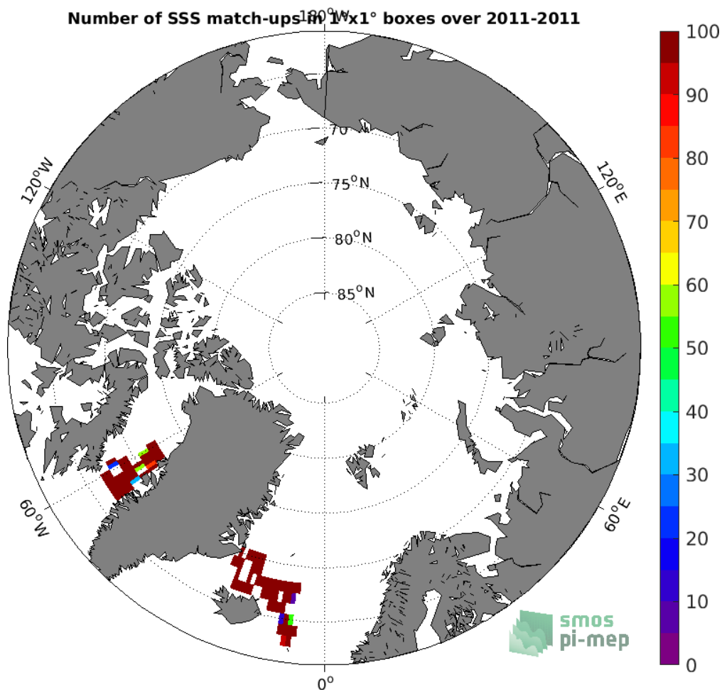
Figure 4: Number of SSS match-ups between TSG (SAMOS) SSS and the Aquarius SSS L4 OI v5 - Monthly (IPRC) SSS product for the Arctic Ocean Pi-MEP region over 1^\circ \times 1^\circ boxes and for the full satellite product period.
