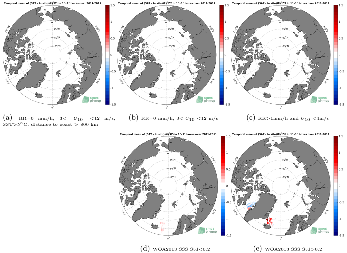
Figure 12: Temporal mean gridded over spatial boxes of size 1°x1° of \Delta SSS (Aquarius-L4-IPRC-V5-MONTHLY - TSG-SAMOS) for 5 different subdatasets corresponding to:RR=0 mm/h, 3 < U_{10} < 12 m/s, SST > 5°C, distance to coast > 800 km (a), RR=0 mm/h, 3 < U_{10} < 12 m/s (b), RR > 1mm/h and U_{10} < 4 m/s (c), WOA2013 SSS Std < 0.2 (d), WOA2013 SSS Std > 0.2 (e).
