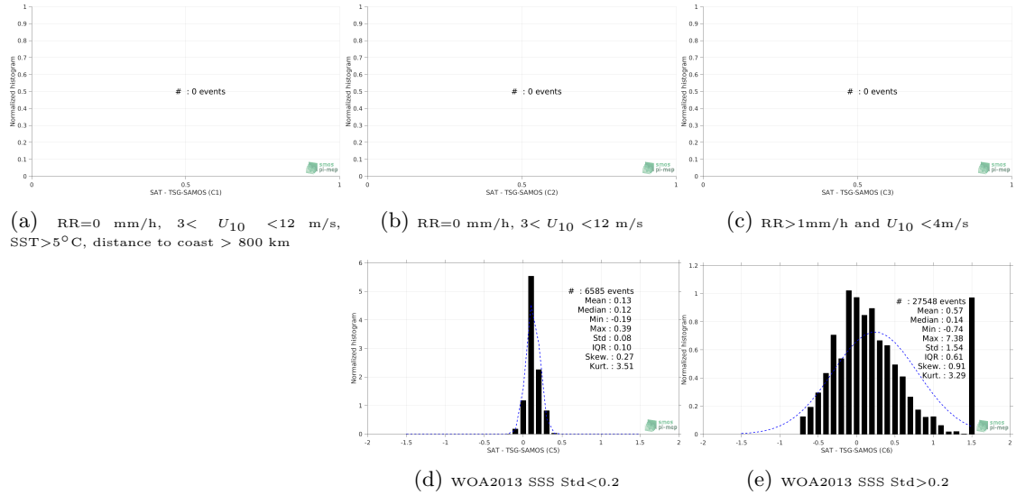
Figure 13: Normalized histogram of \Delta SSS (Aquarius-L4-IPRC-V5-MONTHLY - TSG-SAMOS) for 5 different subdatasets corresponding to: RR=0 mm/h, 3 < U_{10} < 12 m/s, SST>5°C, distance to coast > 800 km (a), RR=0 mm/h, 3 < U_{10} < 12 m/s (b), RR>1mm/h and U_{10} < 4 m/s (c), WOA2013 SSS Std<0.2 (d), WOA2013 SSS Std>0.2 (e).
