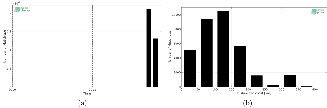
Figure 1: Number of match-ups between TSG-SAMOS and Aquarius-L4-IPRC-V5-MONTHLY SSS as a function of time (a) and as function of the distance to coast (b) over the Arctic Ocean Pi-MEP region and for the full satellite product period.
