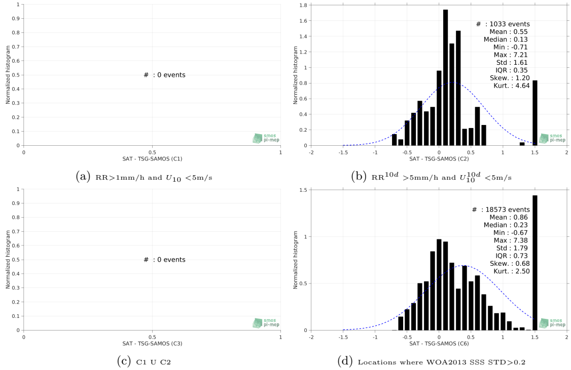
Figure 13: Normalized histogram of \Delta\text{SSS} (Aquarius-L4-IPRC-V5-MONTHLY - TSG-SAMOS) for 6 different subdatasets corresponding to: RR > 1\text{mm/h} and U_{10} < 5\text{m/s} (a), RR^{10d} > 5\text{mm/h} and U_{10}^{10d} < 5\text{m/s} (b), C1 \cup C2 (c), Locations where WOA2013 SSS STD > 0.2 (d).
