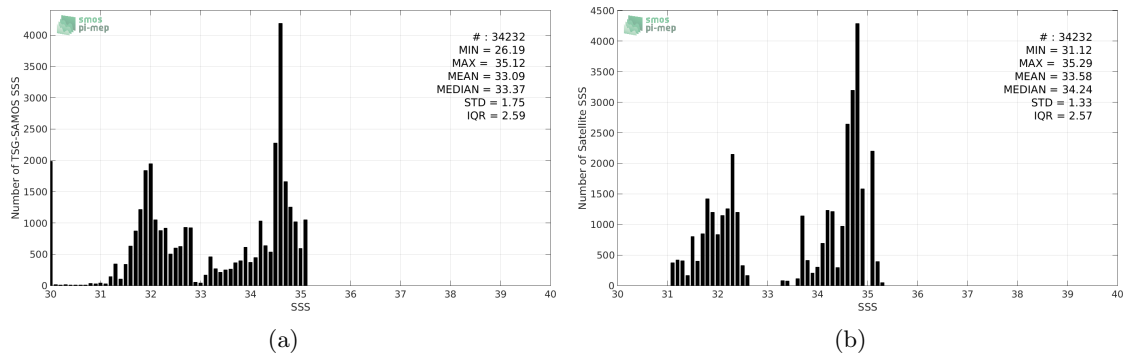
Figure 2: Histograms of SSS from TSG-SAMOS (a) and Aquarius-L4-IPRC-V5-MONTHLY (b) considering all match-up pairs per bins of 0.1 over the Arctic Ocean Pi-MEP region and for the full satellite product period.
