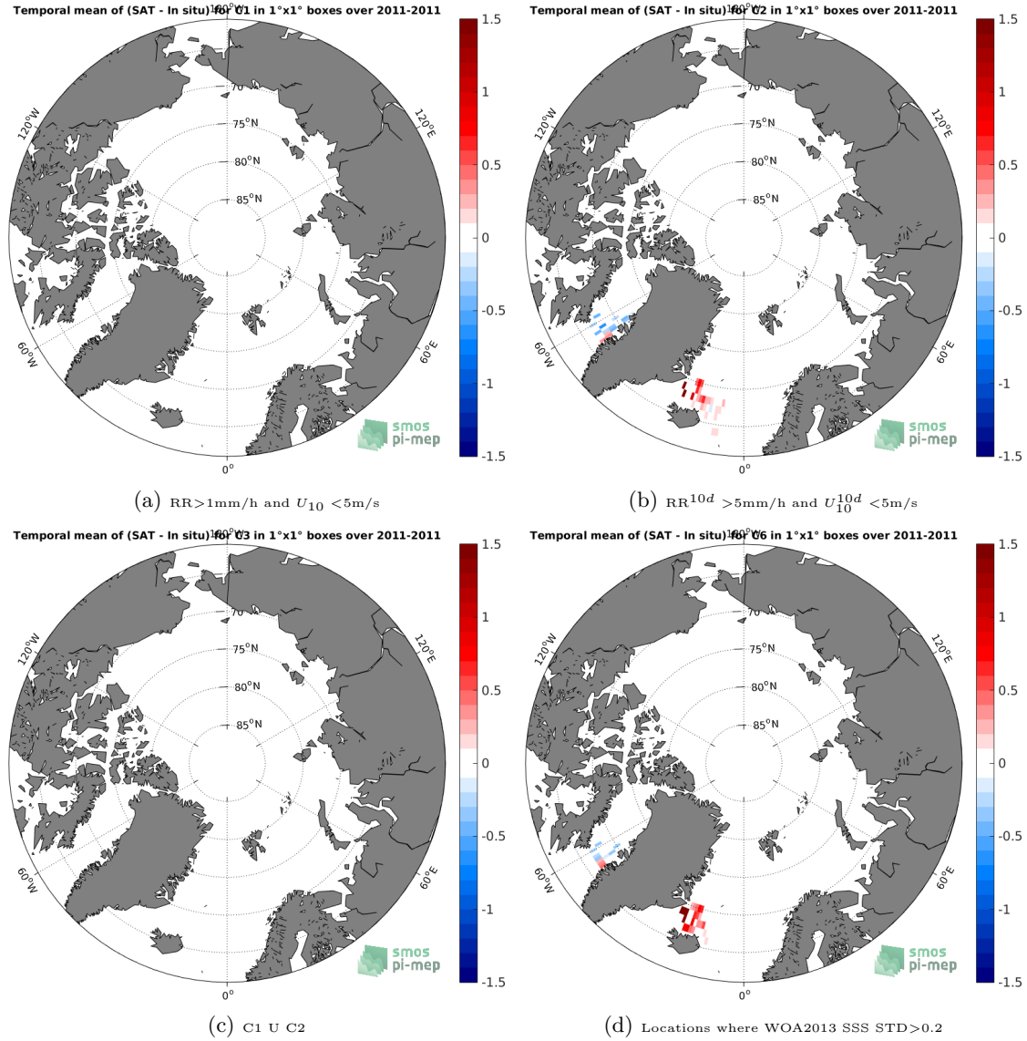
Figure 12: Temporal mean gridded over spatial boxes of size 1^\circ \times 1^\circ of \Delta SSS (Aquarius-L4-IPRC-V5-MONTHLY - TSG-SAMOS) for 4 different subdatasets corresponding to: RR > 1\text{mm/h} and U_{10} < 5\text{m/s} (a), RR^{10d} > 5\text{mm/h} and U_{10}^{10d} < 5\text{m/s} (b), C1 U C2 (c), Locations where WOA2013 SSS STD > 0.2 (d).
