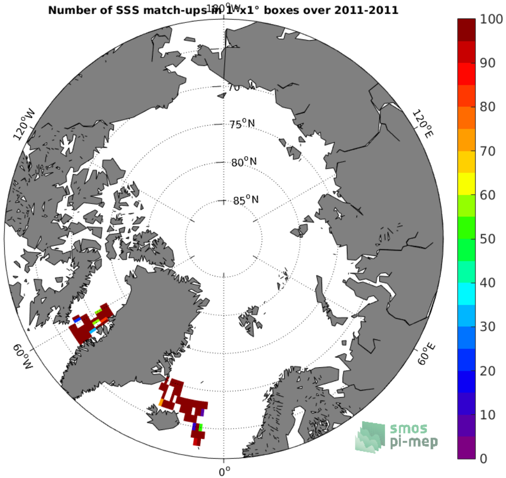
Figure 4: Number of SSS match-ups between TSG-SAMOS SSS and the Aquarius-L4-IPRC-V5-MONTHLY SSS product for the Arctic Ocean Pi-MEP region over 1^\circ \times 1^\circ boxes and for the full satellite product period.
