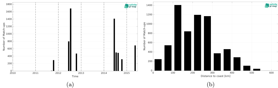
Figure 2: Number of match-ups between TSG (Polarstern) and Aquarius SSS L4 OI v5 - Monthly (IPRC) SSS as a function of time (a) and as function of the distance to coast (b) over the Arctic Ocean Pi-MEP region and for the full satellite product period.
