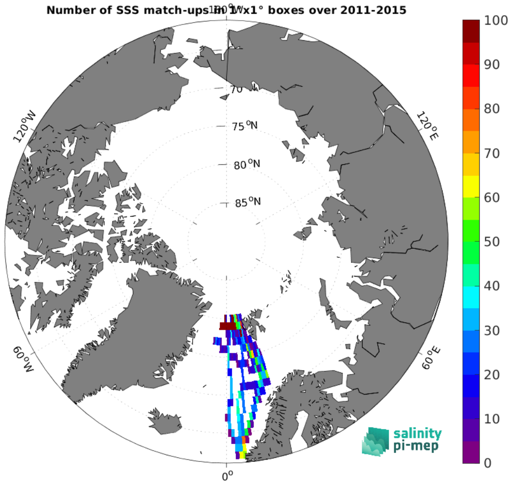
Figure 5: Number of SSS match-ups between TSG (Polarstern) SSS and the Aquarius SSS L4 OI v5 - Monthly (IPRC) SSS product for the Arctic Ocean Pi-MEP region over 1^\circ \times 1^\circ boxes and for the full satellite product period.
