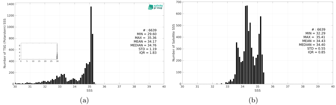
Figure 3: Histograms of SSS from TSG (Polarstern) (a) and Aquarius SSS L4 OI v5 - Monthly (IPRC) (b) considering all match-up pairs per bins of 0.1 over the Arctic Ocean Pi-MEP region and for the full satellite product period.
