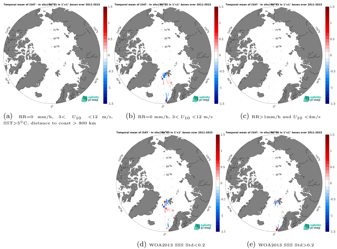
Figure 14: Temporal mean gridded over spatial boxes of size 1^\circ \times 1^\circ of \Delta SSS (Aquarius SSS L4 OI v5 - Monthly (IPRC) - TSG (Polarstern)) for 5 different subdatasets corresponding to:RR=0 mm/h, 3 < U_{10} < 12 m/s, SST > 5^\circ\text{C} , distance to coast > 800 km (a), RR=0 mm/h, 3 < U_{10} < 12 m/s (b), RR > 1 mm/h and U_{10} < 4 m/s (c), WOA2013 SSS Std < 0.2 (d), WOA2013 SSS Std > 0.2 (e).
