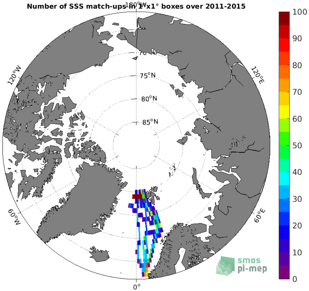
Figure 4: Number of SSS match-ups between TSG (Polarstern) SSS and the Aquarius SSS L4 OI v5 - Monthly (IPRC) SSS product for the Arctic Ocean Pi-MEP region over 1^{\circ} \times 1^{\circ} boxes and for the full satellite product period.
