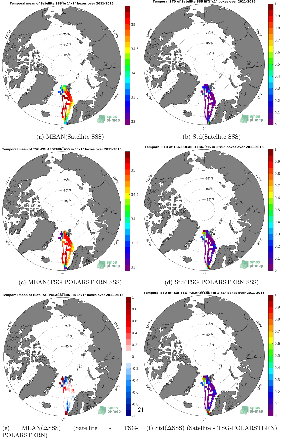
Figure 6: Temporal mean (left) and Std (right) of SSS from Aquarius-L4-IPRC-V5-MONTHLY (top), TSG-POLARSTERN (middle), and of \Delta SSS (Satellite - TSG-POLARSTERN). Only match-up pairs are used to generate these maps.
