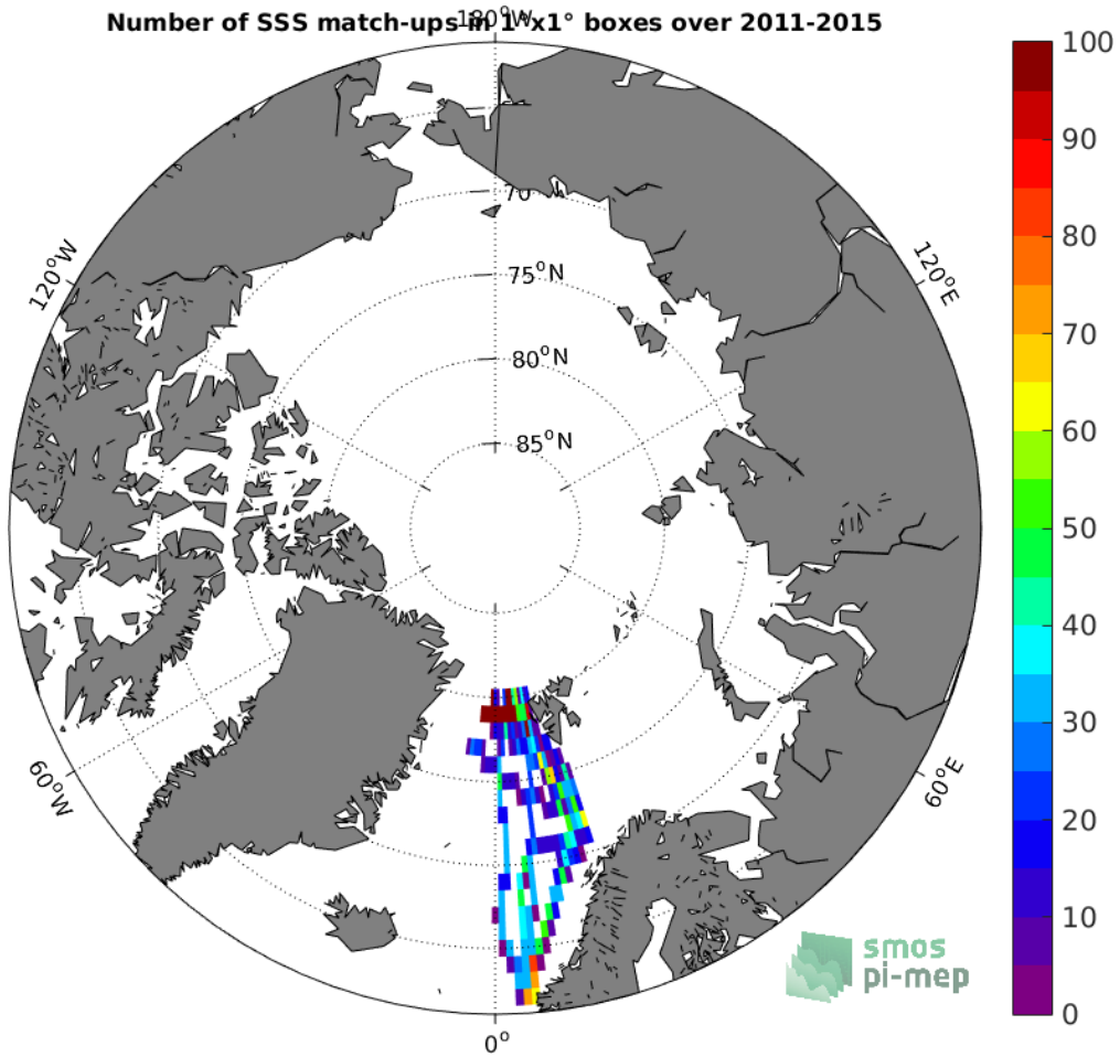
Figure 4: Number of SSS match-ups between TSG-POLARSTERN SSS and the Aquarius-L4-IPRC-V5-MONTHLY SSS product for the Arctic Ocean Pi-MEP region over 1^\circ \times 1^\circ boxes and for the full satellite product period.
