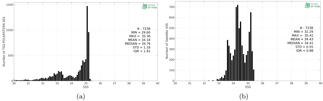
Figure 2: Histograms of SSS from TSG-POLARSTERN (a) and Aquarius-L4-IPRC-V5-MONTHLY (b) considering all match-up pairs per bins of 0.1 over the Arctic Ocean Pi-MEP region and for the full satellite product period.
