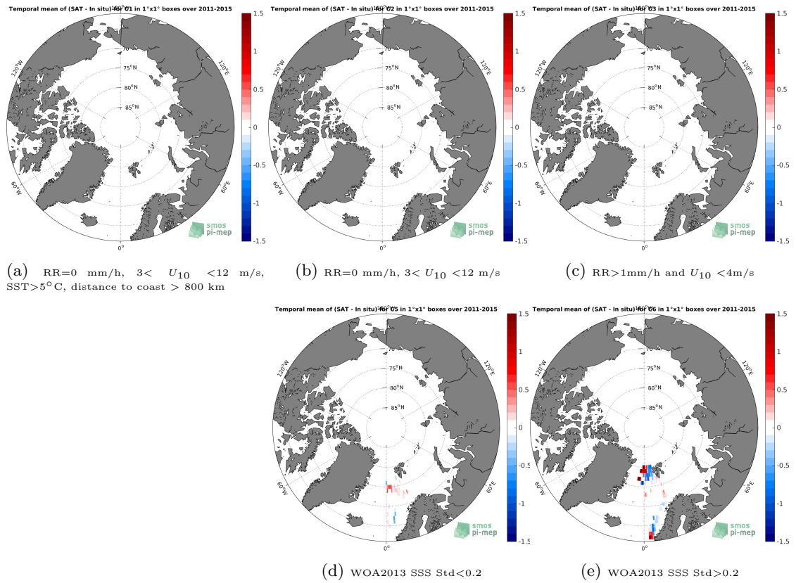
Figure 12: Temporal mean gridded over spatial boxes of size 1^\circ \times 1^\circ of \Delta SSS (Aquarius-L4-IPRC-V5-MONTHLY - TSG-POLARSTERN) for 5 different subdatasets corresponding to:RR=0 mm/h, 3 < U_{10} < 12 m/s, SST >5^\circ C, distance to coast > 800 km (a), RR=0 mm/h, 3 < U_{10} < 12 m/s (b), RR >1 mm/h and U_{10} < 4 m/s (c), WOA2013 SSS Std <0.2 (d), WOA2013 SSS Std >0.2 (e).
