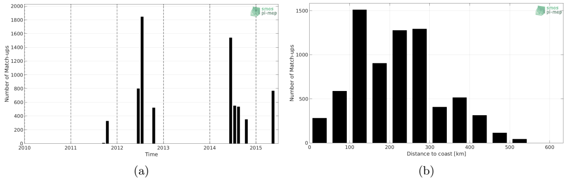
Figure 1: Number of match-ups between TSG-POLARSTERN and Aquarius-L4-IPRC-V5-MONTHLY SSS as a function of time (a) and as function of the distance to coast (b) over the Arctic Ocean Pi-MEP region and for the full satellite product period.
