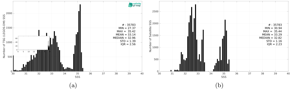
Figure 3: Histograms of SSS from TSG (LEGOS-DM) (a) and Aquarius SSS L4 OI v5 - Monthly (IPRC) (b) considering all match-up pairs per bins of 0.1 over the Arctic Ocean Pi-MEP region and for the full satellite product period.
