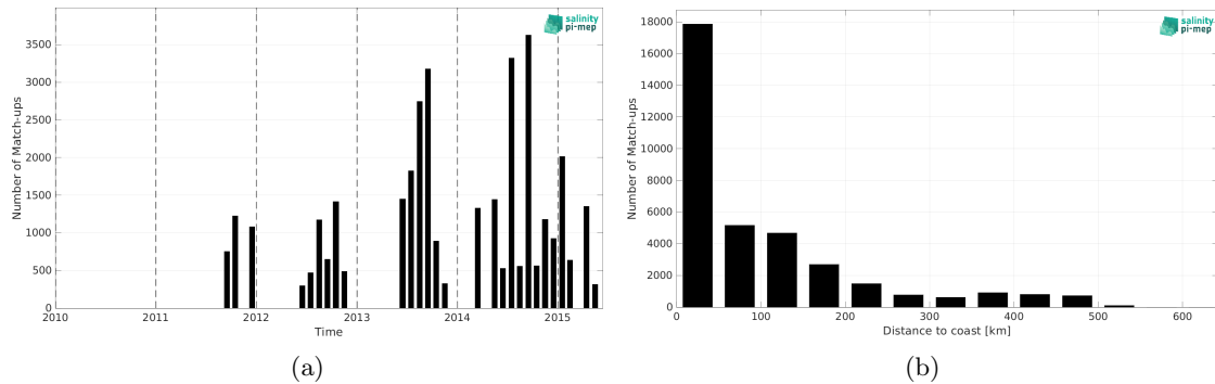
Figure 2: Number of match-ups between TSG (LEGOS-DM) and Aquarius SSS L4 OI v5 - Monthly (IPRC) SSS as a function of time (a) and as function of the distance to coast (b) over the Arctic Ocean Pi-MEP region and for the full satellite product period.
