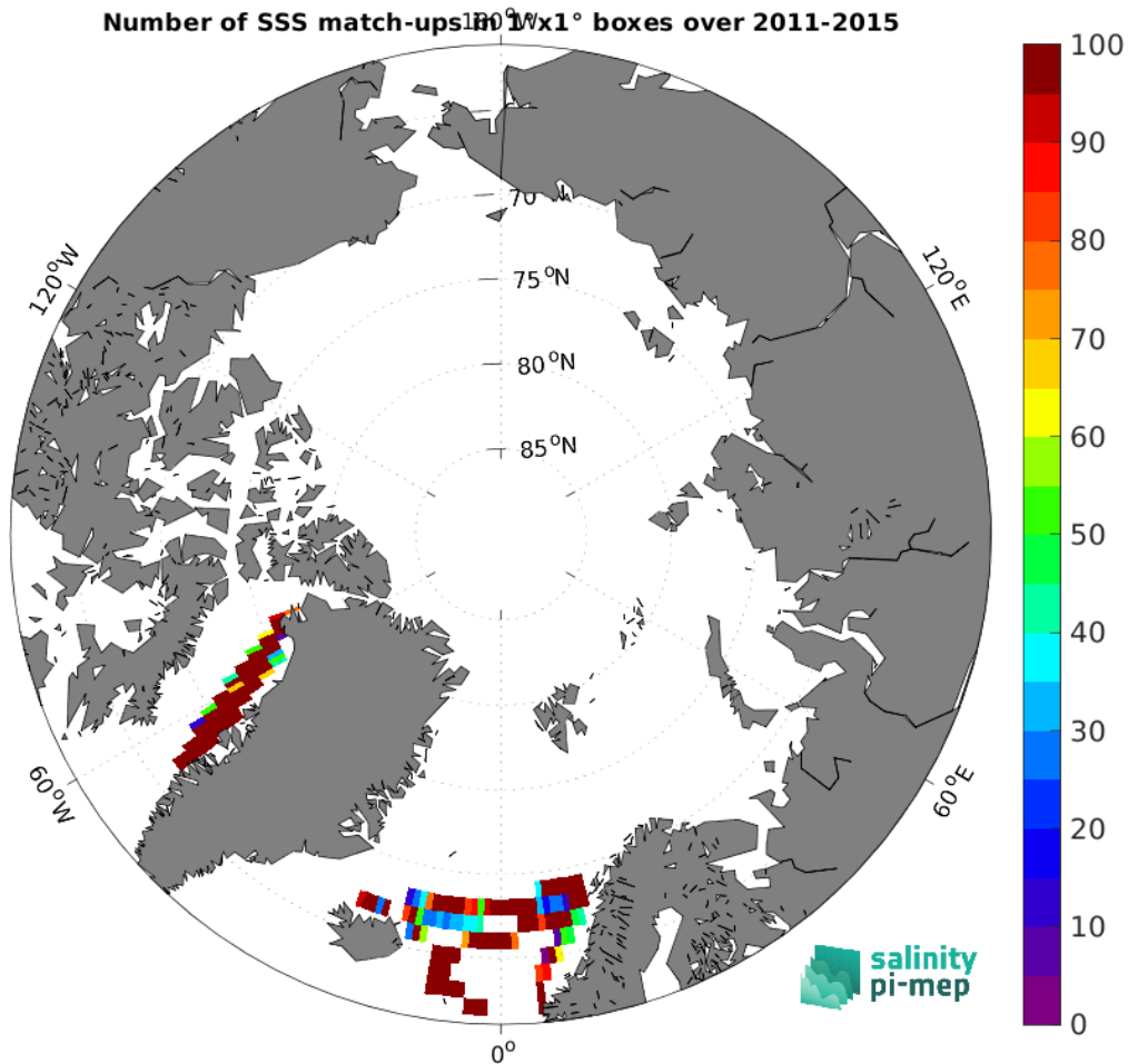
Figure 5: Number of SSS match-ups between TSG (LEGOS-DM) SSS and the Aquarius SSS L4 OI v5 - Monthly (IPRC) SSS product for the Arctic Ocean Pi-MEP region over 1^\circ \times 1^\circ boxes and for the full satellite product period.
