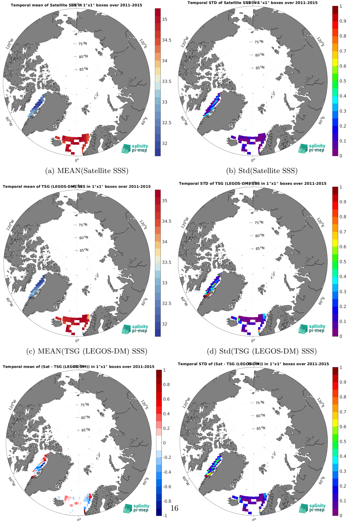
(e) MEAN( \Delta SSS) (Satellite - TSG (LEGOS-DM)) (f) Std( \Delta SSS) (Satellite - TSG (LEGOS-DM)) Figure 7: Temporal mean (left) and Std (right) of SSS from Aquarius SSS L4 OI v5 - Monthly (IPRC) (top), TSG (LEGOS-DM) (middle), and of \Delta SSS (Satellite - TSG (LEGOS-DM)). Only match-up pairs are used to generate these maps.
