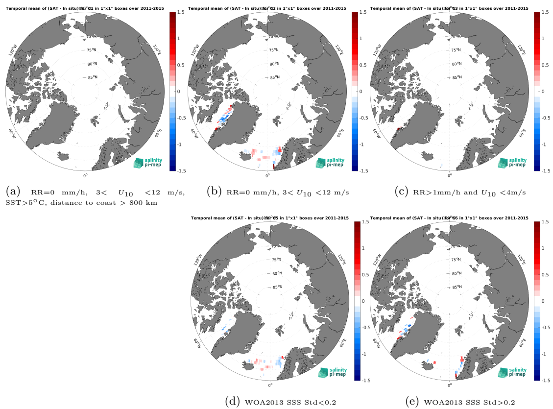
Figure 14: Temporal mean gridded over spatial boxes of size 1^\circ \times 1^\circ of \Delta SSS (Aquarius SSS L4 OI v5 - Monthly (IPRC) - TSG (LEGOS-DM)) for 5 different subdatasets corresponding to:RR=0 mm/h, 3 < U_{10} < 12 m/s, SST >5^\circ\text{C} , distance to coast > 800 km (a), RR=0 mm/h, 3 < U_{10} < 12 m/s (b), RR >1 mm/h and U_{10} < 4 m/s (c), WOA2013 SSS Std <0.2 (d), WOA2013 SSS Std >0.2 (e).
