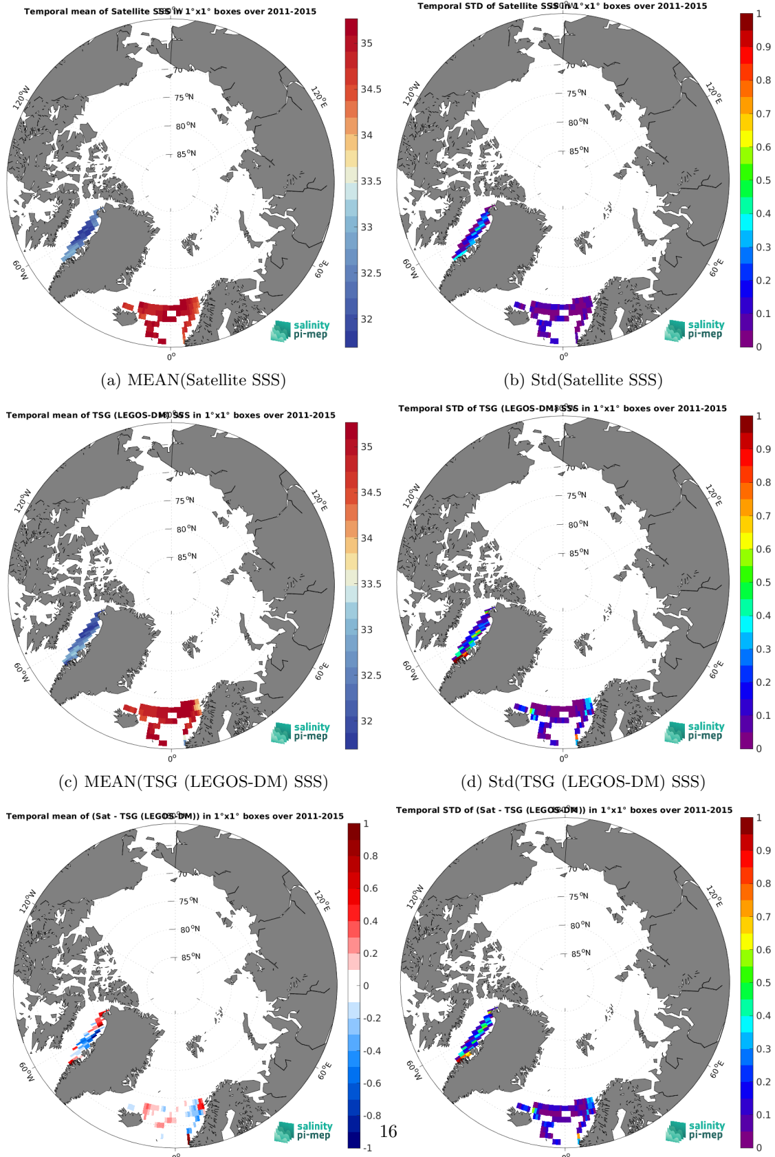
(e) MEAN( \Delta SSS) (Satellite - TSG (LEGOS-DM)) (f) Std( \Delta SSS) (Satellite - TSG (LEGOS-DM)) Figure 6: Temporal mean (left) and Std (right) of SSS from Aquarius SSS L4 OI v5 - Monthly (IPRC) (top), TSG (LEGOS-DM) (middle), and of \Delta SSS (Satellite - TSG (LEGOS-DM)). Only match-up pairs are used to generate these maps.
