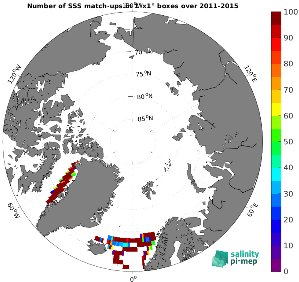
Figure 4: Number of SSS match-ups between TSG (LEGOS-DM) SSS and the Aquarius SSS L4 OI v5 - Monthly (IPRC) SSS product for the Arctic Ocean Pi-MEP region over 1^\circ \times 1^\circ boxes and for the full satellite product period.
