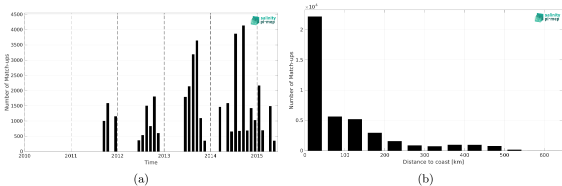
Figure 1: Number of match-ups between TSG (LEGOS-DM) and Aquarius SSS L4 OI v5 - Monthly (IPRC) SSS as a function of time (a) and as function of the distance to coast (b) over the Arctic Ocean Pi-MEP region and for the full satellite product period.
