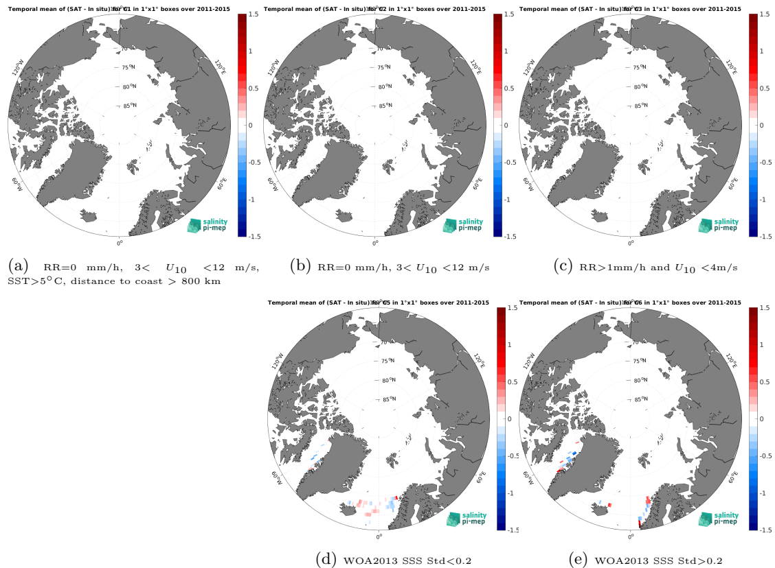
Figure 12: Temporal mean gridded over spatial boxes of size 1^{\circ}\times 1^{\circ} of \Delta\text{SSS} (Aquarius SSS L4 OI v5 - Monthly (IPRC) - TSG (LEGOS-DM)) for 5 different subdatasets corresponding to:RR=0 mm/h, 3 < U_{10} < 12 m/s, SST > 5^{\circ}\text{C} , distance to coast > 800 km (a), RR=0 mm/h, 3 < U_{10} < 12 m/s (b), RR > 1 mm/h and U_{10} < 4 m/s (c), WOA2013 SSS Std < 0.2 (d), WOA2013 SSS Std > 0.2 (e).
