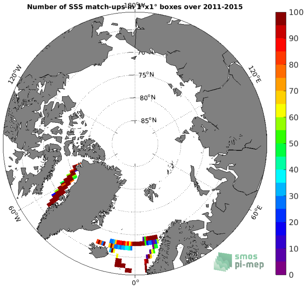
Figure 4: Number of SSS match-ups between TSG (LEGOS-DM) SSS and the Aquarius SSS L4 OI v5 - Monthly (IPRC) SSS product for the Arctic Ocean Pi-MEP region over 1°x1° boxes and for the full satellite product period.
