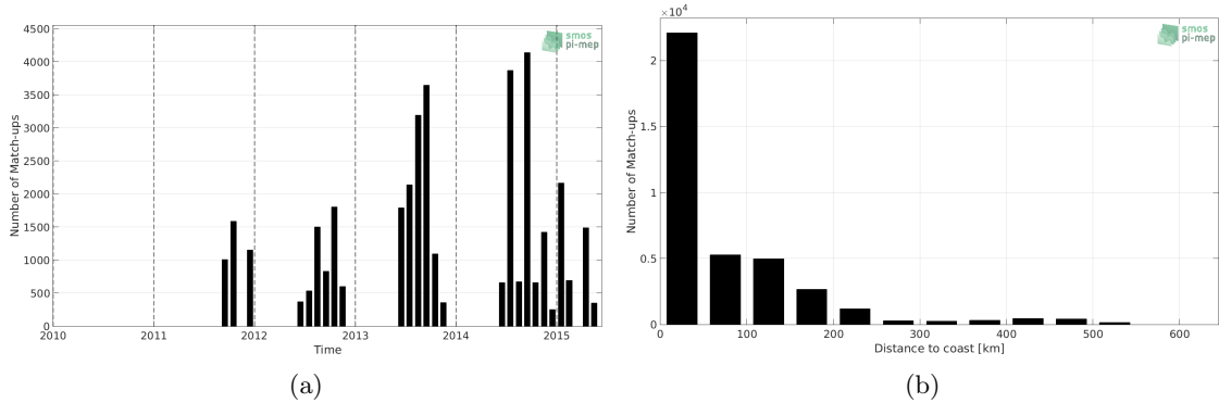
Figure 1: Number of match-ups between TSG-LEGOS-DM and Aquarius-L4-IPRC-V5-MONTHLY SSS as a function of time (a) and as function of the distance to coast (b) over the Arctic Ocean Pi-MEP region and for the full satellite product period.
