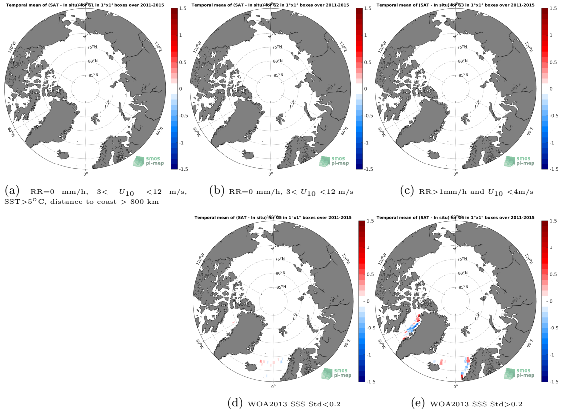
Figure 12: Temporal mean gridded over spatial boxes of size 1^{\circ}\times 1^{\circ} of \Delta\text{SSS} (Aquarius-L4-IPRC-V5-MONTHLY - TSG-LEGOS-DM) for 5 different subdatasets corresponding to:RR=0 mm/h, 3 < U_{10} < 12 m/s, SST >5^{\circ}\text{C} , distance to coast > 800 km (a), RR=0 mm/h, 3 < U_{10} < 12 m/s (b), RR >1 mm/h and U_{10} < 4 m/s (c), WOA2013 SSS Std <0.2 (d), WOA2013 SSS Std >0.2 (e).
