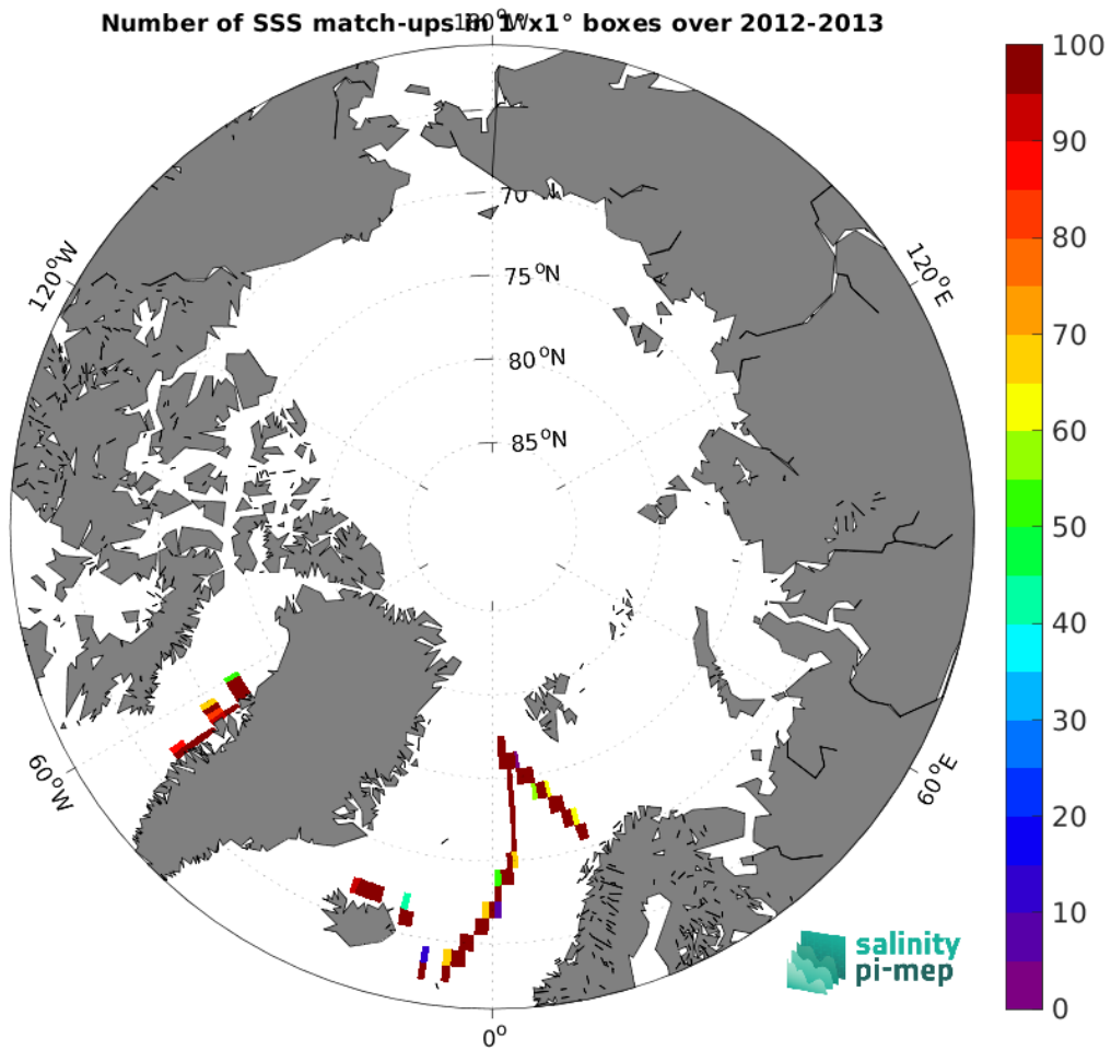
Figure 4: Number of SSS match-ups between TSG (GOSUD-Sailing-ship) SSS and the Aquarius SSS L4 OI v5 - Monthly (IPRC) SSS product for the Arctic Ocean Pi-MEP region over 1^\circ \times 1^\circ boxes and for the full satellite product period.
