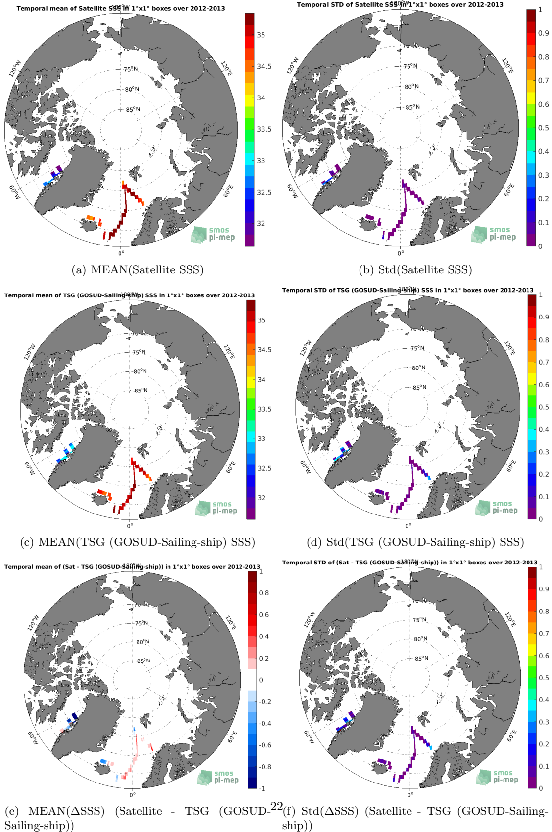
Figure 6: Temporal mean (left) and Std (right) of SSS from Aquarius SSS L4 OI v5 - Monthly (IPRC) (top), TSG (GOSUD-Sailing-ship) (middle), and of \Delta SSS (Satellite - TSG (GOSUD-Sailing-ship)). Only match-up pairs are used to generate these maps.
