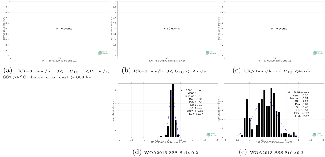
Figure 13: Normalized histogram of \Delta SSS (Aquarius-L4-IPRC-V5-MONTHLY - TSG-GOSUD-Sailing-ship) for 5 different subdatasets corresponding to: RR=0 mm/h, 3 < U_{10} < 12 m/s, SST >5^{\circ}\text{C} , distance to coast > 800 km (a), RR=0 mm/h, 3 < U_{10} < 12 m/s (b), RR >1 mm/h and U_{10} < 4 m/s (c), WOA2013 SSS Std <0.2 (d), WOA2013 SSS Std >0.2 (e).
