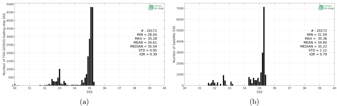
Figure 2: Histograms of SSS from TSG-GOSUD-Sailing-ship (a) and Aquarius-L4-IPRC-V5-MONTHLY (b) considering all match-up pairs per bins of 0.1 over the Arctic Ocean Pi-MEP region and for the full satellite product period.
