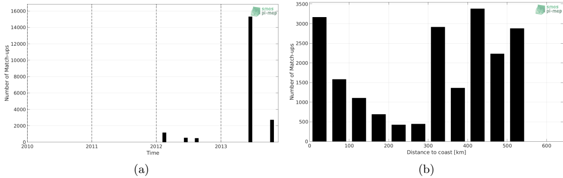
Figure 1: Number of match-ups between TSG-GOSUD-Sailing-ship and Aquarius-L4-IPRC-V5-MONTHLY SSS as a function of time (a) and as function of the distance to coast (b) over the Arctic Ocean Pi-MEP region and for the full satellite product period.
