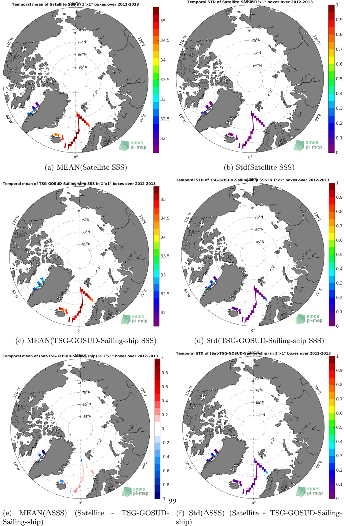
Figure 6: Temporal mean (left) and Std (right) of SSS from Aquarius-L4-IPRC-V5-MONTHLY (top), TSG-GOSUD-Sailing-ship (middle), and of \Delta SSS (Satellite - TSG-GOSUD-Sailing-ship). Only match-up pairs are used to generate these maps.
