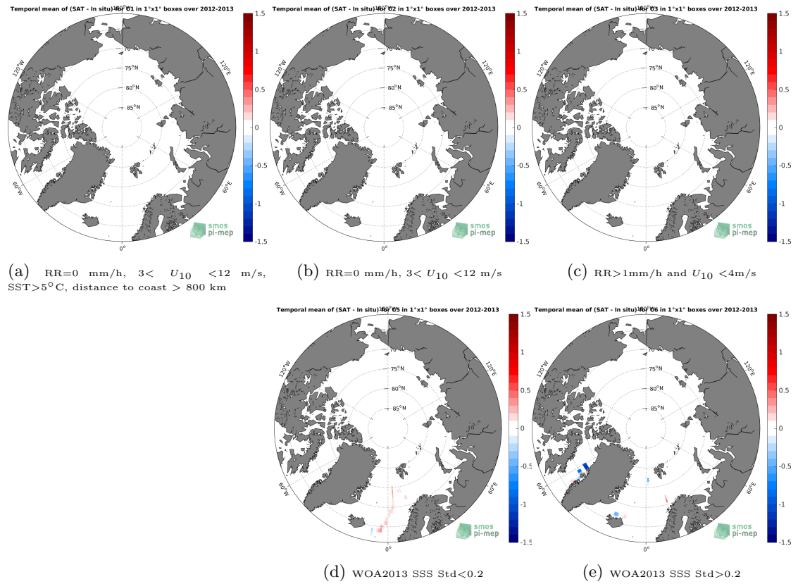
Figure 12: Temporal mean gridded over spatial boxes of size 1^\circ \times 1^\circ of \Delta SSS (Aquarius-L4-IPRC-V5-MONTHLY - TSG-GOSUD-Sailing-ship) for 5 different subdatasets corresponding to:RR=0 mm/h, 3 < U_{10} < 12 m/s, SST > 5^\circ\text{C} , distance to coast > 800 km (a), RR=0 mm/h, 3 < U_{10} < 12 m/s (b), RR > 1 mm/h and U_{10} < 4 m/s (c), WOA2013 SSS Std < 0.2 (d), WOA2013 SSS Std > 0.2 (e).
