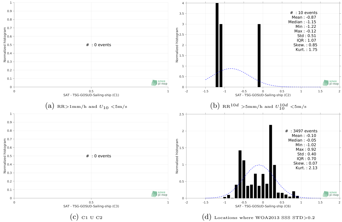
Figure 13: Normalized histogram of \Delta\text{SSS} (Aquarius-L4-IPRC-V5-MONTHLY - TSG-GOSUD-Sailing-ship) for 6 different subdatasets corresponding to: RR > 1\text{mm/h} and U_{10} < 5\text{m/s} (a), RR^{10d} > 5\text{mm/h} and U_{10}^{10d} < 5\text{m/s} (b), C1 \cup C2 (c), Locations where WOA2013 SSS STD > 0.2 (d).
