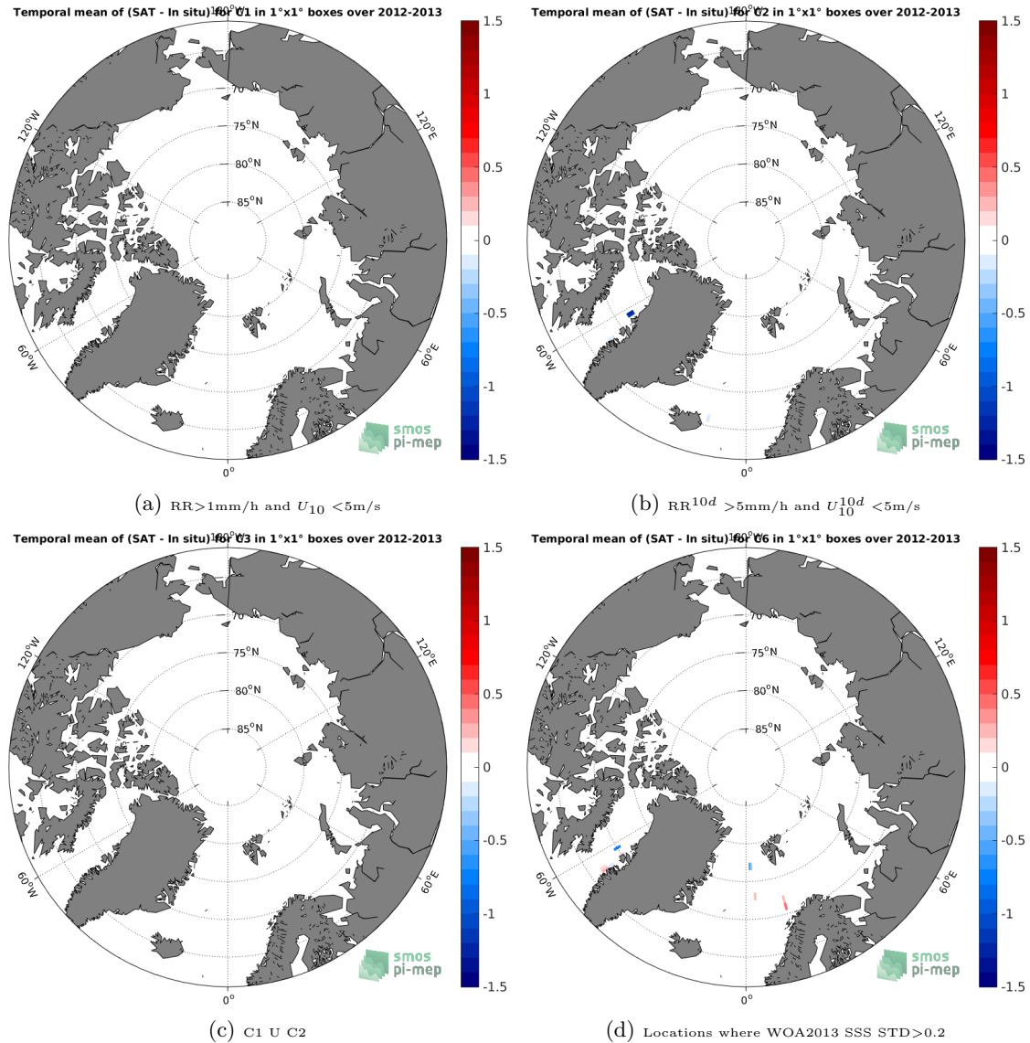
Figure 12: Temporal mean gridded over spatial boxes of size 1^\circ \times 1^\circ of \Delta SSS (Aquarius-L4-IPRC-V5-MONTHLY - TSG-GOSUD-Sailing-ship) for 4 different subdatasets corresponding to: RR > 1\text{mm/h} and U_{10} < 5\text{m/s} (a), RR^{10d} > 5\text{mm/h} and U_{10}^{10d} < 5\text{m/s} (b), C1 U C2 (c), Locations where WOA2013 SSS STD > 0.2 (d).
