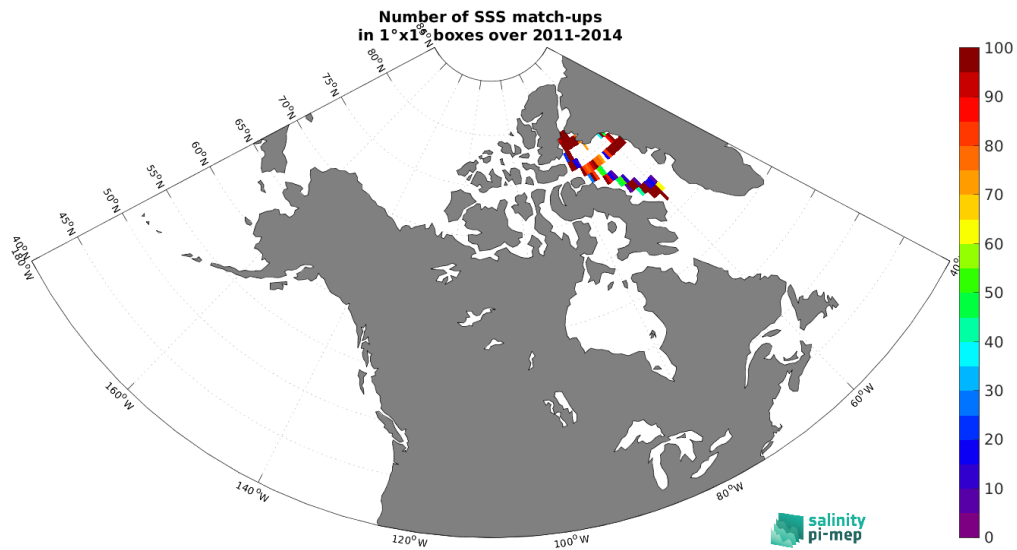
Figure 5: Number of SSS match-ups between TSG (Amundsen) SSS and the Aquarius SSS L4 OI v5 - Monthly (IPRC) SSS product for the Arctic Ocean Pi-MEP region over 1°x1° boxes and for the full satellite product period.
