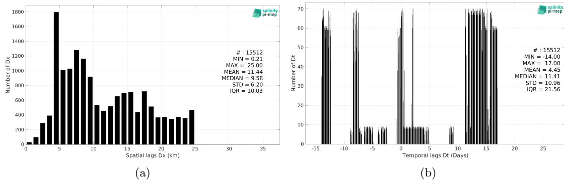
Figure 6: Histograms of the spatial (a) and temporal (b) lags between the location/time of the TSG (Amundsen) measurement and the date of the corresponding Aquarius SSS L4 OI v5 - Monthly (IPRC) SSS pixel.
