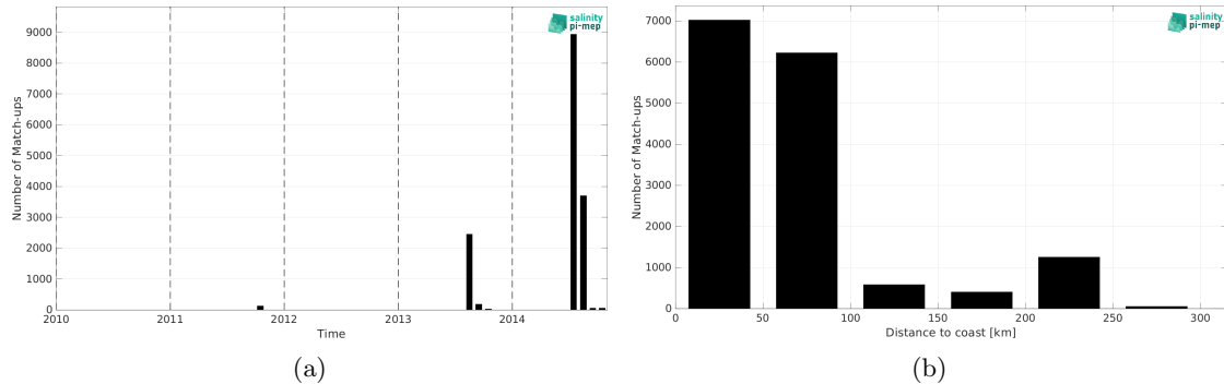
Figure 2: Number of match-ups between TSG (Amundsen) and Aquarius SSS L4 OI v5 - Monthly (IPRC) SSS as a function of time (a) and as function of the distance to coast (b) over the Arctic Ocean Pi-MEP region and for the full satellite product period.
