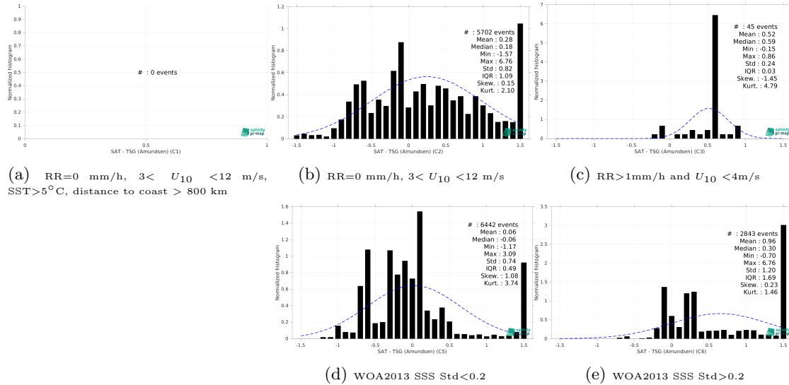
Figure 15: Normalized histogram of \Delta SSS (Aquarius SSS L4 OI v5 - Monthly (IPRC) - TSG (Amundsen)) for 5 different subdatasets corresponding to: RR=0 mm/h, 3 < U_{10} < 12 m/s, SST>5°C, distance to coast > 800 km (a), RR=0 mm/h, 3 < U_{10} < 12 m/s (b), RR>1mm/h and U_{10} < 4 m/s (c), WOA2013 SSS Std<0.2 (d), WOA2013 SSS Std>0.2 (e).
