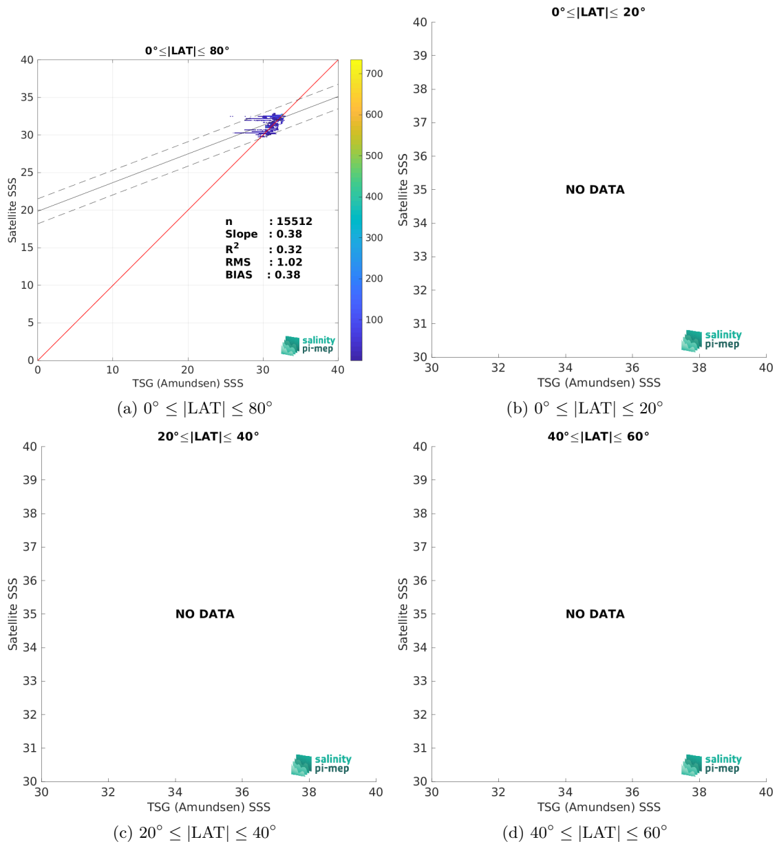
Figure 10: Contour maps of the concentration of Aquarius SSS L4 OI v5 - Monthly (IPRC) SSS (y-axis) versus TSG (Amundsen) SSS (x-axis) at match-up pairs for different latitude bands. For each plot, the red line shows x=y . The black thin and dashed lines indicate a linear fit through the data cloud and the \pm 95\% confidence levels, respectively. The number match-up pairs n , the slope and R^2 coefficient of the linear fit, the root mean square (RMS) and the mean bias between satellite and in situ data are indicated for each latitude band in each plots.
