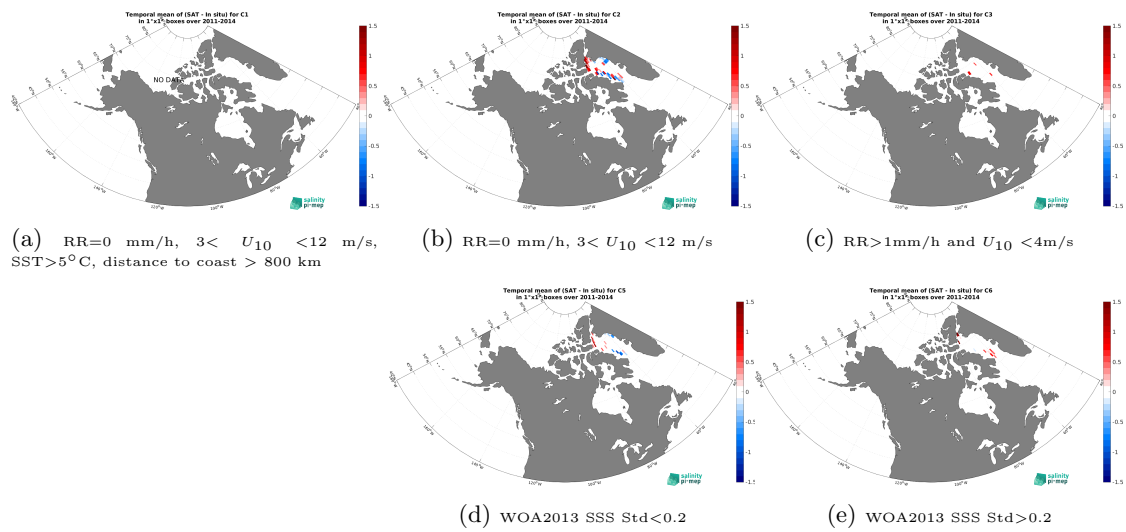
Figure 14: Temporal mean gridded over spatial boxes of size 1^\circ \times 1^\circ of \Delta\text{SSS} (Aquarius SSS L4 OI v5 - Monthly (IPRC) - TSG (Amundsen)) for 5 different subdatasets corresponding to: RR=0 mm/h, 3 < U_{10} < 12 m/s, SST > 5°C, distance to coast > 800 km (a), RR=0 mm/h, 3 < U_{10} < 12 m/s (b), RR > 1mm/h and U_{10} < 4 m/s (c), WOA2013 SSS Std < 0.2 (d), WOA2013 SSS Std > 0.2 (e).
