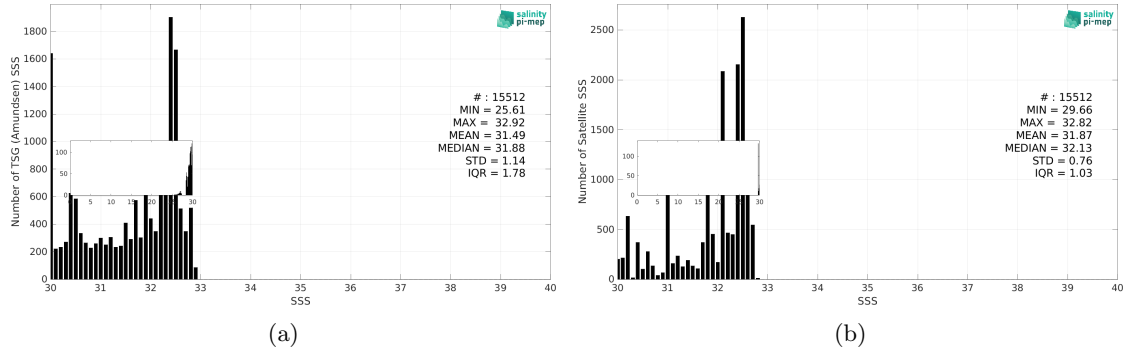
Figure 3: Histograms of SSS from TSG (Amundsen) (a) and Aquarius SSS L4 OI v5 - Monthly (IPRC) (b) considering all match-up pairs per bins of 0.1 over the Arctic Ocean Pi-MEP region and for the full satellite product period.
