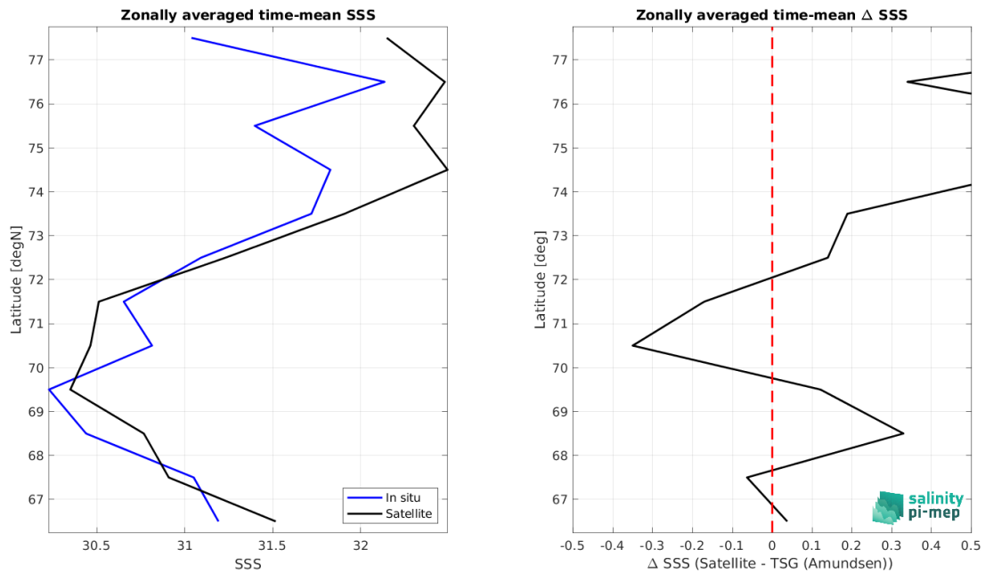
Figure 9: Left panel: Zonal mean SSS from Aquarius SSS L4 OI v5 - Monthly (IPRC) satellite product (black) and from TSG (Amundsen) (blue). Right panel: Zonal mean of \Delta SSS (Satellite - TSG (Amundsen)) for all the collected Pi-MEP match-up pairs estimated over the full satellite product period.
