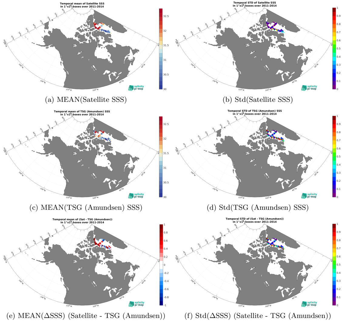
Figure 7: Temporal mean (left) and Std (right) of SSS from Aquarius SSS L4 OI v5 - Monthly (IPRC) (top), TSG (Amundsen) (middle), and of \Delta SSS (Satellite - TSG (Amundsen)). Only match-up pairs are used to generate these maps.
