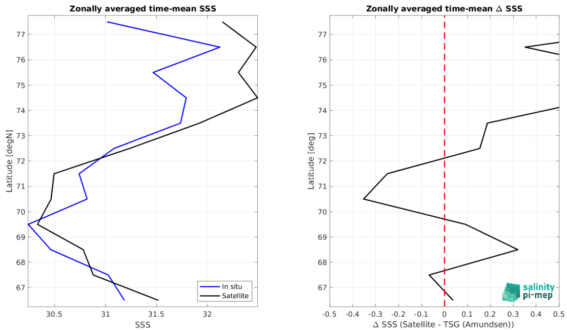
Figure 8: Left panel: Zonal mean SSS from Aquarius SSS L4 OI v5 - Monthly (IPRC) satellite product (black) and from TSG (Amundsen) (blue). Right panel: Zonal mean of \Delta SSS (Satellite - TSG (Amundsen)) for all the collected Pi-MEP match-up pairs estimated over the full satellite product period.
