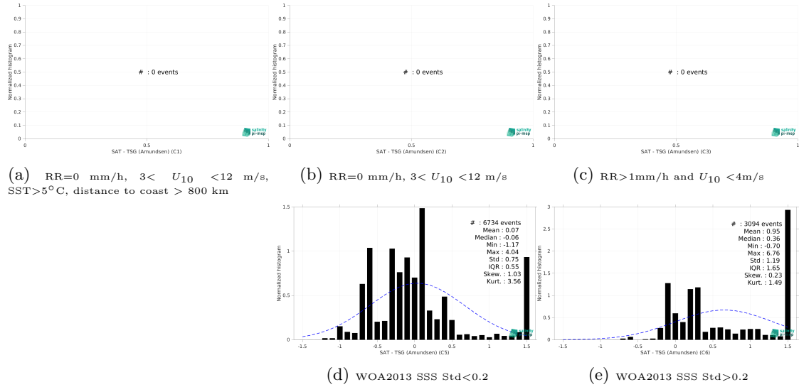
Figure 13: Normalized histogram of \Delta SSS (Aquarius SSS L4 OI v5 - Monthly (IPRC) - TSG (Amundsen)) for 5 different subdatasets corresponding to: RR=0 mm/h, 3 < U_{10} < 12 m/s, SST>5°C, distance to coast > 800 km (a), RR=0 mm/h, 3 < U_{10} < 12 m/s (b), RR>1mm/h and U_{10} < 4 m/s (c), WOA2013 SSS Std<0.2 (d), WOA2013 SSS Std>0.2 (e).
