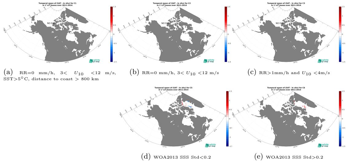
Figure 12: Temporal mean gridded over spatial boxes of size 1^{\circ}\times 1^{\circ} of \Delta\text{SSS} (Aquarius SSS L4 OI v5 - Monthly (IPRC) - TSG (Amundsen)) for 5 different subdatasets corresponding to:RR=0 mm/h, 3 < U_{10} < 12 m/s, SST > 5^{\circ}\text{C} , distance to coast > 800 km (a), RR=0 mm/h, 3 < U_{10} < 12 m/s (b), RR > 1 mm/h and U_{10} < 4 m/s (c), WOA2013 SSS Std < 0.2 (d), WOA2013 SSS Std > 0.2 (e).
