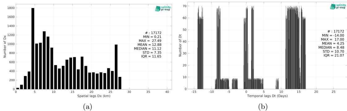
Figure 5: Histograms of the spatial (a) and temporal (b) lags between the location/time of the TSG (Amundsen) measurement and the date of the corresponding Aquarius SSS L4 OI v5 - Monthly (IPRC) SSS pixel.
