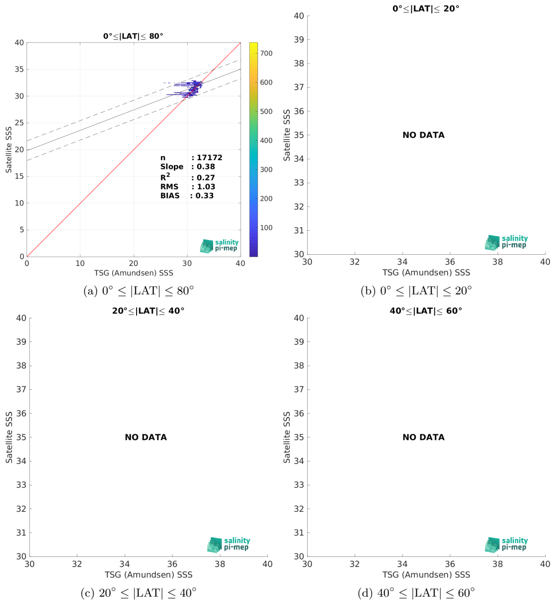
Figure 9: Contour maps of the concentration of Aquarius SSS L4 OI v5 - Monthly (IPRC) SSS (y-axis) versus TSG (Amundsen) SSS (x-axis) at match-up pairs for different latitude bands. For each plot, the red line shows x=y . The black thin and dashed lines indicate a linear fit through the data cloud and the \pm 95\% confidence levels, respectively. The number match-up pairs n , the slope and R^2 coefficient of the linear fit, the root mean square (RMS) and the mean bias between satellite and in situ data are indicated for each latitude band in each plots.
