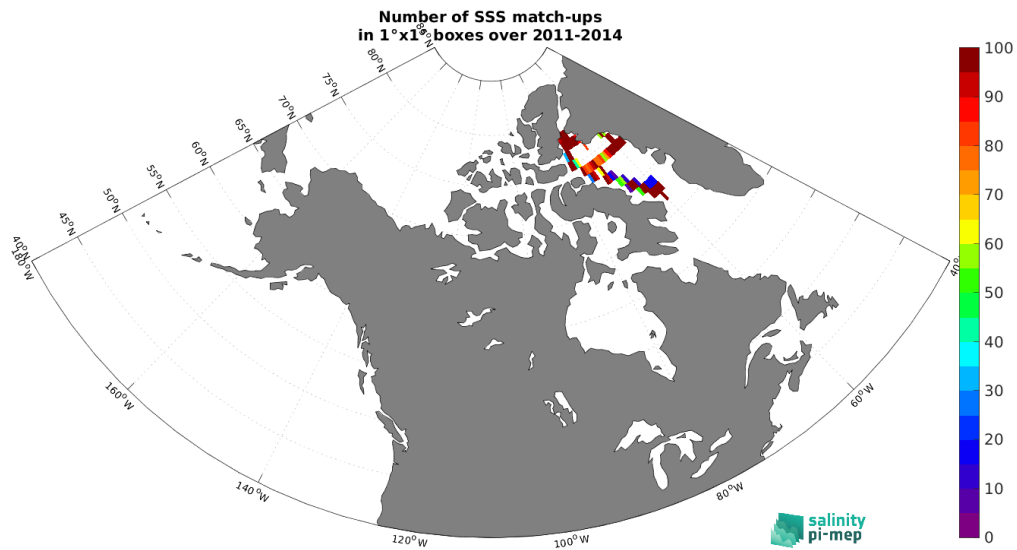
Figure 4: Number of SSS match-ups between TSG (Amundsen) SSS and the Aquarius SSS L4 OI v5 - Monthly (IPRC) SSS product for the Arctic Ocean Pi-MEP region over 1°x1° boxes and for the full satellite product period.
