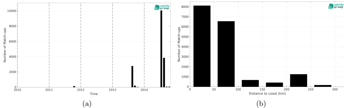
Figure 1: Number of match-ups between TSG (Amundsen) and Aquarius SSS L4 OI v5 - Monthly (IPRC) SSS as a function of time (a) and as function of the distance to coast (b) over the Arctic Ocean Pi-MEP region and for the full satellite product period.
