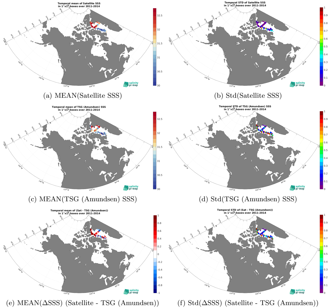
Figure 6: Temporal mean (left) and Std (right) of SSS from Aquarius SSS L4 OI v5 - Monthly (IPRC) (top), TSG (Amundsen) (middle), and of \Delta SSS (Satellite - TSG (Amundsen)). Only match-up pairs are used to generate these maps.
