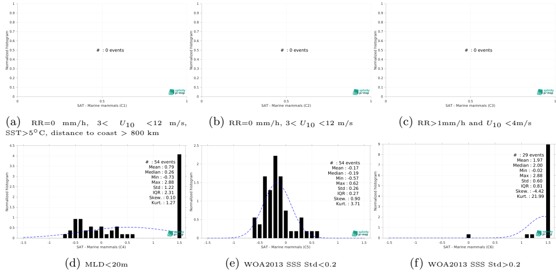
Figure 13: Normalized histogram of \Delta\text{SSS} (Aquarius SSS L4 OI v5 - Monthly (IPRC) - Marine mammals) for 6 different subdatasets corresponding to: RR=0 mm/h, 3 < U_{10} < 12 m/s, SST > 5^\circ\text{C} , distance to coast > 800 km (a), RR=0 mm/h, 3 < U_{10} < 12 m/s (b), RR > 1\text{mm/h} and U_{10} < 4\text{m/s} (c), MLD < 20\text{m} (d), WOA2013 SSS Std < 0.2 (e), WOA2013 SSS Std > 0.2 (f).
