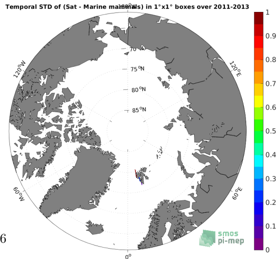
(f) Std( \Delta SSS) (Satellite - Marine mammals)
