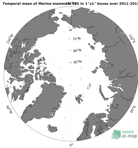
(c) MEAN(Marine mammals SSS)
