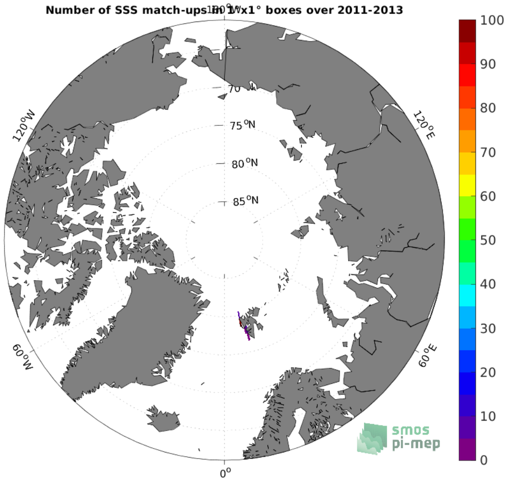
Figure 4: Number of SSS match-ups between Marine mammals SSS and the Aquarius SSS L4 OI v5 - Monthly (IPRC) SSS product for the Arctic Ocean Pi-MEP region over 1^\circ \times 1^\circ boxes and for the full satellite product period.
