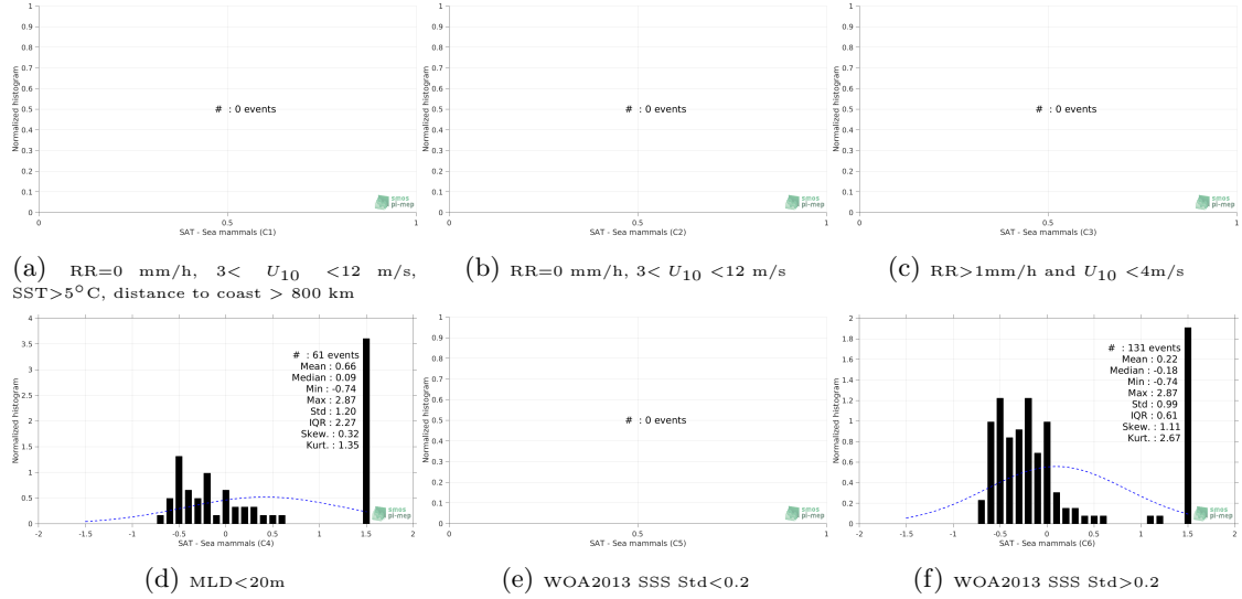
Figure 13: Normalized histogram of \Delta\text{SSS} (Aquarius-L4-IPRC-V5-MONTHLY - Sea mammals) for 6 different subdatasets corresponding to: RR=0 mm/h, 3 < U_{10} < 12 m/s, SST > 5^{\circ}\text{C} , distance to coast > 800 km (a), RR=0 mm/h, 3 < U_{10} < 12 m/s (b), RR > 1\text{mm/h} and U_{10} < 4\text{m/s} (c), MLD < 20\text{m} (d), WOA2013 SSS Std < 0.2 (e), WOA2013 SSS Std > 0.2 (f).
