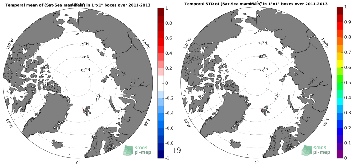
(e) MEAN( \Delta SSS) (Satellite - Sea mammals)
