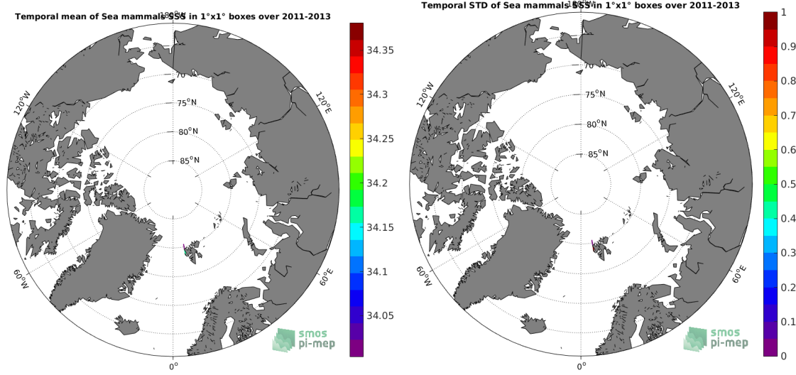
(c) MEAN(Sea mammals SSS)
