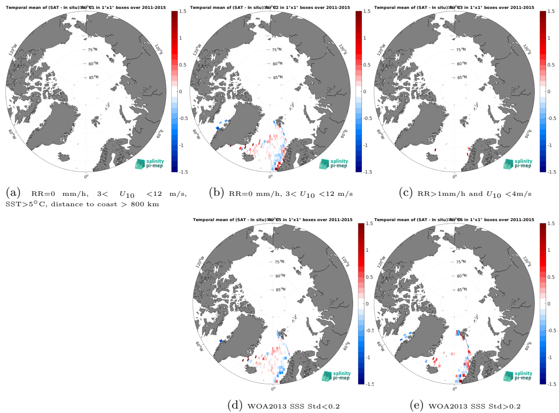
Figure 14: Temporal mean gridded over spatial boxes of size 1^\circ \times 1^\circ of \Delta SSS (Aquarius SSS L4 OI v5 - Monthly (IPRC) - ICES) for 5 different subdatasets corresponding to:RR=0 mm/h, 3 < U_{10} < 12 m/s, SST > 5^\circ\text{C} , distance to coast > 800 km (a), RR=0 mm/h, 3 < U_{10} < 12 m/s (b), RR > 1 mm/h and U_{10} < 4 m/s (c), WOA2013 SSS Std < 0.2 (d), WOA2013 SSS Std > 0.2 (e).
