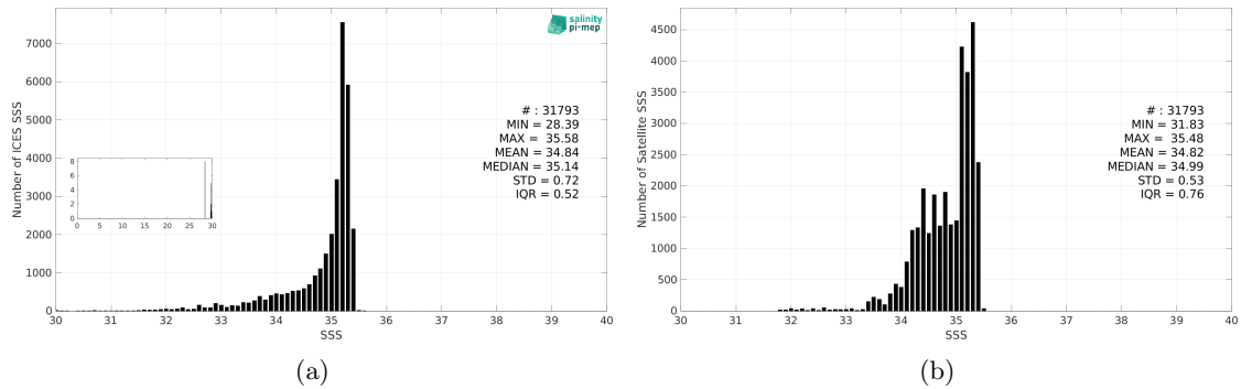
Figure 3: Histograms of SSS from ICES (a) and Aquarius SSS L4 OI v5 - Monthly (IPRC) (b) considering all match-up pairs per bins of 0.1 over the Arctic Ocean Pi-MEP region and for the full satellite product period.
