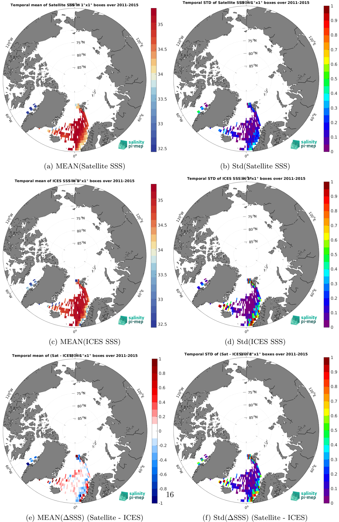
Figure 7: Temporal mean (left) and Std (right) of SSS from Aquarius SSS L4 OI v5 - Monthly (IPRC) (top), ICES (middle), and of \Delta SSS (Satellite - ICES). Only match-up pairs are used to generate these maps.
