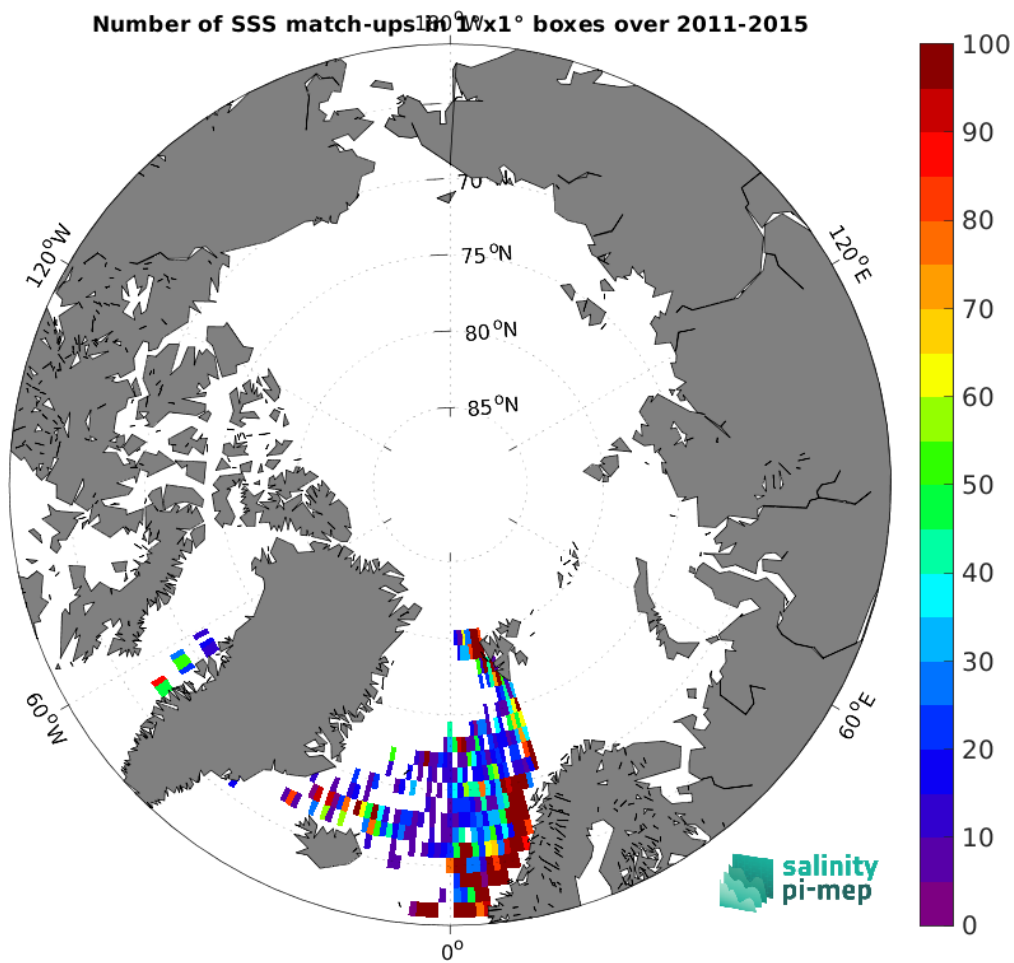
Figure 5: Number of SSS match-ups between ICES SSS and the Aquarius SSS L4 OI v5 - Monthly (IPRC) SSS product for the Arctic Ocean Pi-MEP region over 1^\circ \times 1^\circ boxes and for the full satellite product period.
