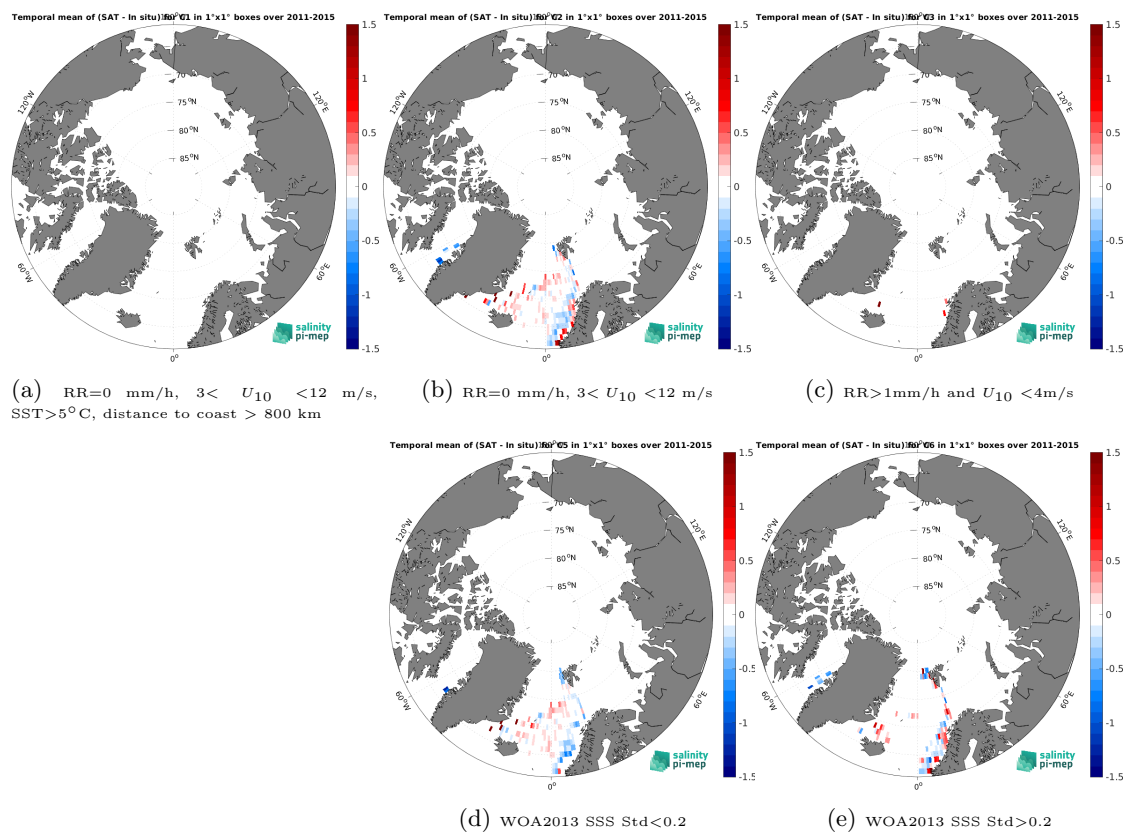
Figure 14: Temporal mean gridded over spatial boxes of size 1^\circ \times 1^\circ of \Delta\text{SSS} (Aquarius SSS L4 OI v5 - Monthly (IPRC) - ICES) for 5 different subdatasets corresponding to: RR=0 mm/h, 3 < U_{10} < 12 m/s, SST > 5°C, distance to coast > 800 km (a), RR=0 mm/h, 3 < U_{10} < 12 m/s (b), RR > 1mm/h and U_{10} < 4 m/s (c), WOA2013 SSS Std < 0.2 (d), WOA2013 SSS Std > 0.2 (e).
