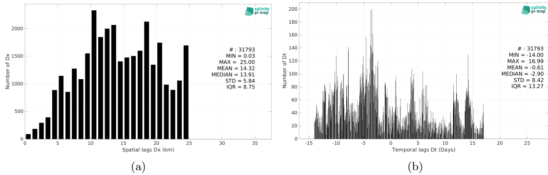
Figure 6: Histograms of the spatial (a) and temporal (b) lags between the location/time of the ICES measurement and the date of the corresponding Aquarius SSS L4 OI v5 - Monthly (IPRC) SSS pixel.
