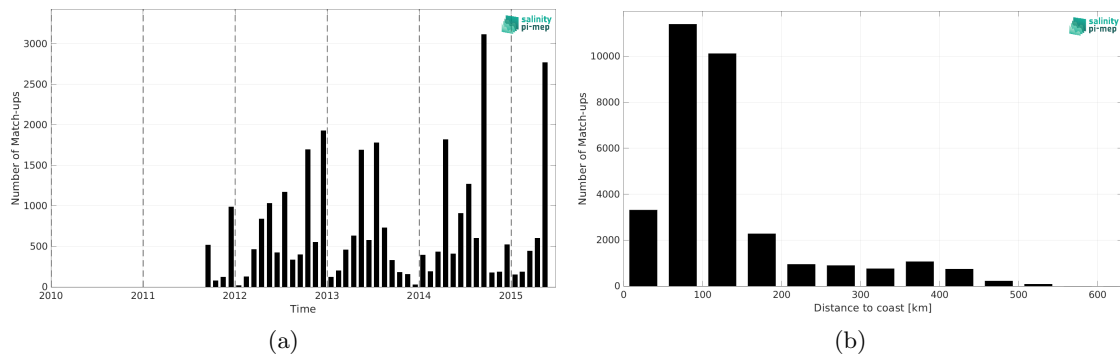
Figure 2: Number of match-ups between ICES and Aquarius SSS L4 OI v5 - Monthly (IPRC) SSS as a function of time (a) and as function of the distance to coast (b) over the Arctic Ocean Pi-MEP region and for the full satellite product period.
