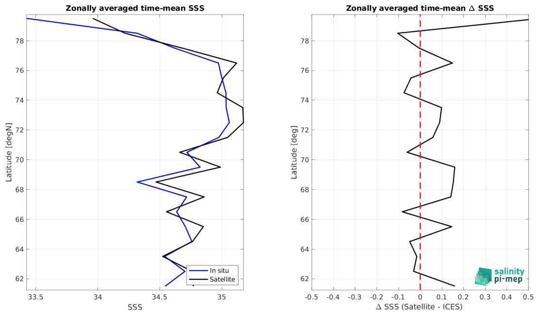
Figure 9: Left panel: Zonal mean SSS from Aquarius SSS L4 OI v5 - Monthly (IPRC) satellite product (black) and from ICES (blue). Right panel: Zonal mean of \Delta SSS (Satellite - ICES) for all the collected Pi-MEP match-up pairs estimated over the full satellite product period.
