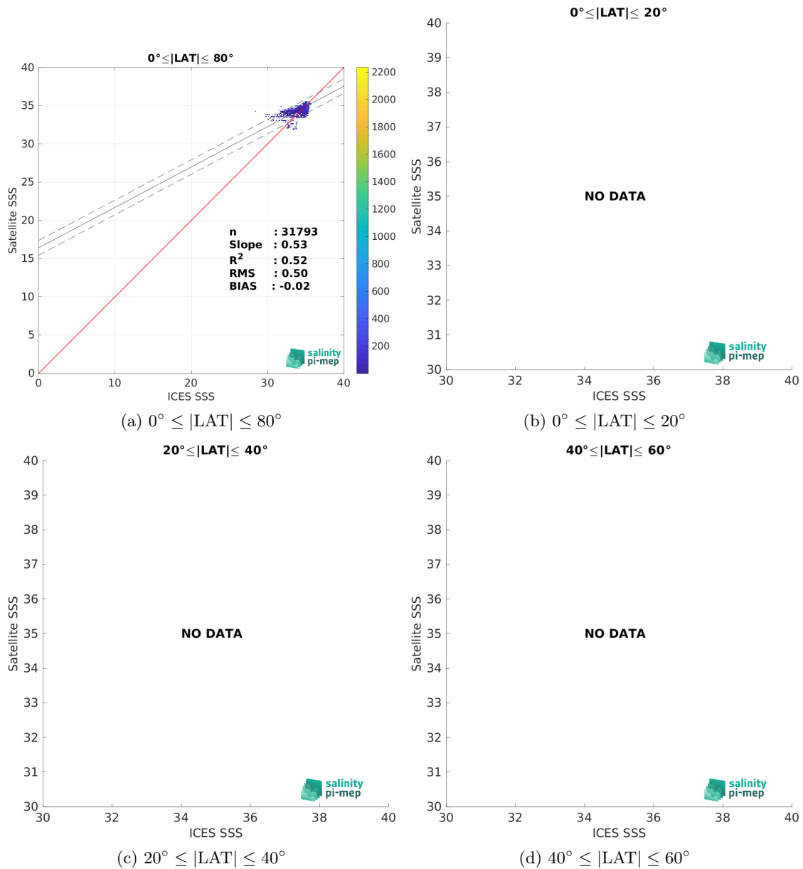
Figure 10: Contour maps of the concentration of Aquarius SSS L4 OI v5 - Monthly (IPRC) SSS (y-axis) versus ICES SSS (x-axis) at match-up pairs for different latitude bands. For each plot, the red line shows x=y . The black thin and dashed lines indicate a linear fit through the data cloud and the \pm 95\% confidence levels, respectively. The number match-up pairs n , the slope and R^2 coefficient of the linear fit, the root mean square (RMS) and the mean bias between satellite and in situ data are indicated for each latitude band in each plots.
