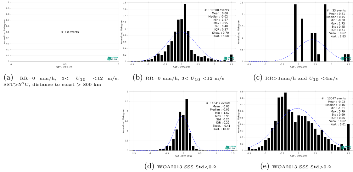
Figure 15: Normalized histogram of \Delta SSS (Aquarius SSS L4 OI v5 - Monthly (IPRC) - ICES) for 5 different subdatasets corresponding to: RR=0 mm/h, 3 < U_{10} < 12 m/s, SST > 5°C, distance to coast > 800 km (a), RR=0 mm/h, 3 < U_{10} < 12 m/s (b), RR > 1mm/h and U_{10} < 4 m/s (c), WOA2013 SSS Std < 0.2 (d), WOA2013 SSS Std > 0.2 (e).
