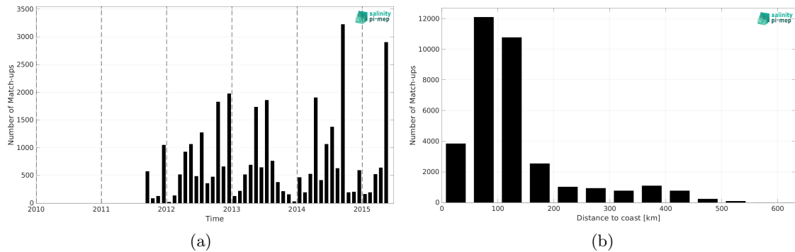
Figure 1: Number of match-ups between ICES and Aquarius SSS L4 OI v5 - Monthly (IPRC) SSS as a function of time (a) and as function of the distance to coast (b) over the Arctic Ocean Pi-MEP region and for the full satellite product period.
