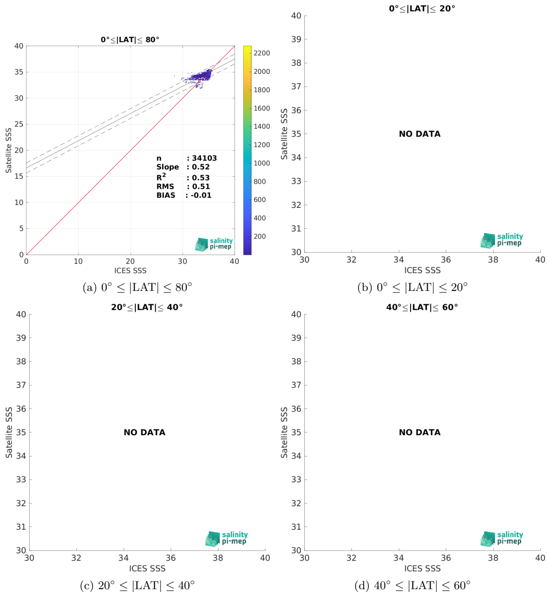
Figure 9: Contour maps of the concentration of Aquarius SSS L4 OI v5 - Monthly (IPRC) SSS (y-axis) versus ICES SSS (x-axis) at match-up pairs for different latitude bands. For each plot, the red line shows x=y . The black thin and dashed lines indicate a linear fit through the data cloud and the \pm 95\% confidence levels, respectively. The number match-up pairs n , the slope and R^2 coefficient of the linear fit, the root mean square (RMS) and the mean bias between satellite and in situ data are indicated for each latitude band in each plots.
