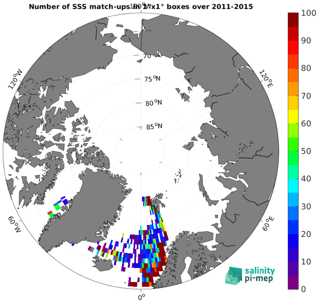
Figure 4: Number of SSS match-ups between ICES SSS and the Aquarius SSS L4 OI v5 - Monthly (IPRC) SSS product for the Arctic Ocean Pi-MEP region over 1^\circ \times 1^\circ boxes and for the full satellite product period.
