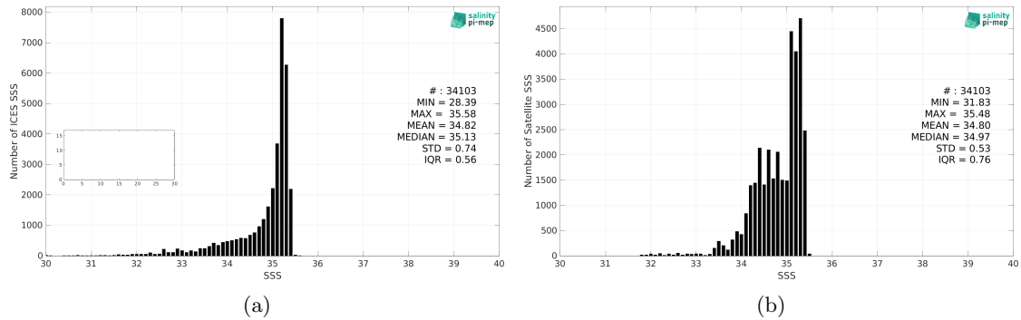
Figure 2: Histograms of SSS from ICES (a) and Aquarius SSS L4 OI v5 - Monthly (IPRC) (b) considering all match-up pairs per bins of 0.1 over the Arctic Ocean Pi-MEP region and for the full satellite product period.
