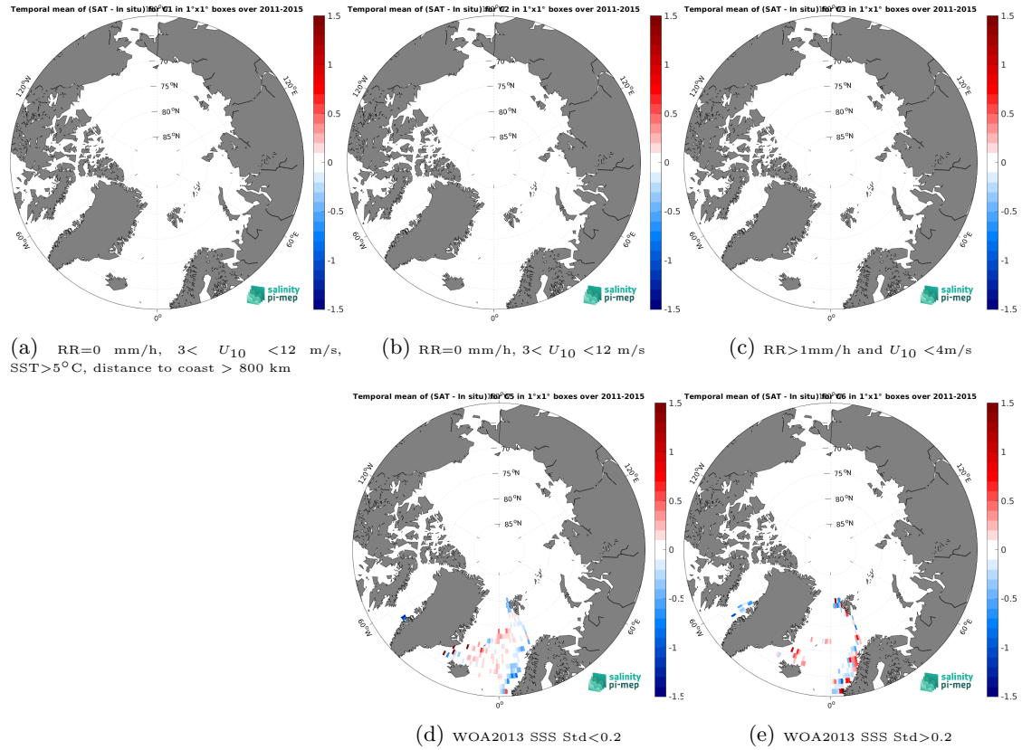
Figure 12: Temporal mean gridded over spatial boxes of size 1^{\circ}\times 1^{\circ} of \Delta\text{SSS} (Aquarius SSS L4 OI v5 - Monthly (IPRC) - ICES) for 5 different subdatasets corresponding to:RR=0 mm/h, 3 < U_{10} < 12 m/s, SST > 5^{\circ}\text{C} , distance to coast > 800 km (a), RR=0 mm/h, 3 < U_{10} < 12 m/s (b), RR > 1 mm/h and U_{10} < 4 m/s (c), WOA2013 SSS Std < 0.2 (d), WOA2013 SSS Std > 0.2 (e).
