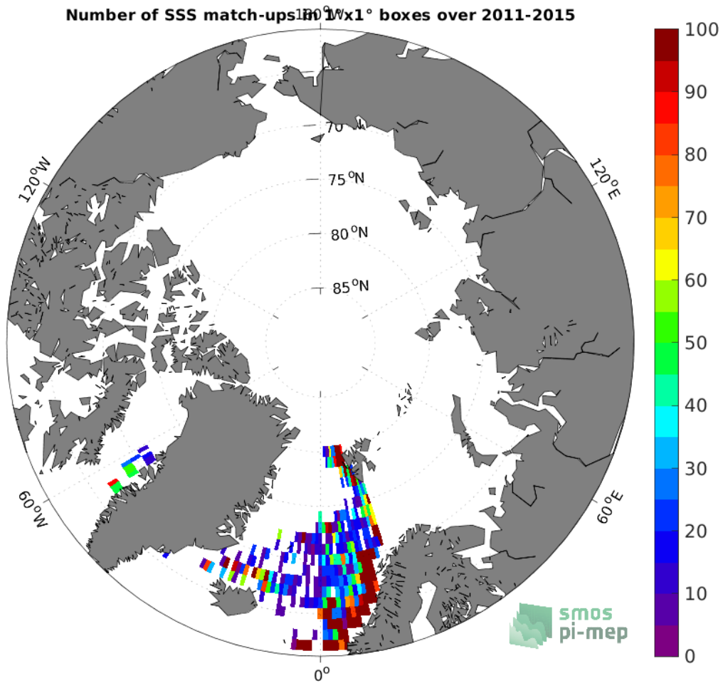
Figure 4: Number of SSS match-ups between ICES SSS and the Aquarius SSS L4 OI v5 - Monthly (IPRC) SSS product for the Arctic Ocean Pi-MEP region over 1^{\circ} \times 1^{\circ} boxes and for the full satellite product period.
