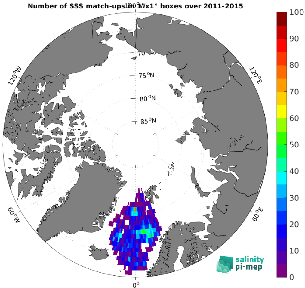
Figure 5: Number of SSS match-ups between Argo SSS and the Aquarius SSS L4 OI v5 - Monthly (IPRC) SSS product for the Arctic Ocean Pi-MEP region over 1^\circ \times 1^\circ boxes and for the full satellite product period.
