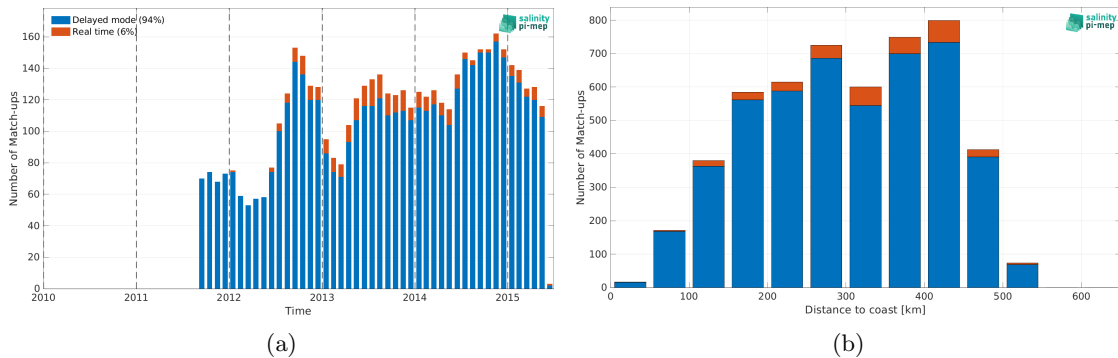
Figure 2: Number of match-ups between Argo and Aquarius SSS L4 OI v5 - Monthly (IPRC) SSS as a function of time (a) and as function of the distance to coast (b) over the Arctic Ocean Pi-MEP region and for the full satellite product period.
