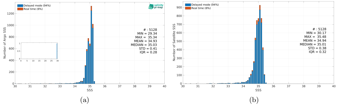
Figure 3: Histograms of SSS from Argo (a) and Aquarius SSS L4 OI v5 - Monthly (IPRC) (b) considering all match-up pairs per bins of 0.1 over the Arctic Ocean Pi-MEP region and for the full satellite product period.
