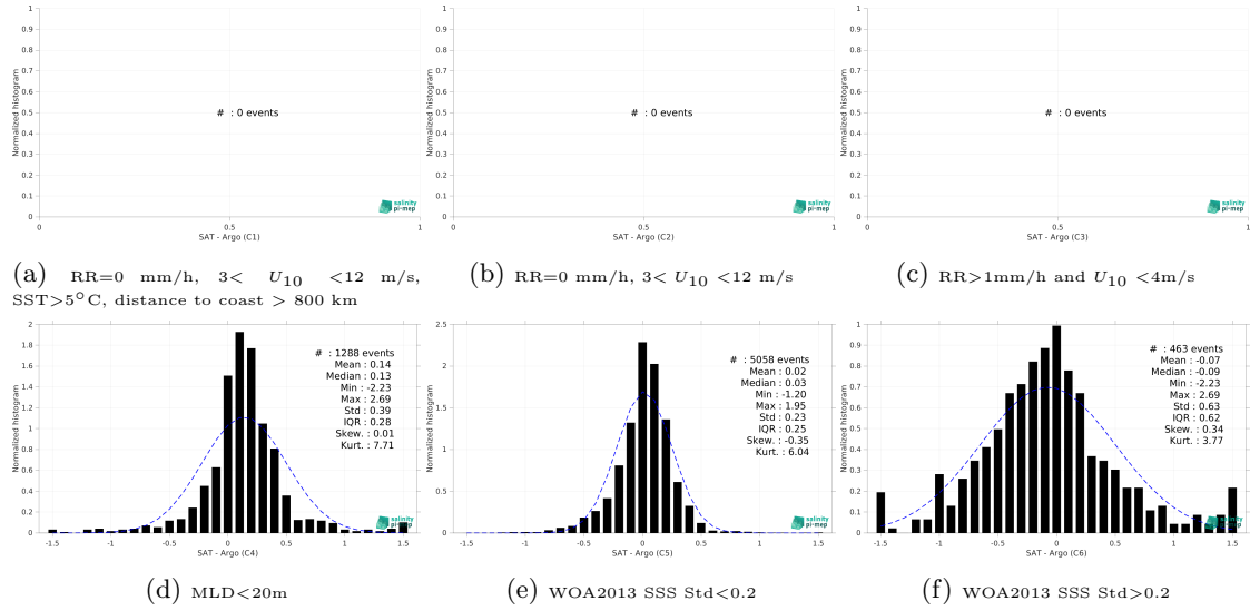
Figure 13: Normalized histogram of \Delta\text{SSS} (Aquarius SSS L4 OI v5 - Monthly (IPRC) - Argo) for 6 different subdatasets corresponding to: RR=0 mm/h, 3 < U_{10} < 12 m/s, SST > 5^\circ\text{C} , distance to coast > 800 km (a), RR=0 mm/h, 3 < U_{10} < 12 m/s (b), RR > 1\text{mm/h} and U_{10} < 4\text{m/s} (c), MLD < 20\text{m} (d), WOA2013 SSS Std < 0.2 (e), WOA2013 SSS Std > 0.2 (f).
