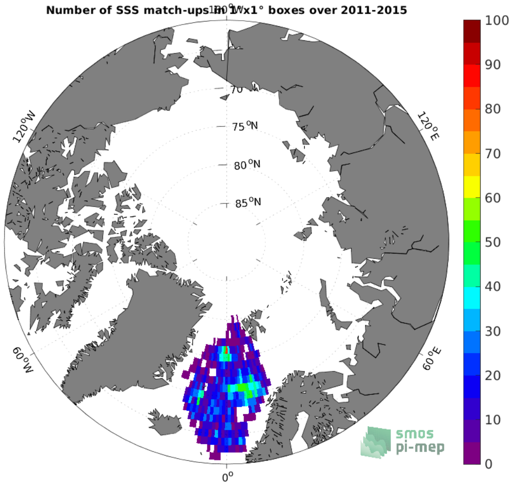
Figure 4: Number of SSS match-ups between Argo SSS and the Aquarius SSS L4 OI v5 - Monthly (IPRC) SSS product for the Arctic Ocean Pi-MEP region over 1^\circ \times 1^\circ boxes and for the full satellite product period.
