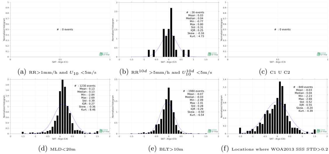
Figure 13: Normalized histogram of \Delta SSS (Aquarius-L4-IPRC-V5-MONTHLY - Argo) for 6 different subdatasets corresponding to: RR > 1mm/h and U_{10} < 5 m/s (a), RR^{10d} > 5 mm/h and U_{10}^{10d} < 5 m/s (b), C1 U C2 (c), MLD < 20m (d), BLT > 10m (e), Locations where WOA2013 SSS STD > 0.2 (f).
