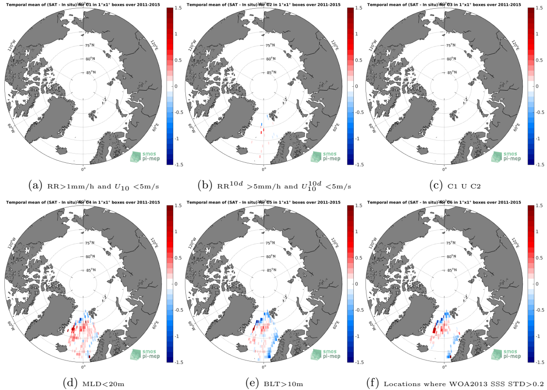
Figure 12: Temporal mean gridded over spatial boxes of size 1°x1° of \Delta SSS (Aquarius-L4-IPRC-V5-MONTHLY - Argo) for 6 different subdatasets corresponding to: RR > 1\text{mm/h} and U_{10} < 5\text{m/s} (a), RR^{10d} > 5\text{mm/h} and U_{10}^{10d} < 5\text{m/s} (b), C1 U C2 (c), MLD < 20\text{m} (d), BLT > 10\text{m} (e), Locations where WOA2013 SSS STD > 0.2 (f).
