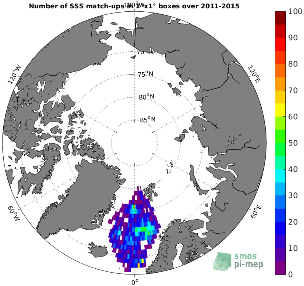
Figure 4: Number of SSS match-ups between Argo SSS and the Aquarius-L4-IPRC-V5-MONTHLY SSS product for the Arctic Ocean Pi-MEP region over 1^\circ \times 1^\circ boxes and for the full satellite product period.
