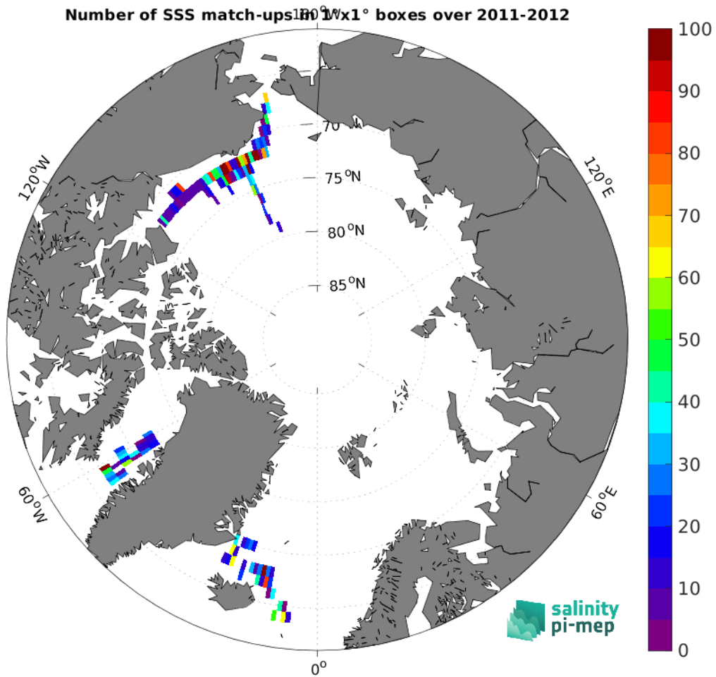
Figure 5: Number of SSS match-ups between TSG (SAMOS) SSS and the Aquarius SSS L3 OR v5 - 7-Day running (NASA-GSFC) SSS product for the Arctic Ocean Pi-MEP region over 1^\circ \times 1^\circ boxes and for the full satellite product period.
