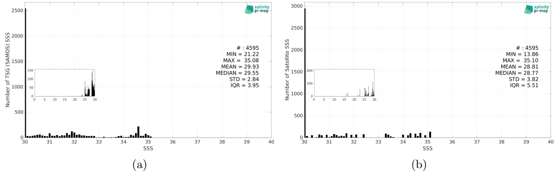
Figure 3: Histograms of SSS from TSG (SAMOS) (a) and Aquarius SSS L3 OR v5 - 7-Day running (NASA-GSFC) (b) considering all match-up pairs per bins of 0.1 over the Arctic Ocean Pi-MEP region and for the full satellite product period.
