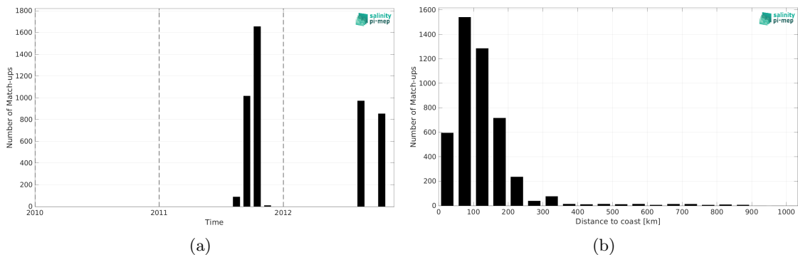
Figure 2: Number of match-ups between TSG (SAMOS) and Aquarius SSS L3 OR v5 - 7-Day running (NASA-GSFC) SSS as a function of time (a) and as function of the distance to coast (b) over the Arctic Ocean Pi-MEP region and for the full satellite product period.
