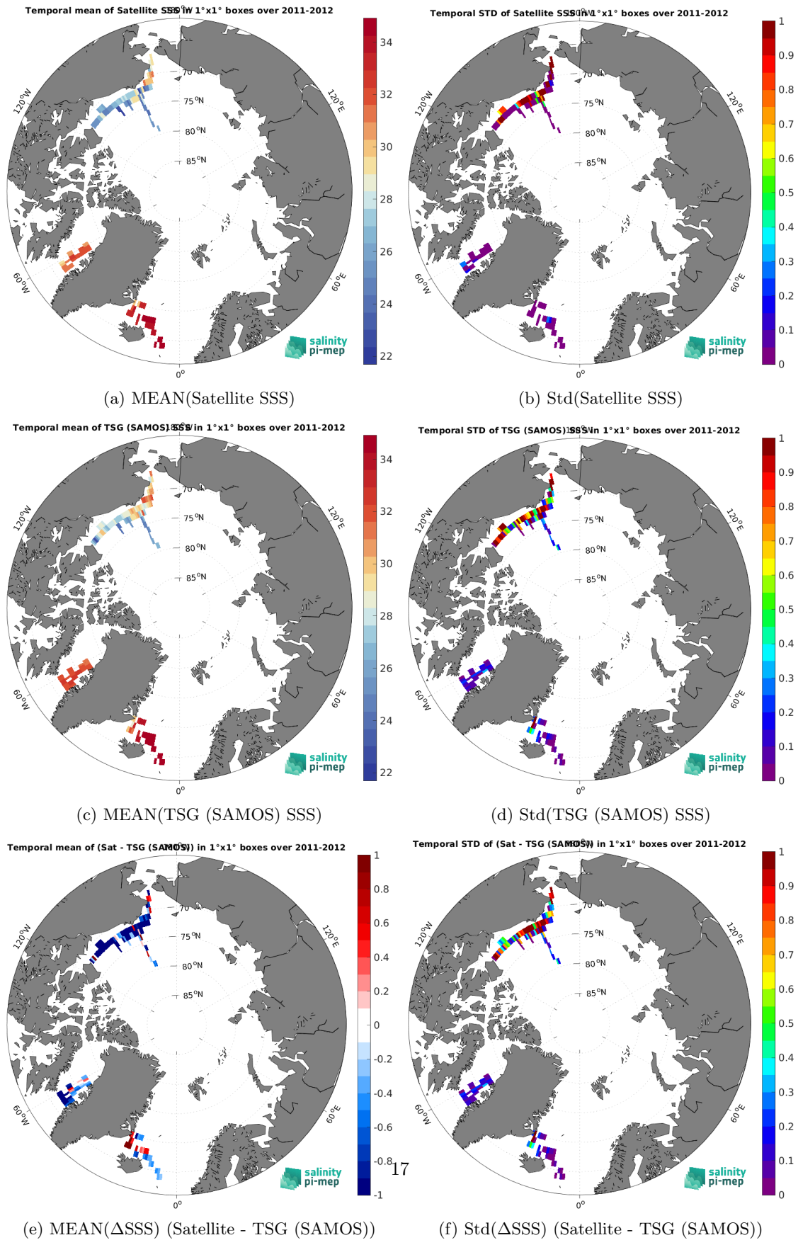
Figure 7: Temporal mean (left) and Std (right) of SSS from Aquarius SSS L3 OR v5 - 7-Day running (NASA-GSFC) (top), TSG (SAMOS) (middle), and of \Delta SSS (Satellite - TSG (SAMOS)). Only match-up pairs are used to generate these maps.
