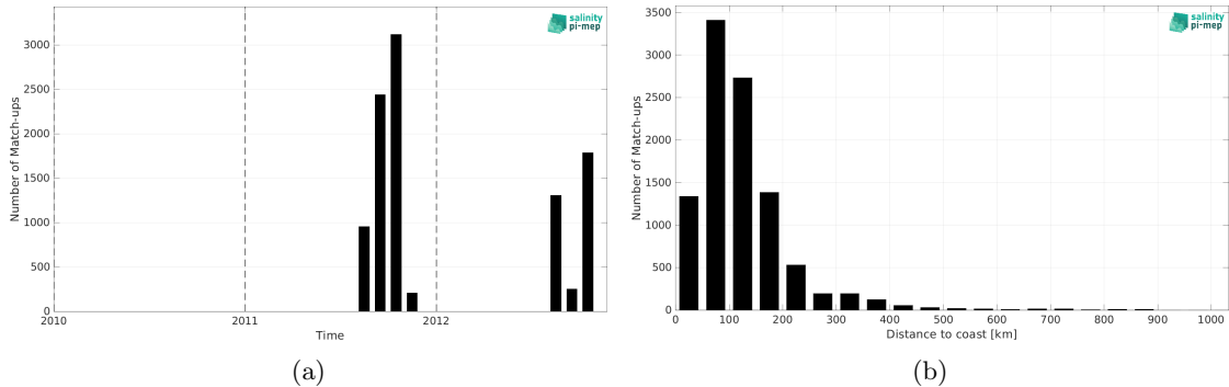
Figure 1: Number of match-ups between TSG (SAMOS) and Aquarius SSS L3 OR v5 - 7-Day running (NASA-GSFC) SSS as a function of time (a) and as function of the distance to coast (b) over the Arctic Ocean Pi-MEP region and for the full satellite product period.
