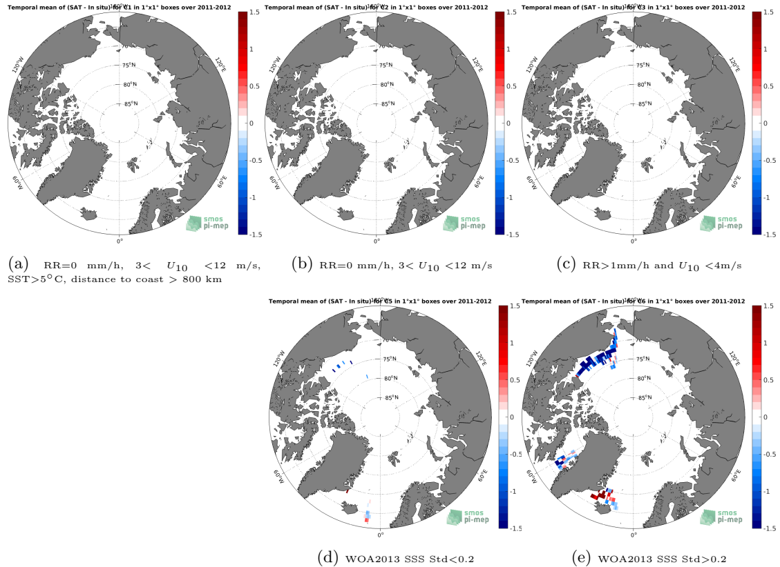
Figure 12: Temporal mean gridded over spatial boxes of size 1^{\circ}\times 1^{\circ} of \Delta\text{SSS} (Aquarius SSS L3 OR v5 - 7-Day running (NASA-GSFC) - TSG (SAMOS)) for 5 different subdatasets corresponding to: RR=0 mm/h, 3 < U_{10} < 12 m/s, SST > 5^{\circ}\text{C} , distance to coast > 800 km (a), RR=0 mm/h, 3 < U_{10} < 12 m/s (b), RR > 1 mm/h and U_{10} < 4 m/s (c), WOA2013 SSS Std < 0.2 (d), WOA2013 SSS Std > 0.2 (e).
