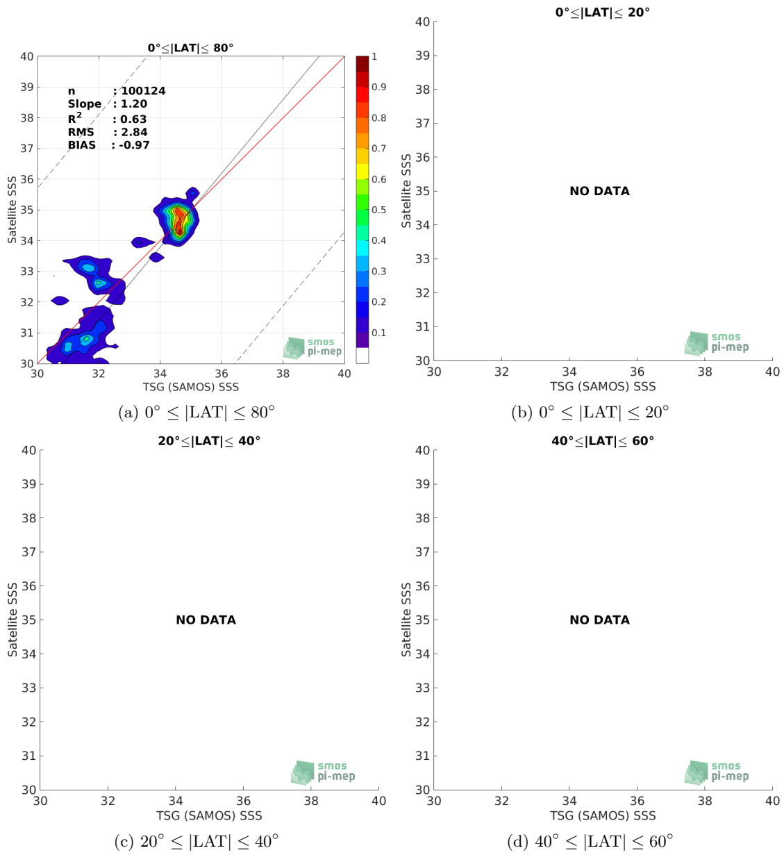
Figure 9: Contour maps of the concentration of Aquarius SSS L3 OR v5 - 7-Day running (NASA-GSFC) SSS (y-axis) versus TSG (SAMOS) SSS (x-axis) at match-up pairs for different latitude bands. For each plot, the red line shows x=y . The black thin and dashed lines indicate a linear fit through the data cloud and the \pm 95\% confidence levels, respectively. The number match-up pairs n , the slope and R^2 coefficient of the linear fit, the root mean square (RMS) and the mean bias between satellite and in situ data are indicated for each latitude band in each plots.
