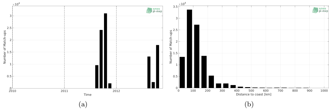
Figure 1: Number of match-ups between TSG (SAMOS) and Aquarius SSS L3 OR v5 - 7-Day running (NASA-GSFC) SSS as a function of time (a) and as function of the distance to coast (b) over the Arctic Ocean Pi-MEP region and for the full satellite product period.
