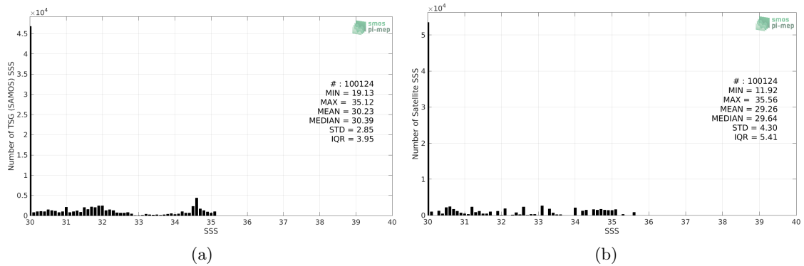
Figure 2: Histograms of SSS from TSG (SAMOS) (a) and Aquarius SSS L3 OR v5 - 7-Day running (NASA-GSFC) (b) considering all match-up pairs per bins of 0.1 over the Arctic Ocean Pi-MEP region and for the full satellite product period.
