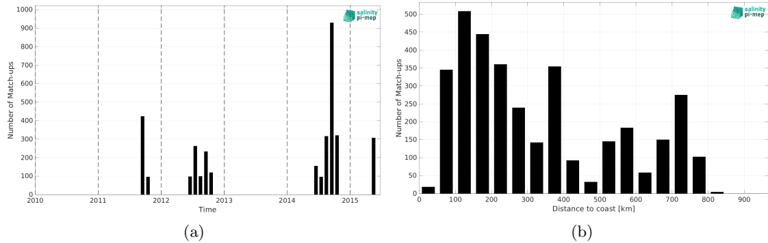
Figure 2: Number of match-ups between TSG (Polarstern) and Aquarius SSS L3 OR v5 - 7-Day running (NASA-GSFC) SSS as a function of time (a) and as function of the distance to coast (b) over the Arctic Ocean Pi-MEP region and for the full satellite product period.
