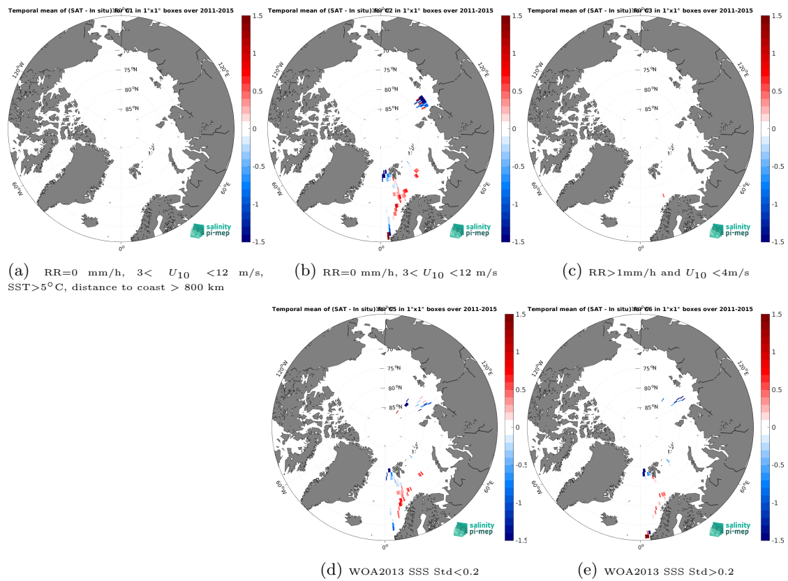
Figure 14: Temporal mean gridded over spatial boxes of size 1^\circ \times 1^\circ of \Delta SSS (Aquarius SSS L3 OR v5 - 7-Day running (NASA-GSFC) - TSG (Polarstern)) for 5 different subdatasets corresponding to:RR=0 mm/h, 3 < U_{10} < 12 m/s, SST >5^\circ C, distance to coast > 800 km (a), RR=0 mm/h, 3 < U_{10} < 12 m/s (b), RR >1 mm/h and U_{10} < 4 m/s (c), WOA2013 SSS Std <0.2 (d), WOA2013 SSS Std >0.2 (e).
