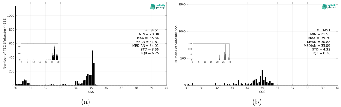
Figure 3: Histograms of SSS from TSG (Polarstern) (a) and Aquarius SSS L3 OR v5 - 7-Day running (NASA-GSFC) (b) considering all match-up pairs per bins of 0.1 over the Arctic Ocean Pi-MEP region and for the full satellite product period.
