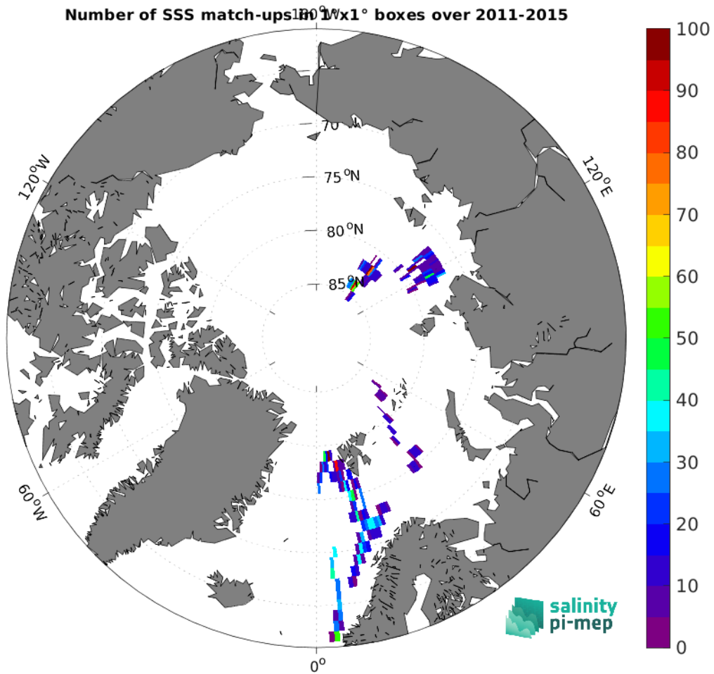
Figure 5: Number of SSS match-ups between TSG (Polarstern) SSS and the Aquarius SSS L3 OR v5 - 7-Day running (NASA-GSFC) SSS product for the Arctic Ocean Pi-MEP region over 1^{\circ} \times 1^{\circ} boxes and for the full satellite product period.
