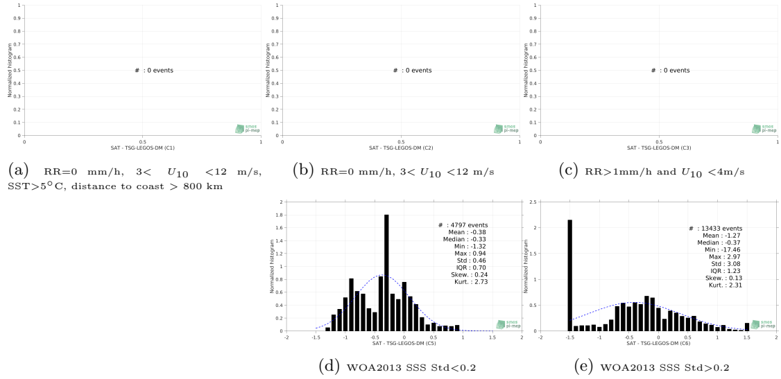
Figure 13: Normalized histogram of \Delta SSS (Aquarius-L3-OR-V5-7DAY-RUNNING-1DEG - TSG-LEGOS-DM) for 5 different subdatasets corresponding to: RR=0 mm/h, 3 < U_{10} < 12 m/s, SST>5°C, distance to coast > 800 km (a), RR=0 mm/h, 3 < U_{10} < 12 m/s (b), RR>1mm/h and U_{10} < 4 m/s (c), WOA2013 SSS Std<0.2 (d), WOA2013 SSS Std>0.2 (e).
