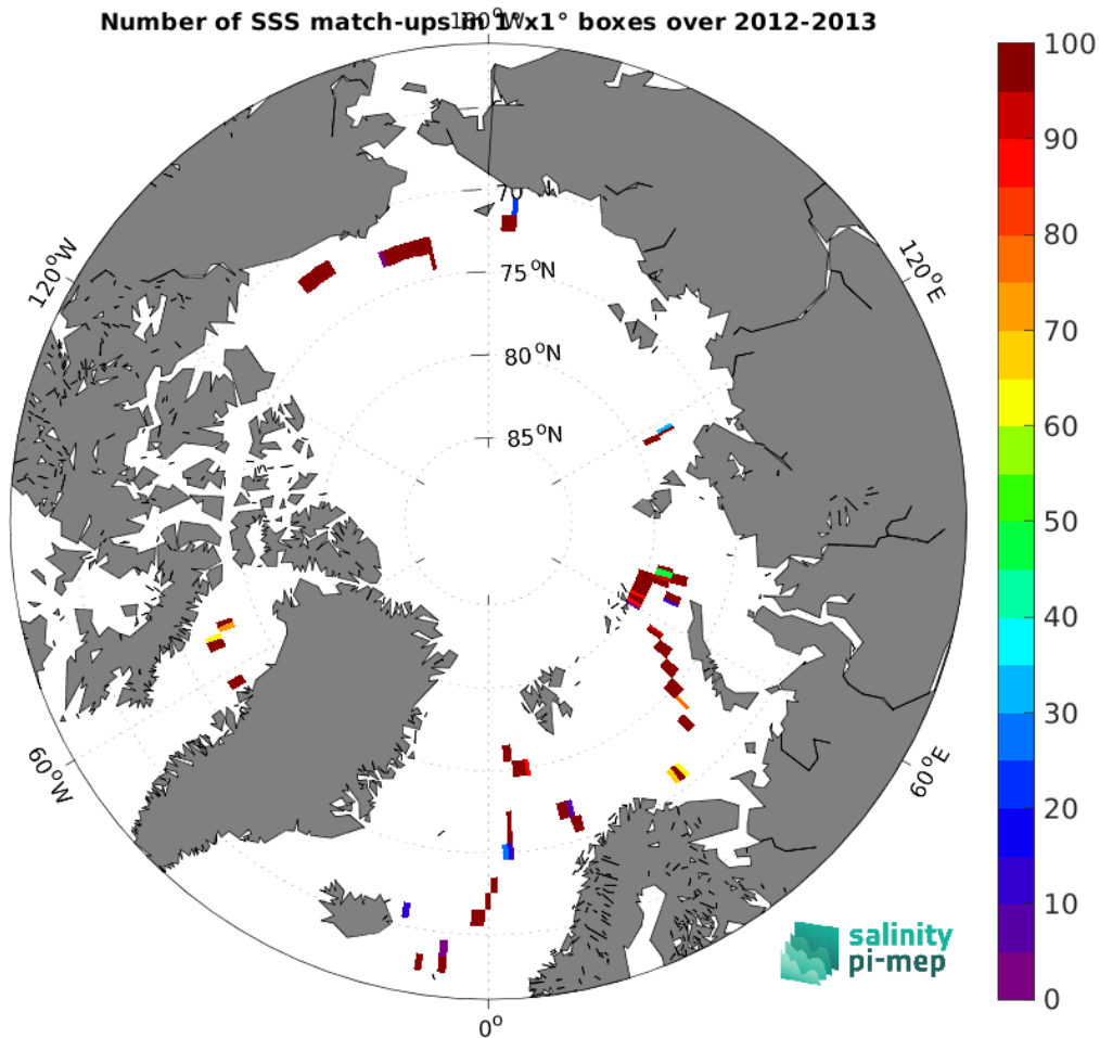
Figure 5: Number of SSS match-ups between TSG (GOSUD-Sailing-ship) SSS and the Aquarius SSS L3 OR v5 - 7-Day running (NASA-GSFC) SSS product for the Arctic Ocean Pi-MEP region over 1^\circ \times 1^\circ boxes and for the full satellite product period.
