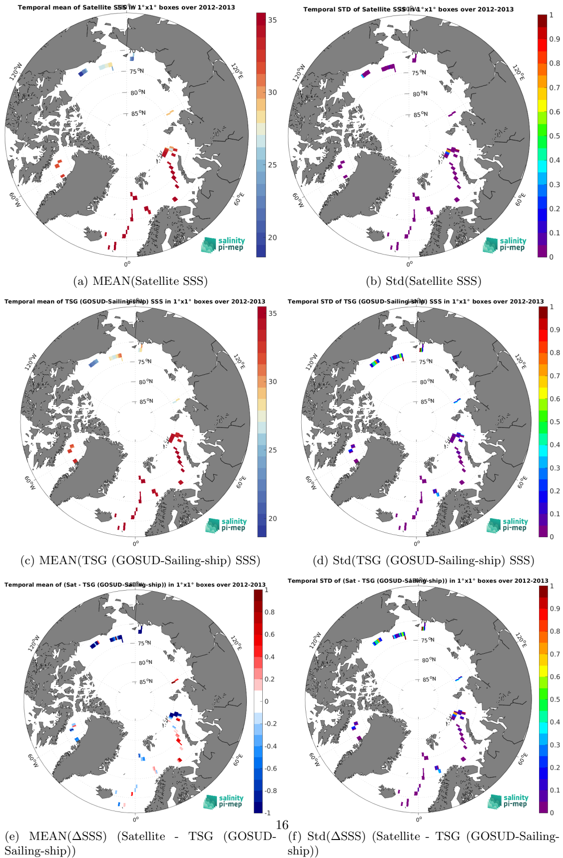
Figure 7: Temporal mean (left) and Std (right) of SSS from Aquarius SSS L3 OR v5 - 7-Day running (NASA-GSFC) (top), TSG (GOSUD-Sailing-ship) (middle), and of \Delta SSS (Satellite - TSG (GOSUD-Sailing-ship)). Only match-up pairs are used to generate these maps.
