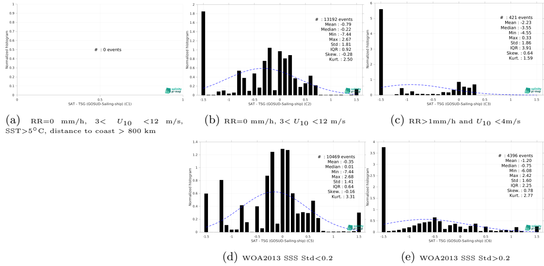
Figure 15: Normalized histogram of \Delta\text{SSS} (Aquarius SSS L3 OR v5 - 7-Day running (NASA-GSFC) - TSG (GOSUD-Sailing-ship)) for 5 different subdatasets corresponding to: RR=0 mm/h, 3 < U_{10} < 12 m/s, SST > 5^\circ\text{C} , distance to coast > 800 km (a), RR=0 mm/h, 3 < U_{10} < 12 m/s (b), RR > 1\text{mm/h} and U_{10} < 4\text{m/s} (c), WOA2013 SSS Std < 0.2 (d), WOA2013 SSS Std > 0.2 (e).
