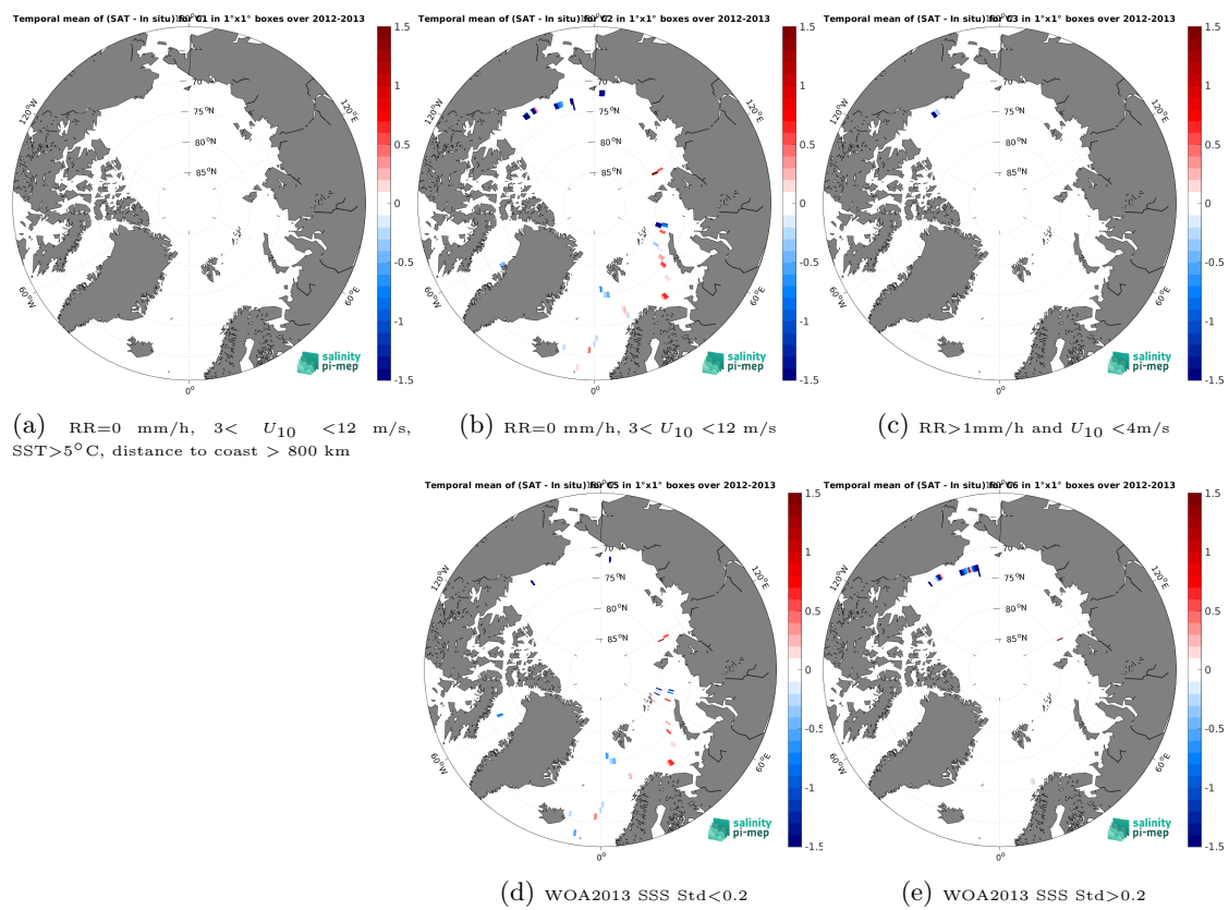
Figure 14: Temporal mean gridded over spatial boxes of size 1^\circ \times 1^\circ of \Delta SSS (Aquarius SSS L3 OR v5 - 7-Day running (NASA-GSFC) - TSG (GOSUD-Sailing-ship)) for 5 different subdatasets corresponding to:RR=0 mm/h, 3 < U_{10} < 12 m/s, SST >5^\circ\text{C} , distance to coast > 800 km (a), RR=0 mm/h, 3 < U_{10} < 12 m/s (b), RR >1 mm/h and U_{10} < 4 m/s (c), WOA2013 SSS Std <0.2 (d), WOA2013 SSS Std >0.2 (e).
