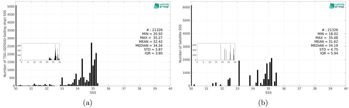
Figure 3: Histograms of SSS from TSG (GOSUD-Sailing-ship) (a) and Aquarius SSS L3 OR v5 - 7-Day running (NASA-GSFC) (b) considering all match-up pairs per bins of 0.1 over the Arctic Ocean Pi-MEP region and for the full satellite product period.
